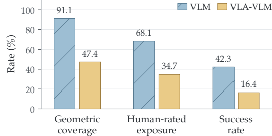
Figure 6: Anomaly exposure and success.
