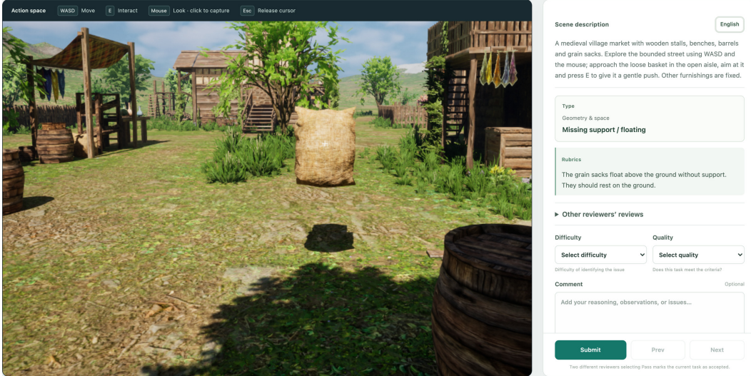
Figure 7: Human validation interface. Reviewers inspect the environment alongside its scene description, anomaly category, and evaluation rubric, then record quality, difficulty, and comments.
