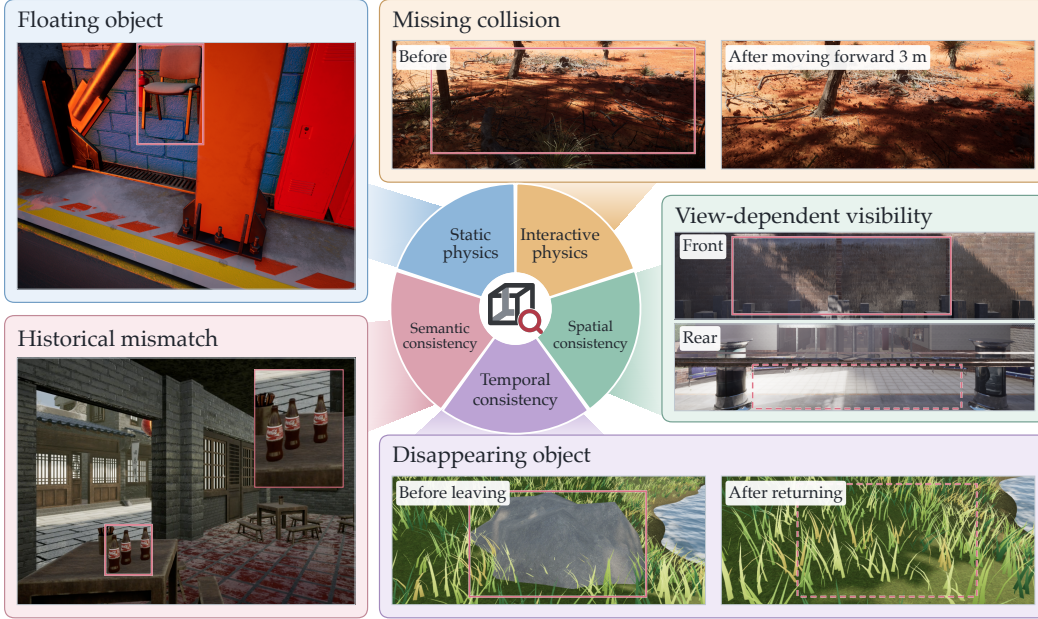
Figure 1: Anomaly taxonomy of WorldAuditBench (Section 3.2). Representative cases illustrate five families of physical, spatial, temporal, and semantic inconsistencies.
