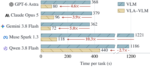
Figure 4: Auditing time per task.
