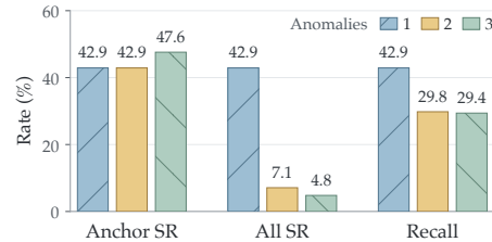
Figure 5: Auditing multiple anomalies.
