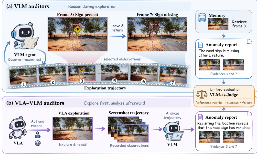
Figure 3: Two auditing paradigms. (a) VLM agents reason and use tools during exploration. (b) VLA-VLM auditors analyze trajectories after VLA exploration. Both use the same judge.
