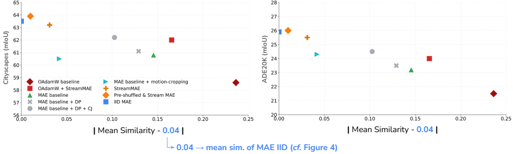
Figure 8: Downstream performance versus the distance from standard i.i.d. MAE in mean gradient cosine similarity between consecutive batches throughout training. Extending Figure 4, we include MAE trained on pre-shuffled & streaming WT++12h (Table 12), StreamMAE with Orthogonal-AdamW, and streaming MAE using only motion-biased crop selection. All models use a ViT-S/16 backbone and are pretrained on WT++12h. All streaming variants use B = 512 without DataDrop.
