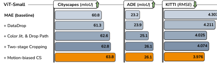
Figure 6: Cumulative ablation study with ViT-S/16 pretrained on WT++12h. Each row adds one component to the previous setting. DataDrop gives modest gains, while stronger regularization and crop selection account for most of the dense-transfer improvement. CS denotes crop selection.
