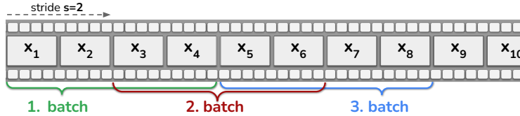
Figure 2: Streaming pretraining setup. Frames are observed in temporal order, and each batch is formed as a sliding window over the stream. Here: B = 4 and stride s = 2 , but typically s \ll B .
