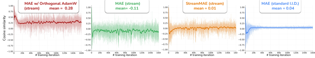
Figure 7: Running average of cosine similarity between gradients from consecutive batches, measured on last-block MLP parameters every 10 steps.
