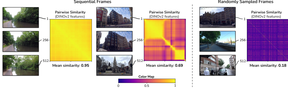
Figure 3: Pairwise DINOv2-L [37] feature similarities for 512 frames from WT++London show that consecutive frames at 15 FPS can be highly similar (left) or contain structured scene changes (block diagonal, middle), whereas randomly sampled frames are markedly more diverse (right).
