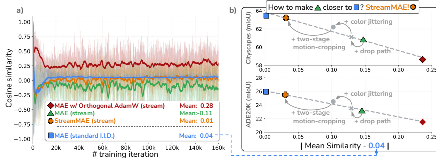
Figure 4: (a) Running average of consecutive batches gradient similarity, measured on last-block MLP parameters every 10 steps. (b) Dense downstream performance versus distance to standard i.i.d. MAE in mean gradient similarity. Methods closer to the i.i.d. MAE reference perform better.
