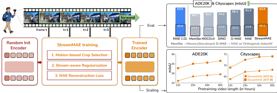
Figure 1: Left: StreamMAE adapts MAE to continuous video streams with stream-aware regularization and crop selection. Right: StreamMAE (ViT-S) improves dense performance over streaming SSL baselines (top) and improves with longer pretraining streams and a larger backbone (bottom).
