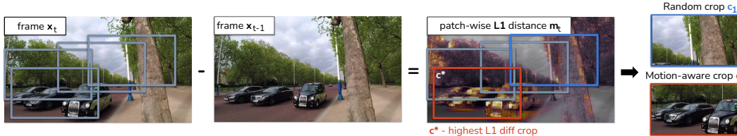
Figure 5: Motion-biased crop selection computes patch-level differences between consecutive frames x_t and x_{t-1} , samples K crop candidates \mathcal{C} , and selects the crop c_t^* with the largest average \ell_1 score.
