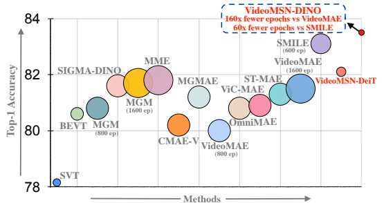
Figure 1: Comparison of top-1 accuracy on Kinetics-400 across state-of-the-art self-supervised video representation learning methods. Each point denotes a method, with bubble size proportional to its pretraining epochs. Our method, VideoMSN with DINO-v3 backbone, achieves state-of-the-art performance with 160× and 60× fewer training epochs compared to VideoMAE [64] and SMILE [63] respectively.
