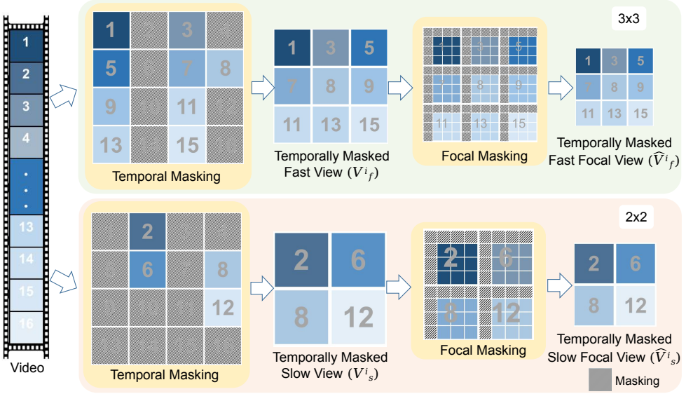
Figure 3: Illustration of two-stage masking of focal views. Temporal Masking drops full frames to generate two different views: the Fast View ( V_f^i ), retaining (approximately) half the frames of the target view of the super image and the Slow View ( V_s^i ) containing approximately a quarter of the same. Subsequently, Focal Masking is applied by selecting a spatially contiguous region and masking all surrounding patches, resulting in the Temporally Masked Fast Focal View \hat{V}_f^i and Temporally Masked Slow Focal View \hat{V}_s^i . This hierarchical masking strategy helps the model attend to the informative regions in both space and time, enabling it to better capture motion patterns and spatial details across different action speeds.
