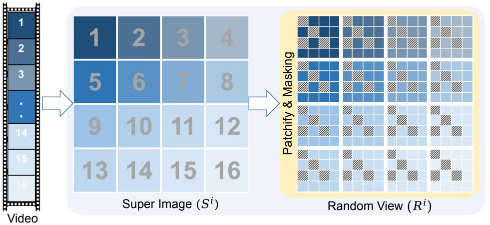
Figure 2: Creation of super image and a random view. Starting from an input video, a super image S^i is formed by arranging M sampled frames into a 2D grid in a row-major format. Each frame is then divided into non-overlapping patches. A random binary mask is applied such that patches at the same spatial location across all frames are masked or retained together enforcing temporal consistency during masking. This results in the Random View ( R^i ). Masked patches are shown in gray for illustration. In practice, the token from that patch is dropped and not passed through the encoder.
