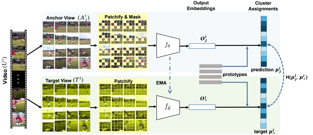
Figure 4: Overview of VideoMSN. Given an unlabeled video clip U^i , equidistant frames are sampled and arranged into a 2D super image. Two different views are generated: the j^{th} anchor view A_j^i , which is randomly masked after patchification and the target view T^i which remains unmasked. Both views are processed using a Siamese architecture. A_j^i is passed through the encoder f_\theta(\cdot) to obtain embeddings \mathbf{O}_j^i , while T^i is passed through the EMA updated target encoder f_{\bar{\theta}}(\cdot) to produce \mathbf{O}_+^i . These representations are then assigned to cluster prototypes, generating a predicted distribution \mathbf{p}_j^i for the anchor and a target distribution \mathbf{p}_+^i for the target. The training objective is to align \mathbf{p}_j^i with \mathbf{p}_+^i using cross-entropy loss H(\mathbf{p}_j^i, \mathbf{p}_+^i) , encouraging the masked anchor representation to match that of the unmasked target.
