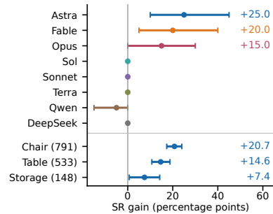
Figure 4: SR gains from reference images, with paired 95% intervals: benchmark (top) and Astra on larger PartNet sets (bottom). Labels give gains in percentage points.
