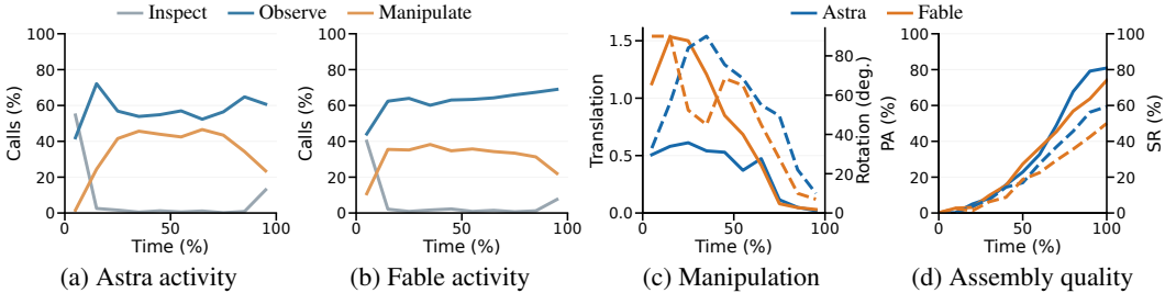
Figure 2: Interaction dynamics of Astra and Fable across 100 evaluations each. (a–b) Mean call shares within active evaluation-bins. (c) Median per-evaluation translation and rotation magnitudes; translation is normalized by the largest-part diagonal. (d) Mean PA and SR. All four plots use benchmark source weights and normalized interaction time. In (c–d), colors identify systems; solid and dashed lines use the left and right axes, respectively.
