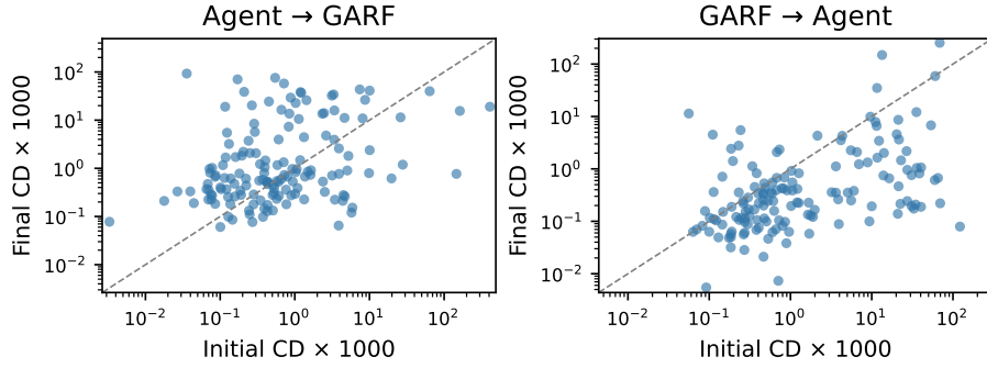
Figure A-5: Per-object changes in shape CD for the two composition orders. Each point is one of the same 150 objects; points below the diagonal improve. Both axes are logarithmic.
