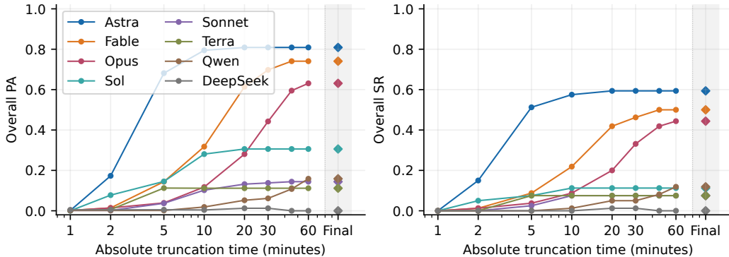
Figure A-2: Recorded-state truncation at absolute budgets. Earlier termination retains the final state. Diamonds in the shaded Final column show untruncated outcomes, not an additional time budget; five episodes have pose changes after 60 minutes of end-to-end time. Terminal values agree with the result tables. These are retrospective curves, not new budget-conditioned agent runs.
