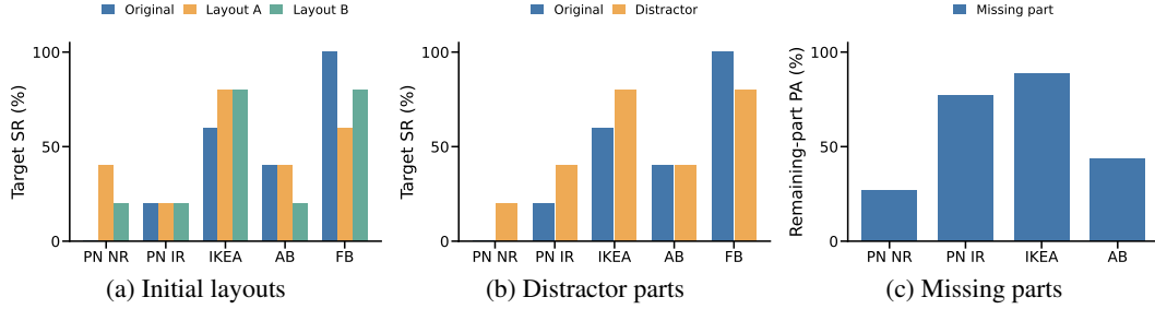
Figure A-6: GPT-6 Astra under task variations on five fixed samples per benchmark block, with one run per condition. PartNet reference conditions share objects and perturbations. Missing-part evaluation measures only retained parts; Fantastic Breaks is excluded from this condition.
