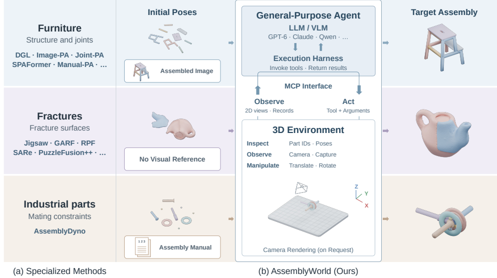
Figure 1: (a) Prior specialized assembly methods across three domains. (b) AssemblyWorld connects a general-purpose model and execution harness to a 3D environment through Model Context Protocol (MCP). Tools return requested views, scene records, or execution status. References guide the agent; initial parts populate the scene. Targets illustrate assembly goals, not agent outputs. Reference conditions, layouts, colors, and the manual icon are illustrative.
