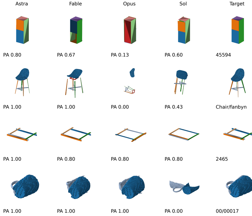
Figure A-3: Four common objects selected near Astra’s median PA in each source, evaluated by Astra, Fable, Opus, and Sol. Columns retain a shared view direction and per-part colors; each view is fitted to its own geometry, so apparent size is not a shared physical scale. Numbers are PA under the common benchmark protocol. The other four systems appear in Figure A-4.
