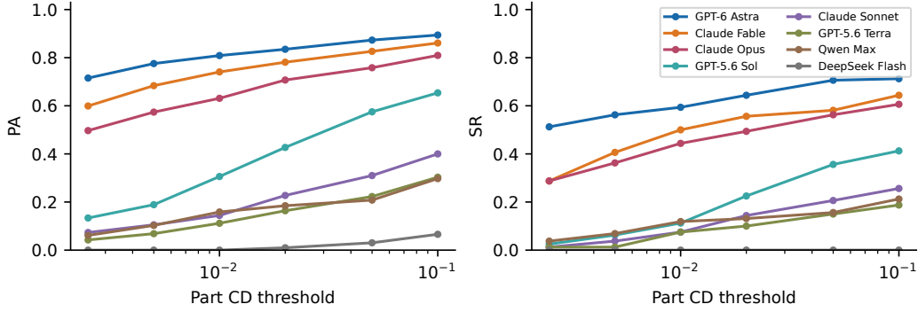
Figure A-1: Correctness-threshold sensitivity for all eight systems. PA/SR use equal source weights; saved registration and Hungarian correspondence remain fixed. The input-shape equivalence threshold remains fixed.
