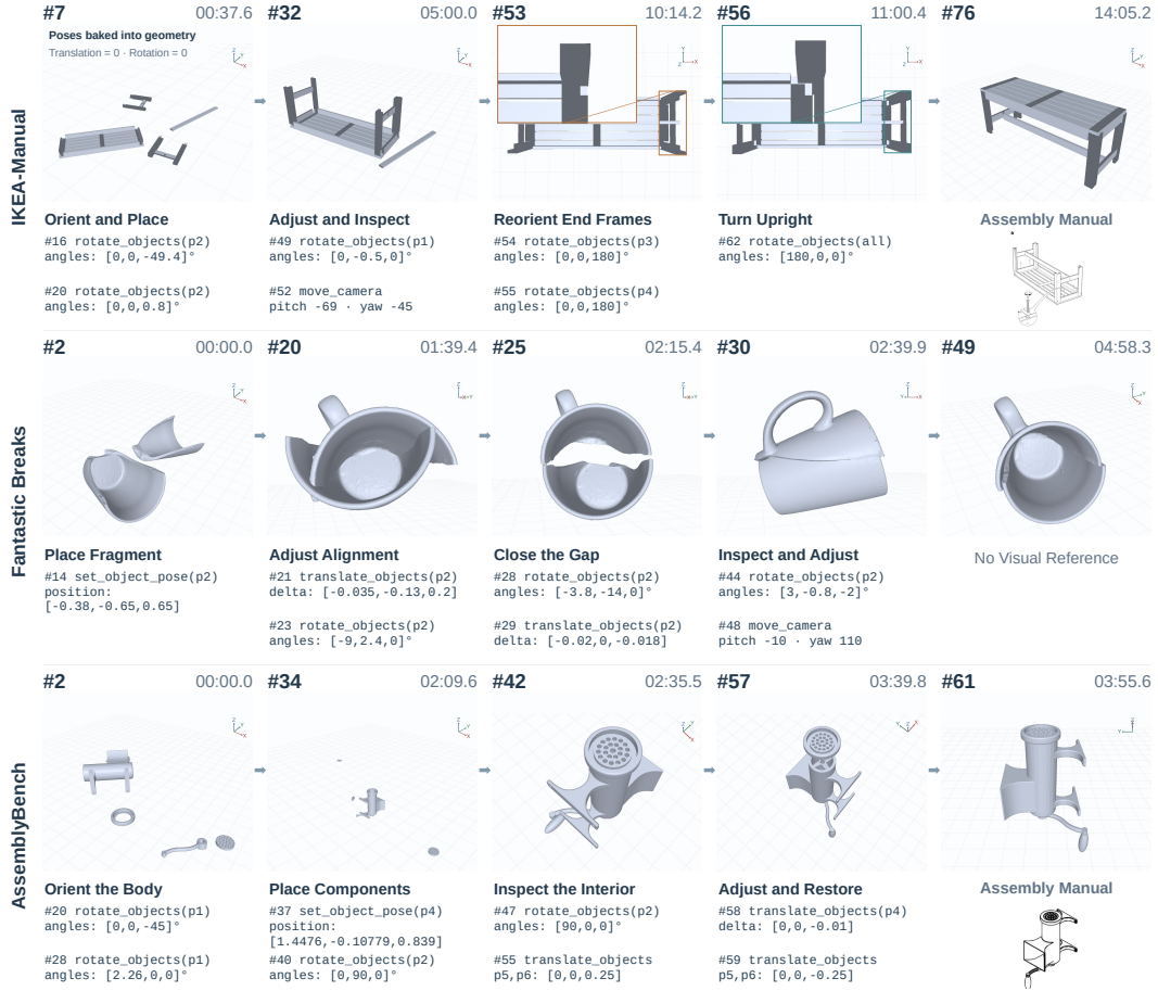
Figure 3: GPT-6 Astra interaction trajectories across three assembly domains. Recorded states are re-rendered from the corresponding camera views. Labels show environment-call numbers (#) and elapsed time; selected MCP calls connect successive views. Insets highlight the IKEA end-frame correction. Part IDs and arguments are abbreviated; angles are in degrees.
