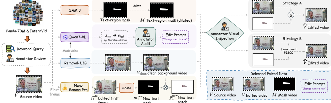
Figure 2: Training data construction pipeline. We compose the four assets ( M , (s_{\text{src}}, s_{\text{tgt}}) , V_{\text{clean}} , and p_1^{\text{new}} ) into the paired edit \hat{V} via Strategy A (alpha composition) or Strategy B (PISCO-based inserter). The overview is in Section 3.1 and implementation details are in Section C.
