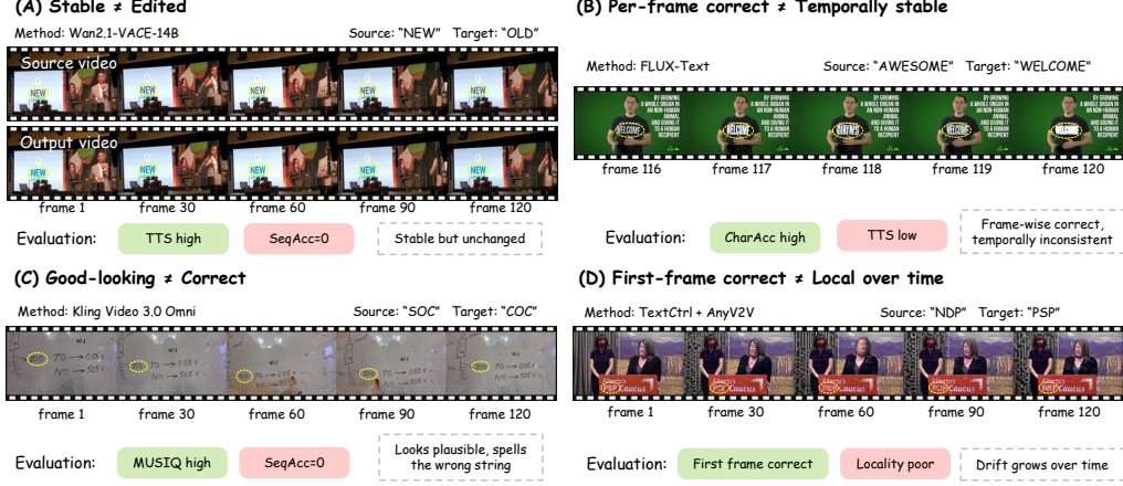
Figure 4: Four representative failure cases. (A) Wan2.1-VACE-14B: masked region returned essentially as the source, target string never rendered. (B) FLUX-Text [11]: per-frame editing yields legible text on individual frames, but the glyph identity is inconsistent between adjacent frames. (C) Kling Video 3.0 Omni [6]: high per-frame visual quality, but the rendered text does not match the requested target. (D) TextCtrl+AnyV2V [10, 13]: the first-frame edit propagates while the rendered text and surrounding scene structure drift away.
