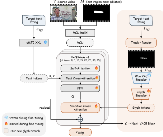
Figure 3: ViTeX-Edit-14B architecture. Three streams condition the VACE backbone: target text s_{\text{tgt}} via frozen uMT5-XXL, source V and mask M via the VCU, and a target-text glyph video pooled by the glyph encoder into tokens E_G . Every VACE block queries E_G through an added condition cross-attention layer. Implementation details are in Section G.
