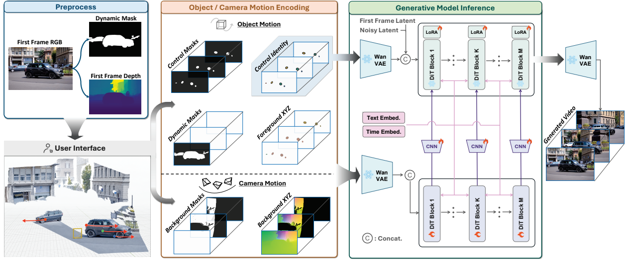
Figure 3: The GenCine 3D control workflow. We estimate depth and a dynamic mask from an RGB image, then lift them into a 3D scene for motion authoring. The artist specifies camera and object motion in a shared world frame using a 3D interface such as Blender. We convert the controls into background XYZ, foreground XYZ, and foreground identity maps, indicating static scene positions, moving handle positions, and handle identity. Validity masks distinguish available guidance from missing values, while the dynamic mask marks the initial foreground. A frozen Wan VAE encodes the maps for the video model. Training pairs videos with guidance recovered from their motion; at inference, the same maps express artist-authored controls.
