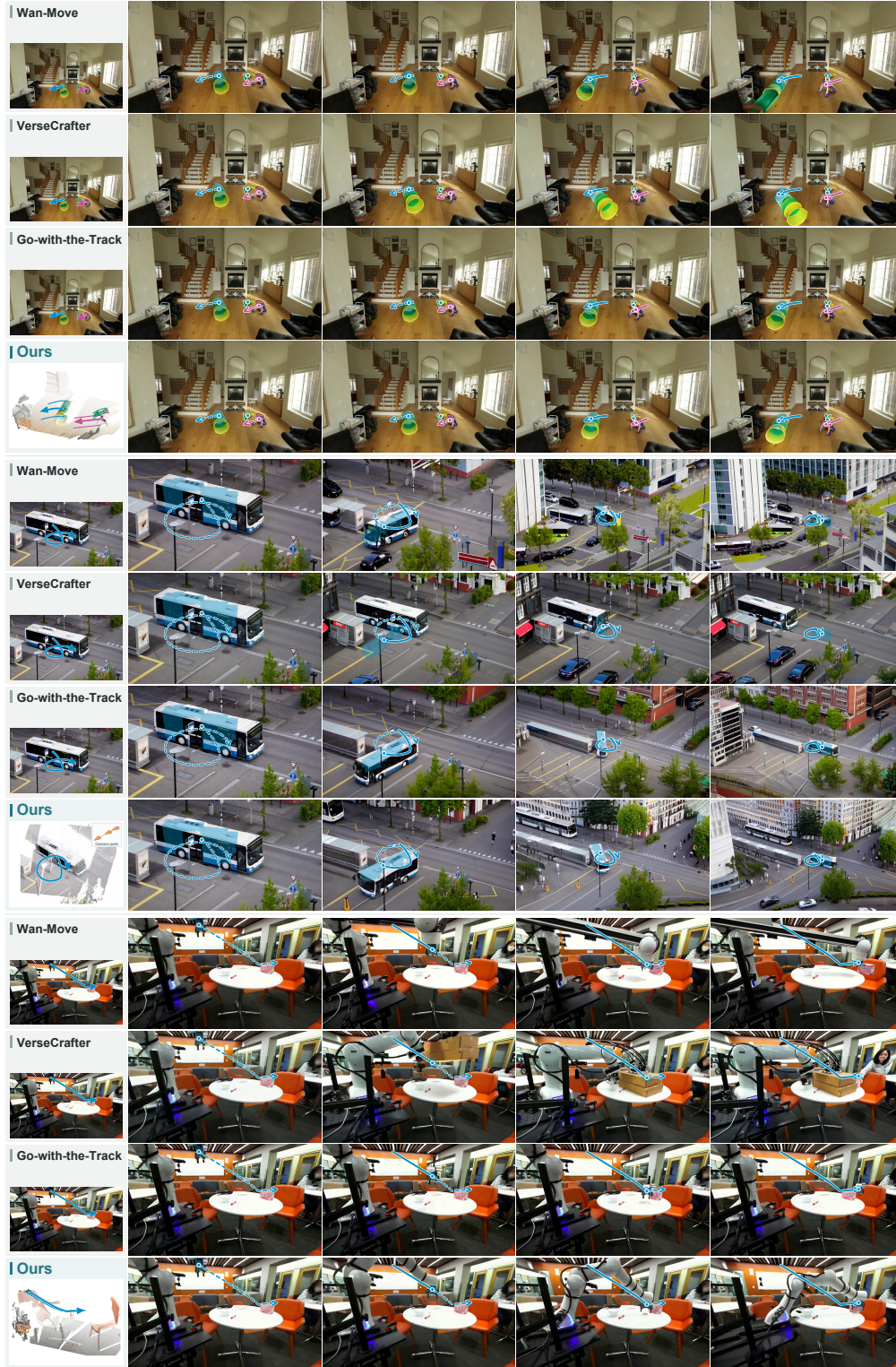
Figure 5: Qualitative comparison on artist-authored motion. Living room, Bus, and Robotic arm (top to bottom) each show Wan-Move, VerseCrafter, Go-with-the-Track, and GenCine (ours), in row order. The first column shows 3D controls (GenCine) or shared 2D projections (baselines); four output frames sample each control interval. Solid/dashed paths show elapsed/remaining target motion, dots mark current targets, and translucent masks show projected target regions.
