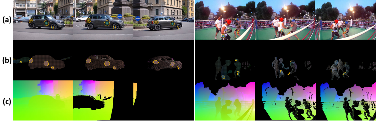
Figure 9: Examples of the three guidance maps. All maps use the same rasterized image-plane interface. (a) Foreground identity maps overlaid on RGB frames. Each artist-selected 3D handle region is rendered with a fixed identity color through its projected Gaussian footprint. (b) Foreground XYZ maps encode the current 3D positions of handle points as RGB values. (c) Background XYZ maps encode the world positions of valid static points. Both XYZ maps share one per-axis normalization, placing their values in the same coordinate system.
