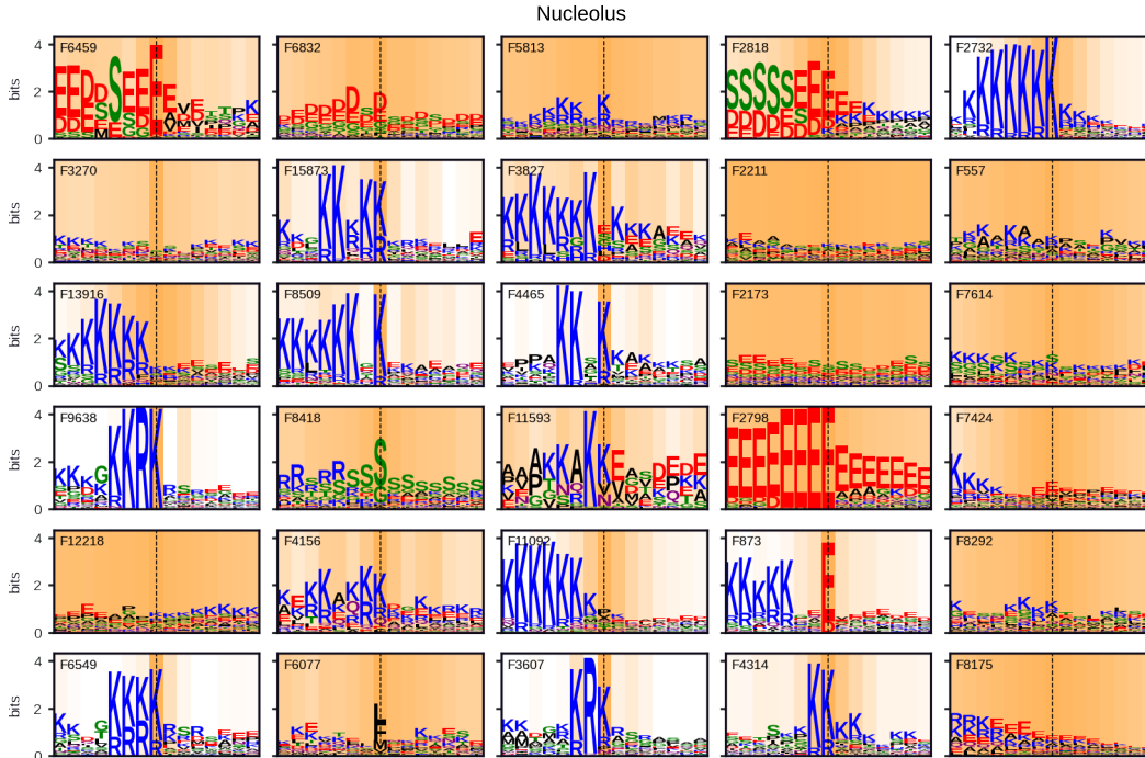
Figure 13: Nucleolus. Logo plots of the top-30 enriched features.
