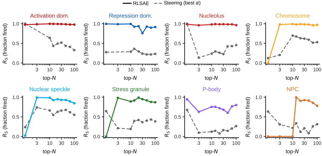
Figure 10: Feature activation fraction versus top- N . For all 8 sequence sets (2 transcriptional effector sequences and 6 compartment association sequences) the average fraction of target features which fire within generated sequences, R_S , as a function of top- N , for RL-SAE (solid colored lines) and activation steering (grey dashed lines). R_S for steering is presented at the best \alpha value across the sweep, regardless of whether that \alpha passes the sequence entropy threshold (i.e. steering R_S values presented here are a generous upper bound).
