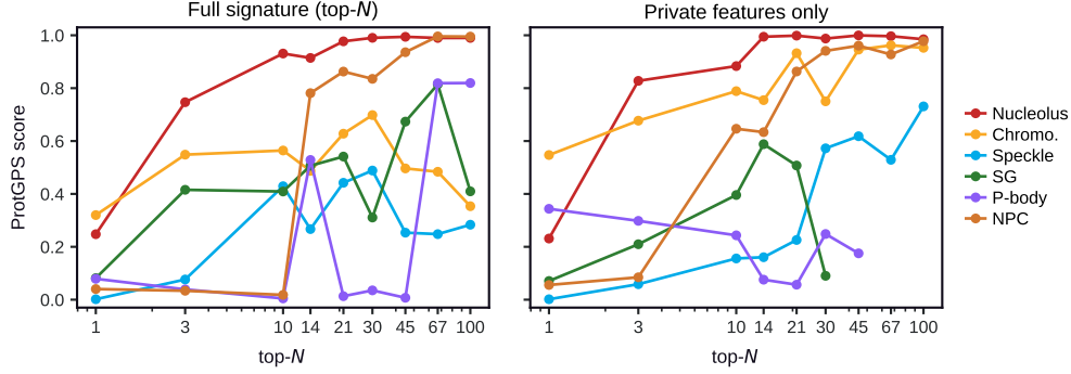
Figure 8: ProtGPS dose-response against top- N . Left: Average ProtGPS score for sequences generated after RL-SAE on the top- N features per compartment. Right: Average ProtGPS score for sequences generated after RL-SAE on the top- N features which are private to the given compartment. Stress granule and P-body only have 36 and 55 private features, respectively.
