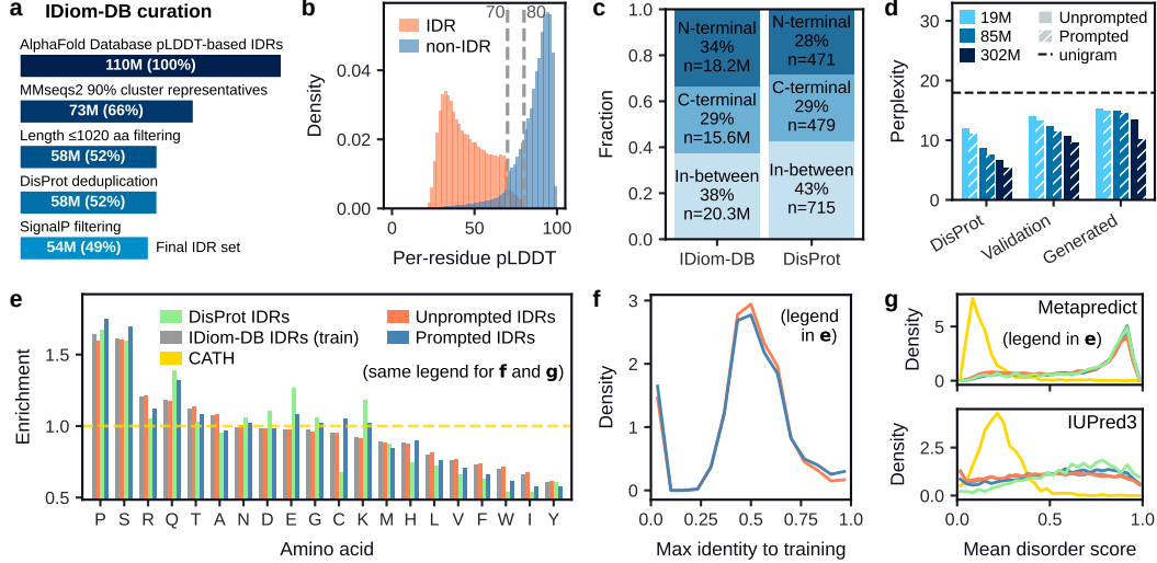
Figure 1: Training on 54M curated IDRs enables the generation of diverse and biologically plausible IDRs. (a) IDiom-DB curation workflow. (b) AlphaFold2 pLDDT distribution of curated IDRs and non-IDRs. (c) Fraction of curated training IDRs and experimental DisProt IDRs which are located at the N-terminus, C-terminus, and internally. (d) IDiom model perplexity on DisProt, validation, and generated IDRs. Solid and hatched bars indicate unprompted and prompted IDRs, respectively. (e) Amino acid compositional enrichment for training, generated, and DisProt IDRs, relative to the folded CATH sequences’ compositions. This panel’s legend also applies to panels (f) and (g). (f) Sequence identity of generated IDRs relative to training set IDRs, calculated with MMseqs2. (g) Predicted disorder scores of training, generated, and DisProt IDRs, alongside CATH sequences (higher is more disordered).
