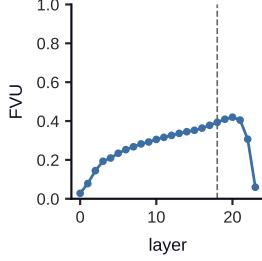
Figure 7: Sparse autoencoder layer sweep. Fraction of variance unexplained (FVU) per layer, evaluated on 10K held-out validation records ( k = 32 , expansion \times 16 ). The layer-18 is marked by the vertical dashed line.
