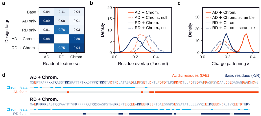
Figure 4: Feature compatibility determines the organization of sequences with composed features. (a) Fraction of features activated in each target feature set by sequences generated under each RL-SAE condition. The chromosome feature set is private-30. (b) Distribution of the per-sequence Jaccard overlap between residues which fire on chromosome association features versus on activation domain or repression domain features. Curves show each design and a position-shuffled null. (c) Distribution of charge patterning \kappa parameter for chromosome + AD/RD, and scrambled variants. (d) Example generated chromosome + AD/RD sequences showing feature firing positions for chromosome association (light blue) and the activation domain (AD, upper, red) or repression domain (RD, lower, dark blue).
