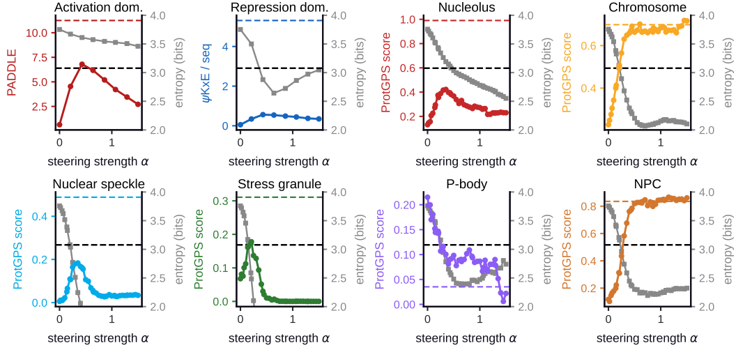
Figure 11: Steering dose-response at N = 30 . Here, we plot the various scoring metrics (PADDLE, \psi KxE, NDSM, and ProtGPS) versus activation steering strength \alpha at top- N = 30 . The metrics are plotted as colored curves (left axis), and the generated sequence entropies are plotted as grey curves (right axis).
