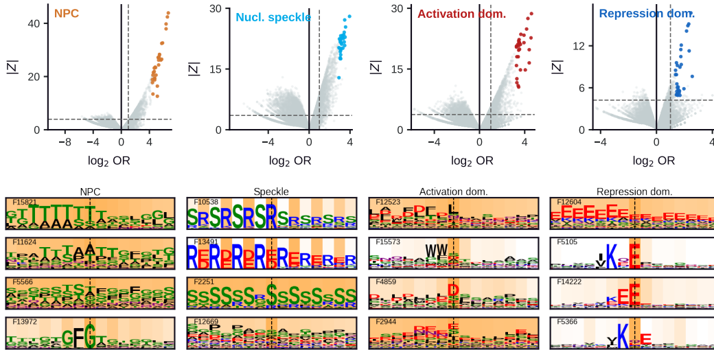
Figure 2: Enriched SAE features recover canonical IDR sequence grammars. Top row: Statistical significance |Z| versus \log_2 odds ratio (LOR) for all 16,384 IDiomSAE features in nuclear pore complex, nuclear speckle, transcriptional activation, and repression sequence sets. Dashed lines mark \text{LOR} = 1 (vertical) and the false discovery rate threshold of 10^{-3} (horizontal). Features in the upper right quadrant pass both thresholds. Bottom row: Information content logos for each set’s top-four enriched features, showing residue likelihoods within a \pm 7 -residue window around peak firing positions (vertical dashed line position). Orange shading indicates the feature activation strength at each residue position. Logo construction is described in Appendix R.
