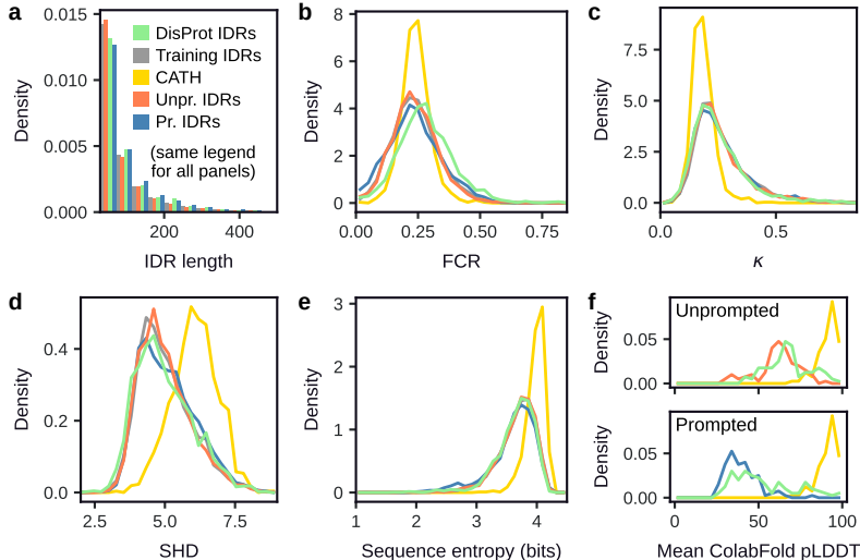
Figure 6: Characterization of training IDRs, Idiom-generated IDRs, DisProt IDRs, and CATH sequences. (a) Distribution of training, generated, and DisProt IDR lengths. The legend in this panel applies to all other panels in this figure. (b) Distribution of the fraction of charged residues (FCR) for training, generated, and DisProt IDRs, and CATH sequences. (c) Distribution of charge patterning \kappa parameter. (d) Distribution of sequence hydropathy decoration (SHD). (e) Distribution of sequence entropy. (f) Distribution of AlphaFold2 scores for CATH sequences, Idiom-generated IDRs, unprompted (upper) and prompted (lower), as well as DisProt IDRs without surrounding context (upper) and with context (lower).
