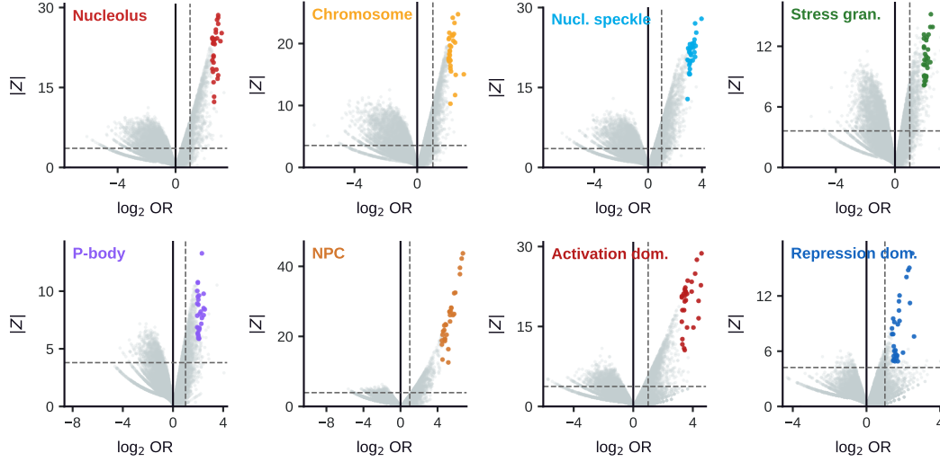
Figure 12: Feature enrichment plots for all eight sequence sets. Feature enrichment plots (hypergeometric |Z| versus \log_2 odds ratio (LOR)) for all 8 sequence sets. The top-30 features as ranked by LOR are the colored dots. The horizontal dashed line marks the FDR threshold, and the vertical dashed line marks the \text{LOR} \geq 1 threshold.
