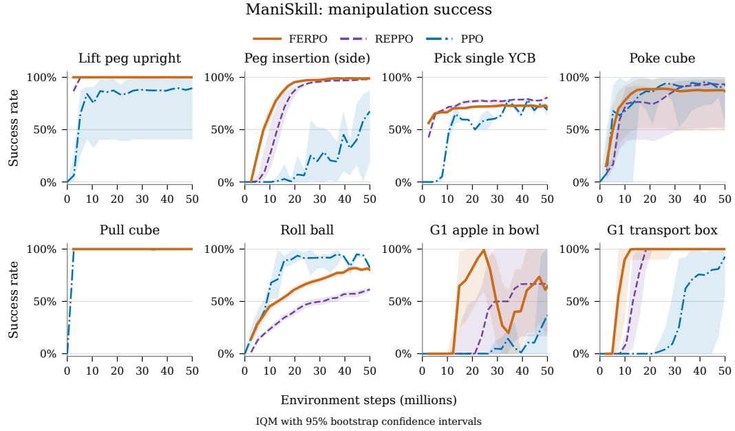
Figure 15: All eight ManiSkill tasks. All methods show success-rate IQM with pointwise 95% bootstrap confidence intervals. FERPO uses 20 seeds per task except G1 transport box (ten). PPO uses one configuration across all eight tasks; REPPO uses the official published trial CSVs.
