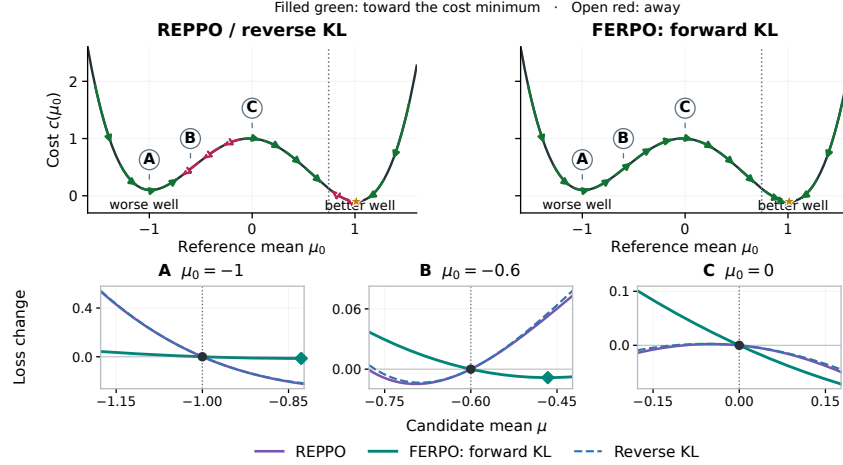
Figure 1: Actor directions and local losses. Top: green/red arrows point toward/away from the cost minimum (star); lengths are illustrative, not convergence guarantees. Bottom: frozen-reference losses at A–C, zeroed at the reference; KL losses are scaled by T . Details: Appendix A.1.
