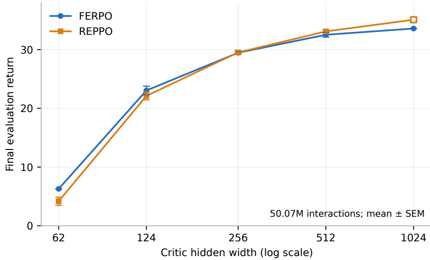
Figure 8: Final return versus critic width on G1. Points show seed means and error bars show one SEM. The open square marks the single-seed REppo reference at width 1,024, for which no error bar is reported. Both methods lose substantial return at width 62; FERPO reaches 6.29 and REppo 4.19. These endpoints do not identify the source of critic approximation error.
