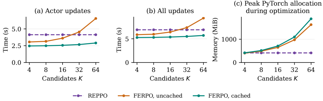
Figure 2: Update cost on an A100. Medians and ranges over three repetitions with 131,072 rollout states. Actor time includes cache construction; total updates include critic training. PyTorch allocation excludes simulation and unused reservations.
