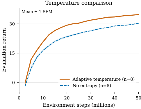
Figure 7: Temperature learning curves. Adaptive temperature versus no entropy regularization at K = 16 . Both curves show seed means with one-SEM bands. Both curves use eight completed seeds at every evaluation; the adaptive control uses corrected temperature learning rate 0.0003. Final returns are 34.81 \pm 0.24 with adaptive temperature and 30.32 \pm 0.27 without entropy regularization. The final evaluations also appear in Figure 3 (left).
