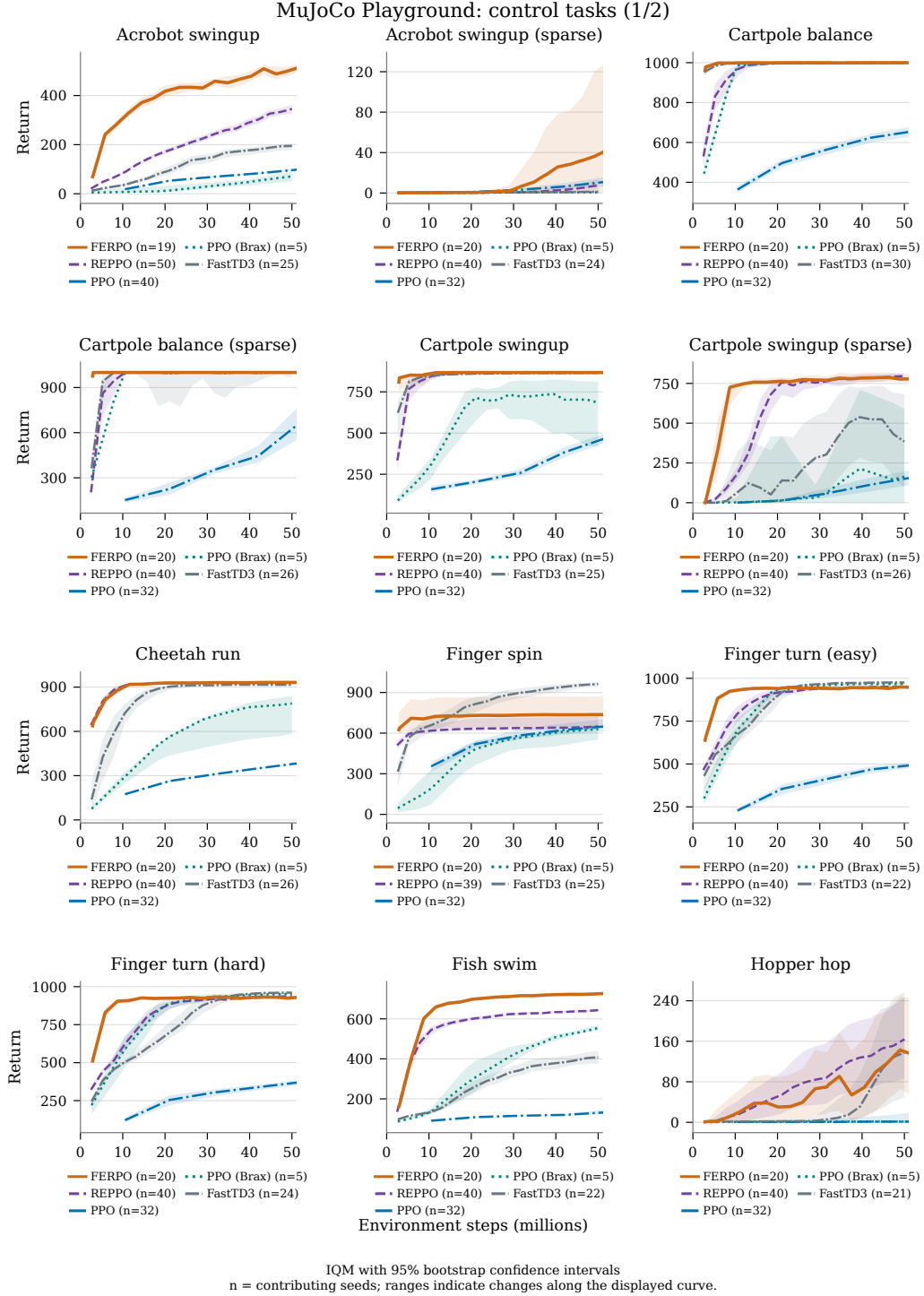
Figure 12: DMC learning curves (1/2) . The first 12 of 22 tasks. All methods show IQM with pointwise 95% bootstrap confidence intervals. Legends report contributing seeds n ; ranges indicate changes across the displayed evaluations. Curves retain their source evaluation schedules. Baseline configurations are fixed across all DMC tasks as specified in Table 3.
