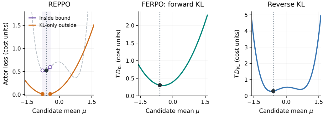
Figure 5: Frozen-reference losses at B. Left: REppo’s active expected-cost/entropy branch (purple) and KL-only branch (orange); the pale dashed curve extends the inactive cost branch. Open and filled endpoints show the loss switch. Middle: forward KL from the fixed FERPO target to the candidate Gaussian. Right: reverse KL to that same target. Both KL curves are scaled by T = 0.15 ; this positive scaling preserves directions. Vertical dotted lines and black dots mark the reference \mu_0 = -0.6 .
