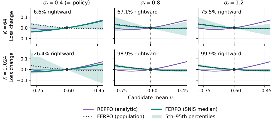
Figure 6: Wider proposals recover the population fitting loss. Losses at B with the same reference policy and target throughout. Teal: SNIS median and pointwise 5th–95th percentiles across 5,000 batches; dotted black: population FERPO; purple: analytic REPO. Percentages give the frequency of rightward SNIS directions. Shading shows batch variation, not confidence intervals for the mean. Losses are zeroed at the reference, and forward losses are scaled by T .
