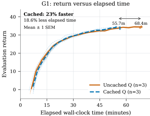
Figure 9: Cached versus uncached Q against elapsed time. G1 deterministic evaluation return for seeds 3–5 per method on the same Vega A100 node. Both use K = 8 and eight critic epochs on the full rollout. Bold curves and one-SEM bands use linear interpolation at common times; faint curves show individual runs. The arrow marks mean completion times at 50,069,504 interactions: 55.7 versus 68.4 minutes. At 50 minutes, interpolated mean returns are 33.55 cached and 32.86 uncached. Figure 3 (middle) shows all five seeds against environment interactions.
