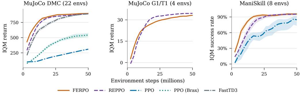
Figure 4: Benchmark learning curves. IQM with equal environment weights and equal seed weights within environments. Bands: pointwise 95% confidence intervals from 10,000 within-environment bootstrap resamples. G1/T1 FERPO uses K = 16 , ESS target 0.65, and eight seeds per task. Details: Appendix A.3.
