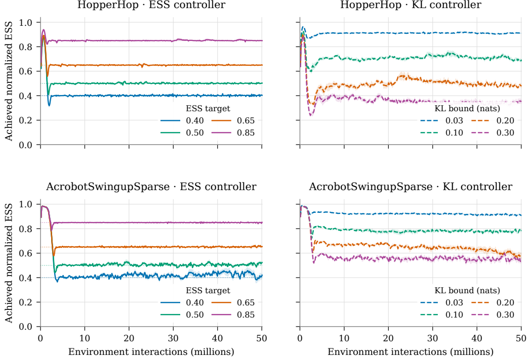
Figure 11: Achieved ESS under both controllers. Per-iteration geometric mean of normalized SNIS ESS under direct ESS control (left) and policy-KL control (right). Curves show unsmoothed means with one-SEM bands across 12 seeds. Dotted lines mark ESS targets; right-panel legends give policy-KL bounds in nats.
