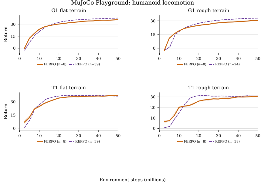
Figure 14: All four G1/T1 locomotion tasks. FERPO and official REPPPO trials show IQM with pointwise 95% bootstrap confidence intervals. FERPO uses K = 16 , normalized ESS target 0.65, and eight completed seeds per task; legends report each method’s seed count. Results use the recorded evaluation protocols described in Appendix A.3.7.
