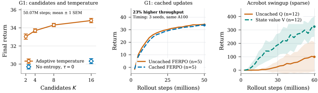
Figure 3: Ablations. Left: G1 candidate count and temperature at 50.07M steps (eight seeds for K = 2, 16 and \tau = 0 ; ten for K = 4, 8 ). Middle: cached versus uncached G1 updates ( K = 8 ). Right: state-value versus Q critics on AcrobotSwingupSparse (sparse rewards, K = 16 ). Means with one SEM (left, middle) or one SD (right); panels use separate controls. The state-value variant uses 17\times more simulator transitions per rollout step.
