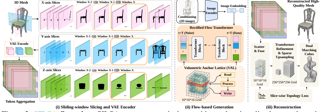
Figure 2: SILSA Overview. SILSA represents each shape with overlapping slice latents along the x , y , and z axes. A topology-aware SliceVAE encodes surfaces into fixed multi-axis slice latents and decodes them through sparse volumetric upsampling into a high-resolution mesh. An image-conditioned rectified-flow transformer generates these latents, using a Volumetric Anchor Lattice as shared 3D memory for cross-axis coordination. Slice-wise persistent-homology and Betti-transition losses supervise connected components, holes, and topological consistency during VAE training.
