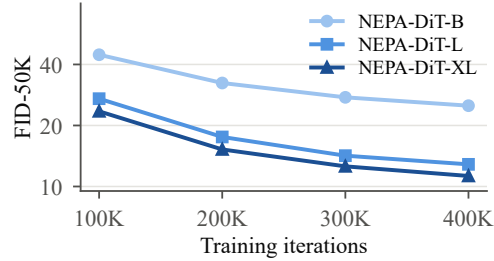
Figure 6: Training progress of NEPA-DiT-B/L/XL, FID-50K without guidance.
