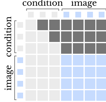
Figure 4: Attention mask. Rows are queries and columns are keys; dark cells are masked.
