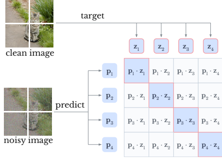
Figure 5: Embedding prediction loss.
