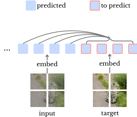
Figure 1: Multi-embedding prediction.
