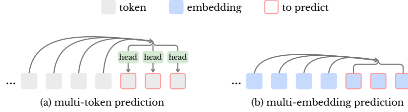
Figure 2: Multi-token vs. multi-embedding prediction. Both predict several items at once. (a) Tokens are discrete, so hidden states are decoded into tokens by output heads. (b) Embeddings are continuous, so the outputs of the model are the predictions themselves. In both, the same context predicts all targets in one forward pass.
