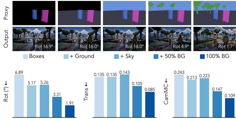
Figure 5 Proxy composition and camera control. LynnReal-Omni on 20 scene-camera pairs, from entity boxes only to adding ground, sky and 50% of the background objects. Top: scene 043 at 4.25 s; the overlay gives the mean rotation error of that video. Bottom: means over the 20 pairs (lower is better). The 100% BG reference uses the original prompts and first-frame setting and is not a controlled step.
