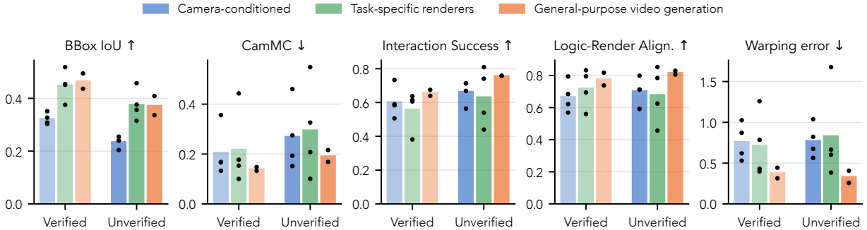
Figure 3 Method classes at a glance. Main-track results per method class in Verified-FF (light) and Unverified-FF (dark). Bars show class means, dots the individual methods. Camera-conditioned: EchoWM, SANA-WM, LingBot 2.0, AlayaWorld v1.1; task-specific renderers: Cosmos-Transfer2.5, C2R, CWM, LynnReal-Omni; general-purpose video generation: MiniMax-H3, Seedance 2.5.
