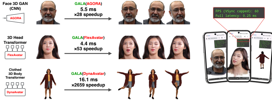
Figure 1: GALA enables efficient, high-fidelity animation across diverse Gaussian avatar models. By introducing shared blendshapes and a lightweight coefficient predictor, GALA accelerates CPU animation by up to three orders of magnitude and enables real-time deployment on mobile devices.
