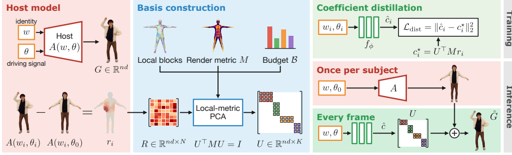
Figure 2: Overview of GALA. Residuals r_i of the host model A with respect to the neutral avatar A(w_i, \theta_0) (Section 3.2.1) are decomposed by a spatially local, rendering-aware PCA under a memory budget \mathcal{B} into the block-diagonal basis U (Section 3.2.2). A coefficient network f_\phi is trained to regress the projected coefficients c^* (Section 3.2.3). At inference, the neutral avatar is computed once per subject, and every frame costs one evaluation of a shallow network f_\phi and a linear blend.
