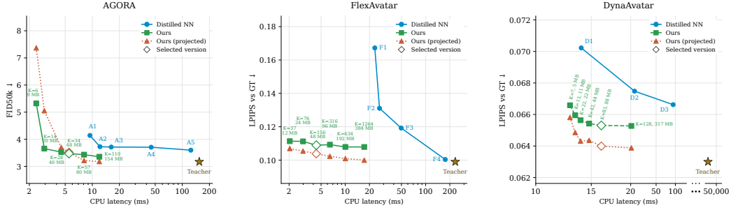
Figure 4: Comparison to alternative distillation: quality against the CPU time of the animation step, lower is better on both axes. Teacher is the host model, our models are labeled with the components per Gaussian and the basis size, and the diamond marks our final model.
