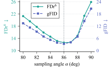
Figure A22: Sampling angle \alpha with 1-step generation using Sphere2-B trained on ImageNet 256 \times 256 . \text{FDr}^6 and FID agree in a “U” shape along the angle, with the best quality at 86^\circ .
