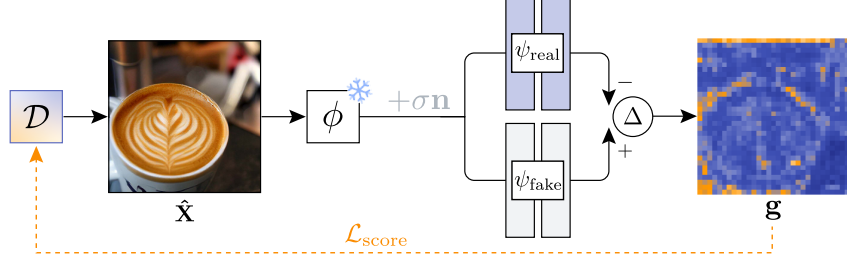
Figure 7: Score matching loss. Fake features from the frozen extractor \phi are denoised by the real and fake score models (each a two-layer transformer EDM denoiser (Karras et al., 2022)), and their difference gives the direction \mathbf{g} that pulls fake features toward real ones. During transport, both score models are frozen and run once each; only the decoder \mathcal{D} is updated by \mathbf{g} through \mathcal{L}_{\text{score}} .
