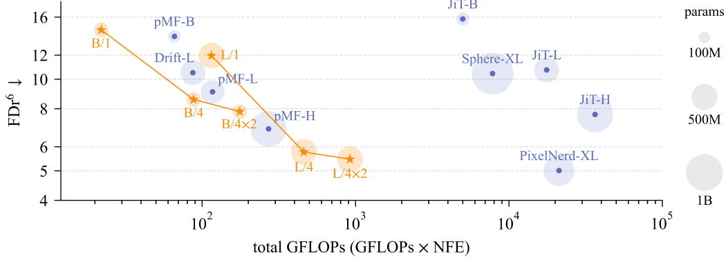
Figure 9: Generation quality vs. sampling compute on ImageNet 256 \times 256 among pixel-space models. Circles are pixel-space baselines and stars are Sphere2 at 1, 4 (without CFG) and 4 \times 2 NFE (with CFG), joined per model. The halo area around each marker is proportional to parameters.
