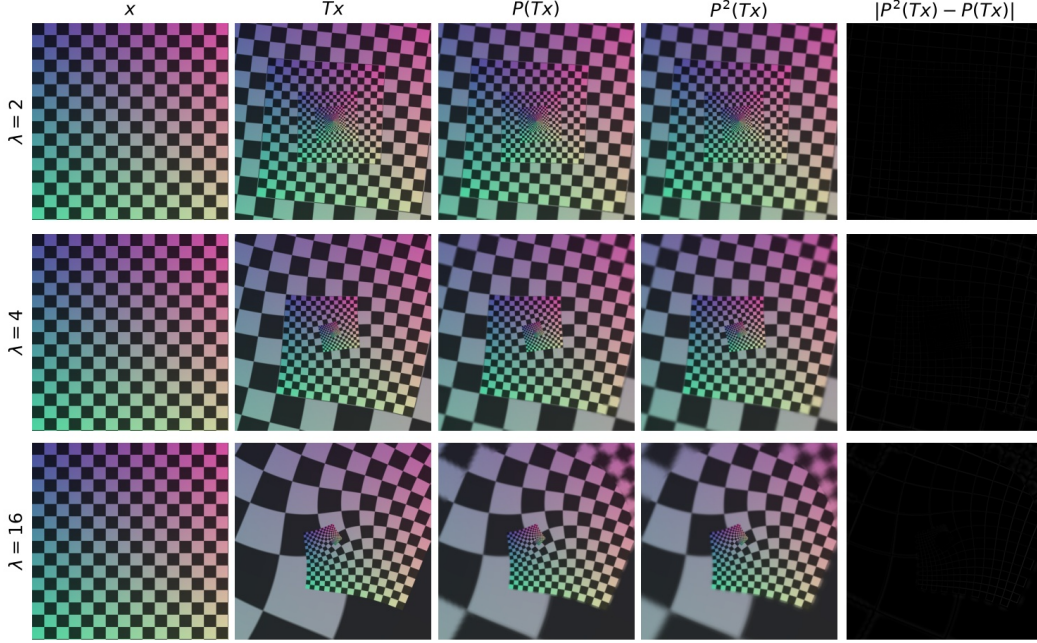
Figure 10: Checking geometric round trips. From left to right: x , Tx , P(Tx) , P^2(Tx) , and the residual |P^2(Tx) - P(Tx)| , where P = TT^\dagger . Rows use deck ratios \lambda = 2, 4, 16 . The three transformed images coincide in the continuous construction; the rasterized comparison shows blur and residual differences near checkerboard edges. The measured residual |P^2(Tx) - P(Tx)| is 0.011, 0.012, 0.014 (top to bottom), each at the bilinear-resampling floor.
