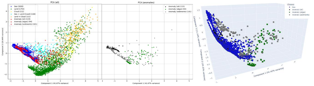
Fig. 3. PCA analysis of labeled patches in the encoder's latent space. The left figure shows the separation of different patch classes (anomalies in red), the middle figure colors anomalies by type, and the 3D PCA on the right illustrates the separation between sea and anomalies. Patch counts per label are indicated in the legend.
