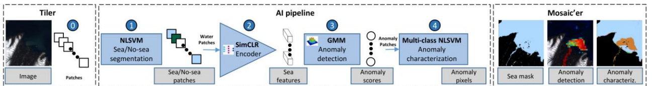
Fig. 1. Architecture of the anomaly detection pipeline: The Tiler (0) splits the input image into patches, which are processed by the AI pipeline. Sea patches are filtered (1), encoded into a latent space (2), and analyzed for anomalies (3). Anomalies are segmented (4) to identify their type. The Mosaic'er then recombines the patches for visualization.
