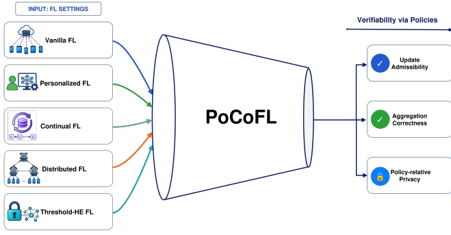
Fig. 1. PoCoFL system model linking FL settings, policy predicates, and verifiability guarantees.
