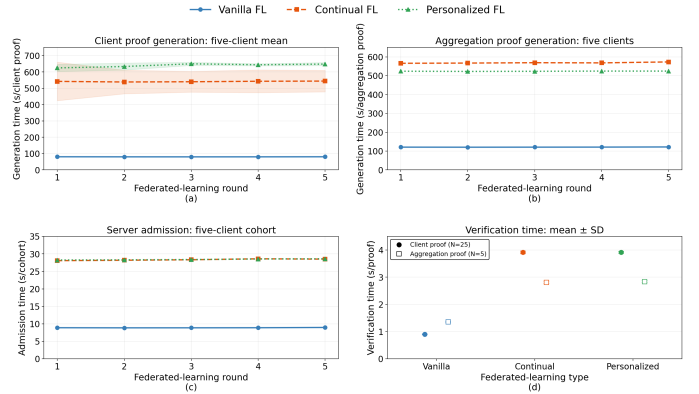
Fig. 3. EZKL timing over five rounds at K = 5 : (a) mean client-proof generation, (b) aggregation-proof generation, (c) five-client cohort admission, and (d) mean proof-verification time. Shading in (a) and error bars in (d) show \pm one sample standard deviation.
