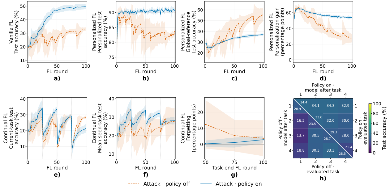
Fig. 2. Effect of policy enforcement under model-poisoning attacks in vanilla (a), personalised (b-d), and continual (e-h) FL. Shading denotes standard deviation across five paired seeds. In (h), upper/lower triangles show policy enforcement on/off, respectively.
