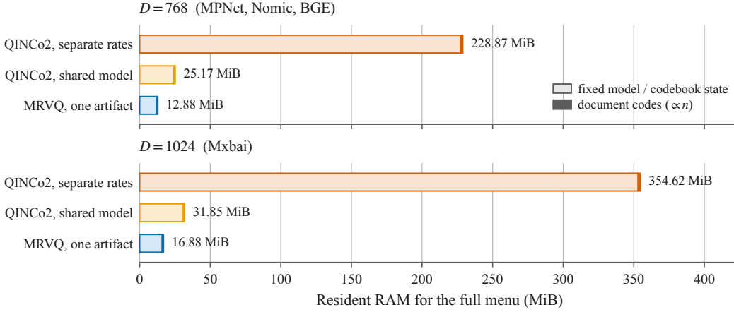
Figure 3: FiQA ( n = 57.6 k) resident RAM for the full rate menu, split into fixed model or codebook state and the document codes that grow with n . The code term is a thin sliver at this corpus size, which is why the measured ratios in Table 1 are far above the asymptotic 1.75\times .
