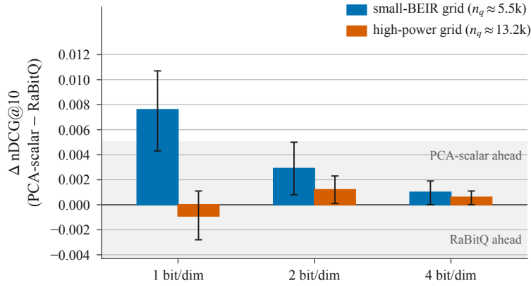
Figure 4: PCA-scalar – RaBitQ / Extended-RaBitQ nDCG@10 at matched nominal bits per dimension, with 95% paired-bootstrap intervals. Positive values favor PCA-scalar; the shaded region is the pre-specified \pm 0.005 practical-equivalence band.
