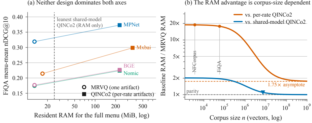
Figure 2: (a) FiQA menu-mean nDCG@10 versus resident RAM for the full menu. MRVQ ( \circ ) occupies the low-memory corner and per-rate QINCo2 ( \square ) the high-quality corner; neither dominates on both axes. The dashed line marks the leanest shared-model QINCo2 RAM, whose quality we do not measure. (b) The same accounting as a function of corpus size at D=768 . The advantage over per-rate QINCo2 decays from \sim 18\times at the evaluated corpora to the 1.75\times code-stream asymptote, and the shared-model advantage falls below 1.1\times at n=7.3\text{M} ( \blacktriangledown ).
