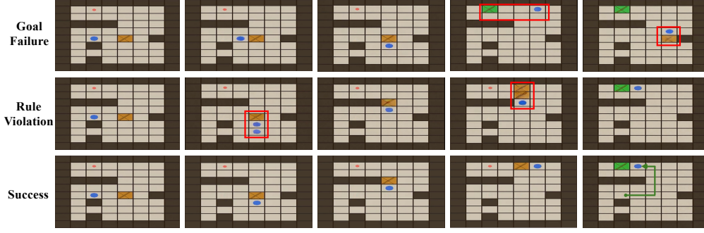
Figure 5: Failure Modes of Standard AR.
