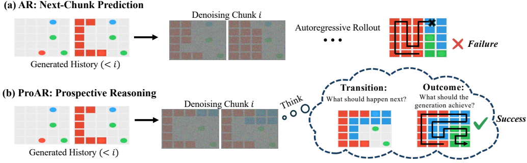
Figure 1: Overview of ProAR. (a) Standard AR relies on local next-chunk prediction, leading to trajectory drift and task failure. (b) ProAR introduces prospective reasoning to anticipate immediate transitions and final outcomes, guiding generation toward task success.
