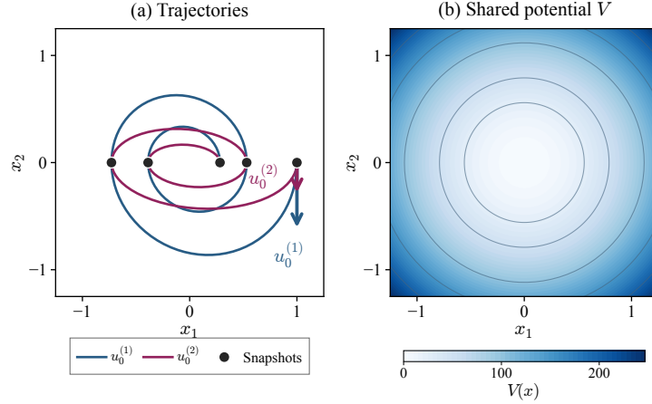
Figure 6: Snapshots are not identifiable without the initial velocity. Left: simulated trajectories with their individual initial velocities pass through the same points and are therefore not identifiable from them. Right: shared circular potential.
