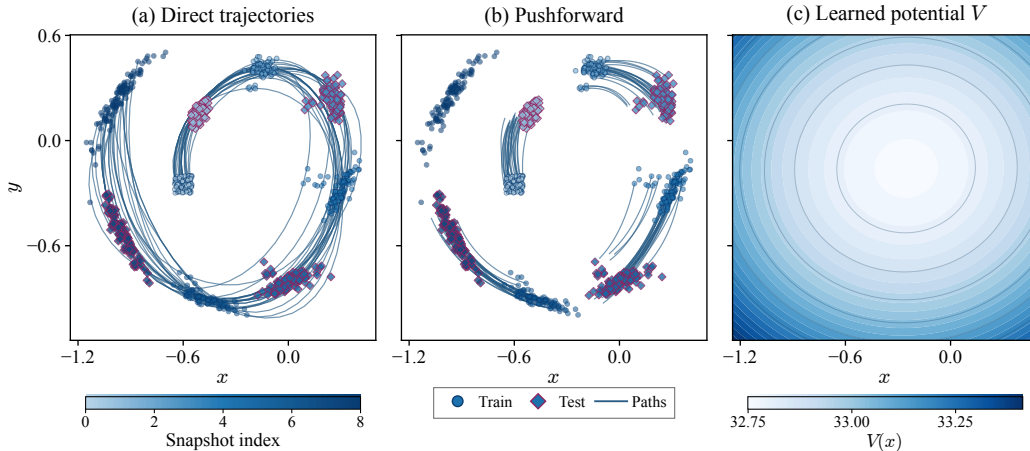
Figure 10: Double-Stitch predictions on the small ocean vortex ( V(x) , seed 0). Left: learned trajectories (used for direct evaluation). Center: pushforward predictions (used for pushforward evaluation). Right: learned potential.
