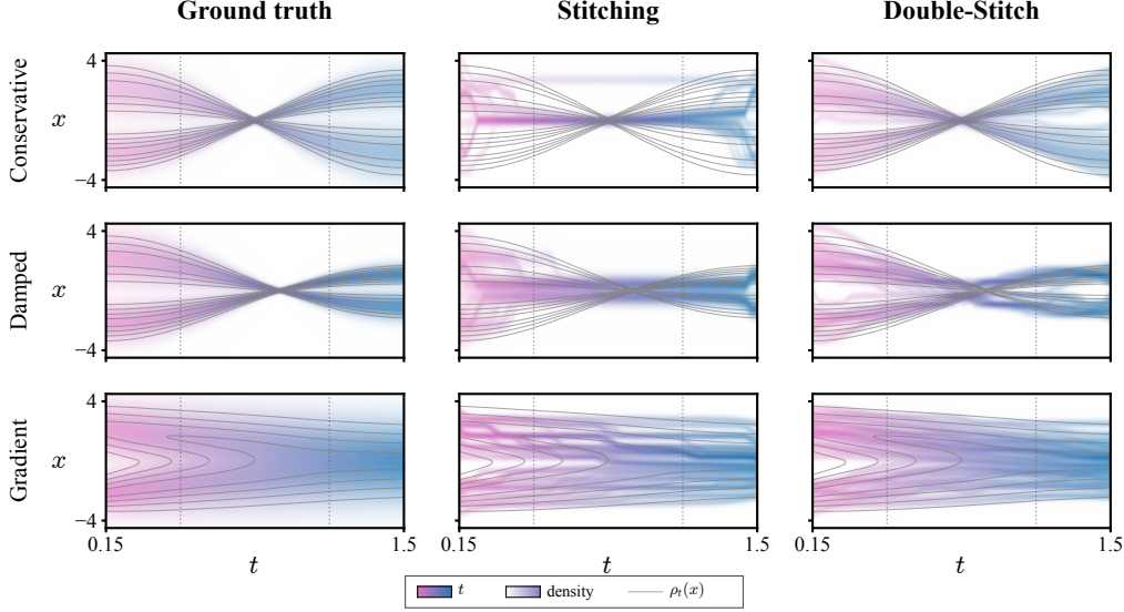
Figure 11: Double-Stitch learns all three Gaussian-mixture flows. Left: ground-truth conservative, damped and gradient densities. Center: Stitching, which fails on the conservative flow and underperforms on the damped flow. Right: Double-Stitch, which succeeds on all three. Dotted lines mark the held-out times.
