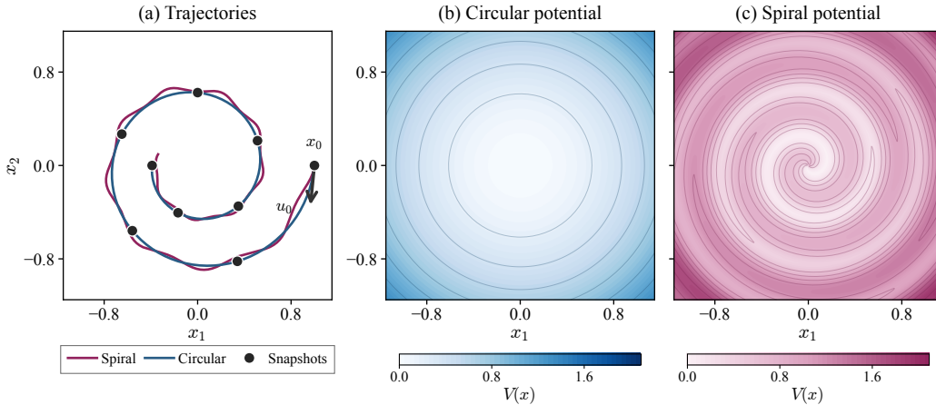
Figure 7: Potentials are not identifiable from only snapshots. Left: simulated trajectories with their shared initial velocities pass through the same points and are therefore not identifiable from them. Right: the potentials that produced the corresponding trajectories.
