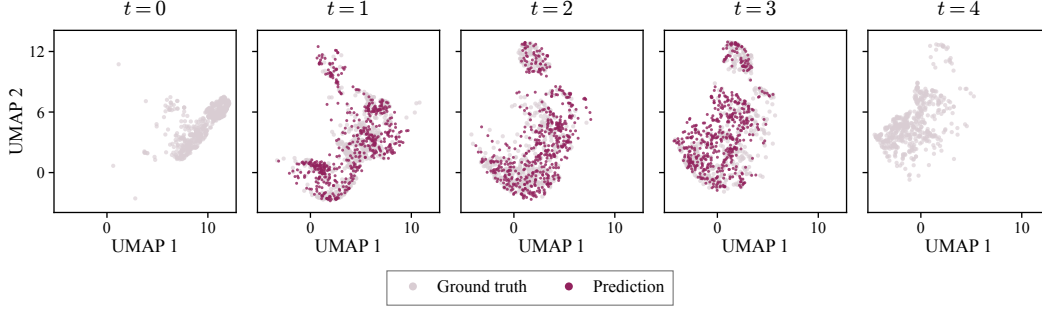
Figure 8: Double-Stitch predictions on EB L1O ( V(x) , seed 0). Shared UMAP. Pale points are ground truth, dark points are predictions.
