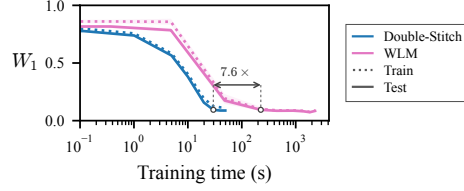
Figure 2: Training on synthetic WHF (mean \pm std, 3 seeds). Static methods. Arrow shows the training time ratio at test W_1 \approx 0.09 .
