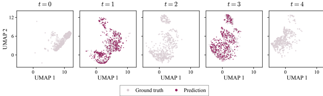
Figure 9: Double-Stitch predictions on EB L2O ( V(x) , seed 0). Shared UMAP. Pale points are ground truth, dark points are predictions.
