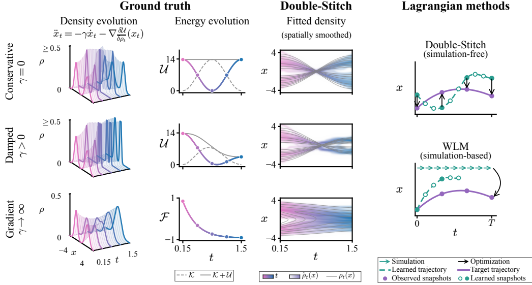
Figure 1: Simulation-free fitting across three dynamical regimes. Left: conservative, damped and gradient-flow examples, with analytic densities, energies and Double-Stitch fits. Right: schematic training procedures for Double-Stitch and WLM. Grey curves show kinetic and total energy for the oscillators; the gradient-flow panel shows free energy. Grey contours show analytic densities.
