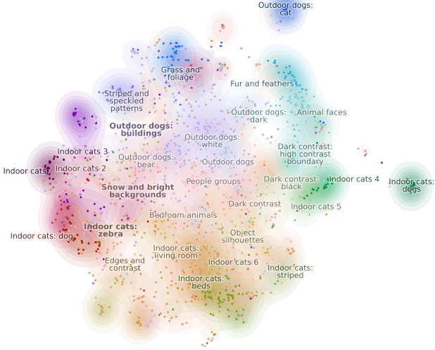
Figure 4. UMAP of outlier activations after projection into CLIP space. The feature organization remains consistent with the texture-sink interpretation.
