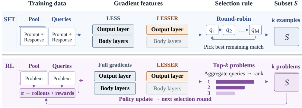
Figure 2: Data selection with output-layer gradient features in SFT and RL. Pool and query representations determine similarity scores, while the selection rule produces the training subset. LESSER replaces the gradient representation within this pipeline.
