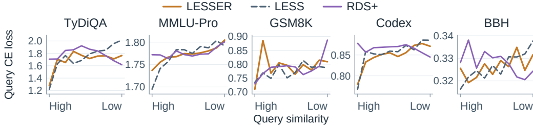
Figure 9: Qwen3-4B-Base: query loss across similarity bins. Each bin uses one training run; bin 0 is closest to the queries.
