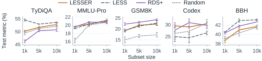
Figure 3: LESSER closely tracks LESS on downstream performance. Panels show Llama-2-7B; values are means over three training seeds, and error bars show one sample standard deviation. Across all 60 model–task–budget cells, the absolute score gap of LESSER averages 1.3 points against LESS, 2.2 against RDS+, and 2.6 against Random.
