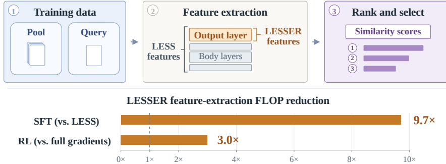
Figure 1: Efficient data selection with output-layer gradients. Given a candidate training pool and a small query set representative of downstream tasks, LESSER extracts output-layer gradient features to rank and select training examples. These features approximate the downstream behavior of full-gradient methods like LESS while substantially reducing feature-extraction FLOPs.
