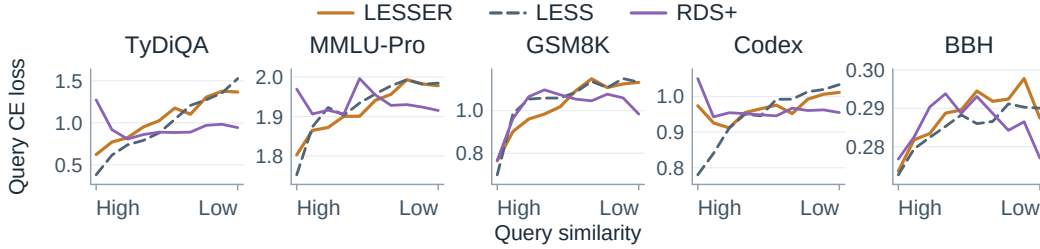
Figure 4: Higher-similarity training examples lead to lower query loss. Query loss after SFT on Llama-2-7B, stratified by example score. For both LESS and LESSER, examples with higher query similarity generally yield lower query loss after fine-tuning.
