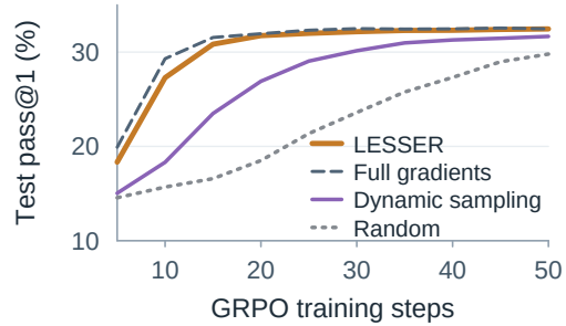
Figure 6: LESSER closely tracks full gradients in RL. Held-out Countdown accuracy over GRPO training steps, averaged over two seeds. Higher is better.
