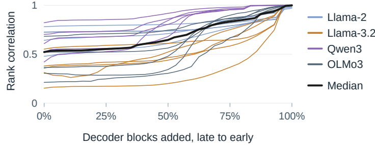
Figure 11: Per-example rankings depend on gradients throughout the network. Spearman correlation with the full-gradient cosine ranking as decoder blocks are added to the output layer from last to first. Candidates are ranked by their cosine with the query gradient over the included parameters. Thin lines denote model–task pairs, colored by model, and the black line shows the median.
