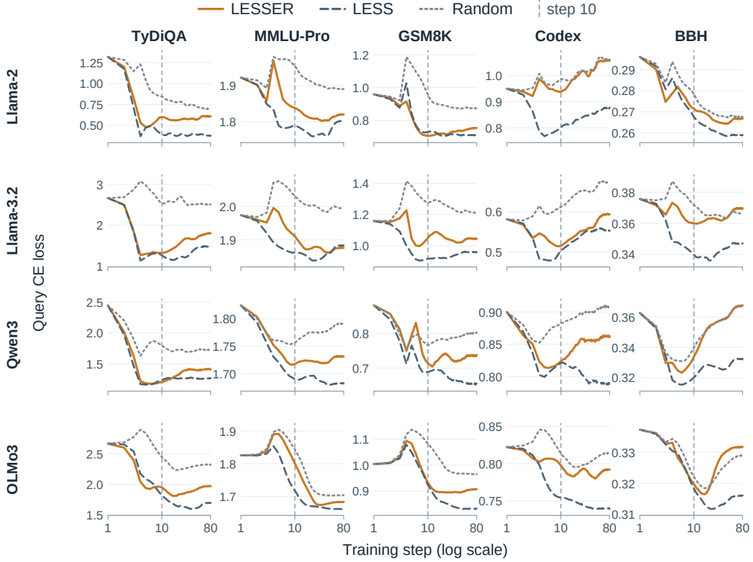
Figure 12: Query loss across training steps. Each panel is one model–task pair.
