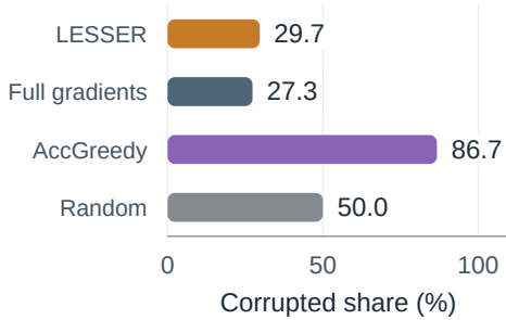
Figure 5: LESSER closely matches full gradients in detecting problems with corrupted rewards. Corruption share among the selected problems. Lower is better.
