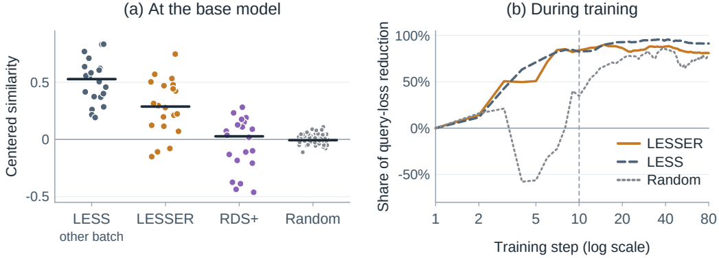
Figure 7: LESSER-selected batches induce gradients aligned with those from LESS. (a) Centered batch-gradient alignment between LESS batches and batches selected by each method, at the base model. Dots denote model-task pairs, and bars show medians. (b) Median share across model-task pairs of the query-loss decrease reached by each training step.
