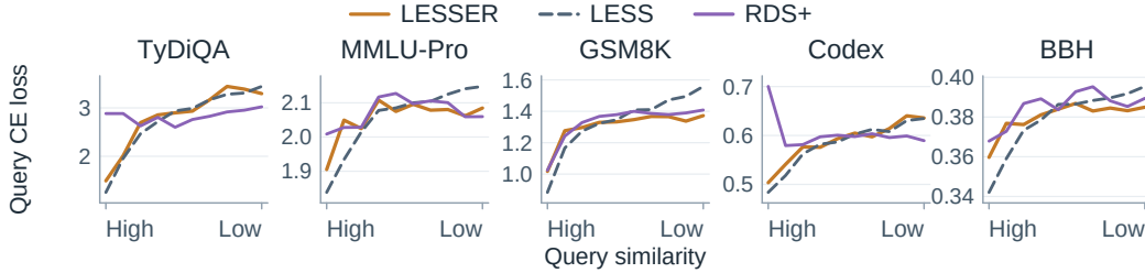
Figure 8: Llama-3.2-3B: query loss across similarity bins. Each bin uses one training run; bin 0 is closest to the queries.
