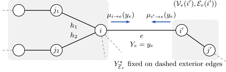
(b) Recursive elimination at i
