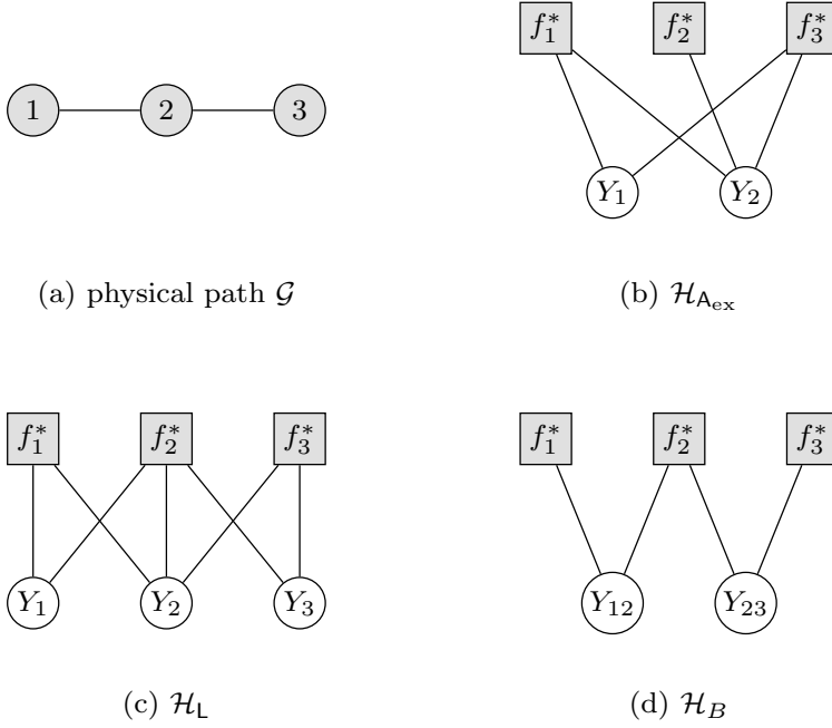
Fig. 1: Three faithful representations (see (1)) of the same path graph 1 - 2 - 3 induce distinct factor graphs: the generic A_{\text{ex}} couples nonadjacent factors, the Laplacian L produces a cyclic factor graph, and the incidence matrix B reproduces the node-edge incidence structure.
