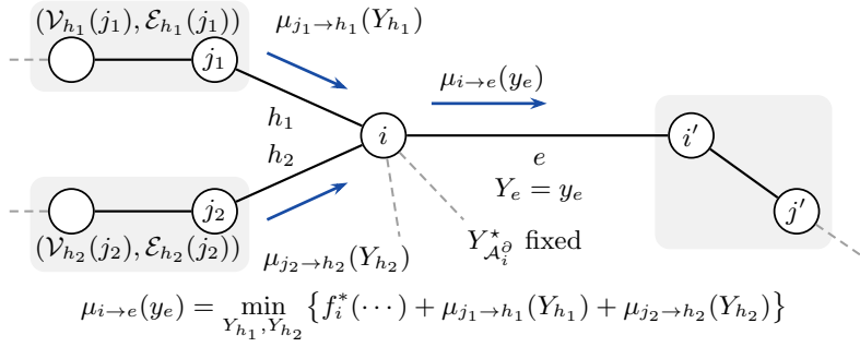
Fig. 3: Messages on the same tree block: (a) fixing Y_e = y_e separates the minimization into two subgraphs; (b) eliminating Y_{h_1}, Y_{h_2} combines the two incoming messages with f_i^* , while the dashed exterior-edge coordinates remain fixed at Y_{\bar{\mathcal{E}}_r}^* .
