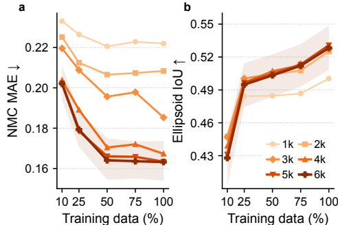
Figure 4: Predictive data scaling on test_struct . NMC MAE (a) and covariance-ellipsoid IoU (b) across 10–100% of the training data and 1k–6k training steps.
