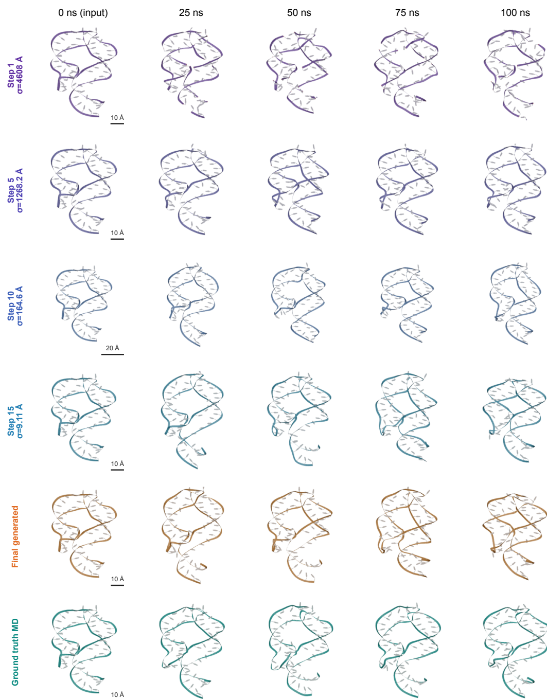
Figure 8: Stepwise denoising of the median-motion held-out RNA 3SKR_A. Columns show 0, 25, 50, 75, and 100 ns. Step rows are diagnostic \hat{x}_0 estimates at the labeled noise scales; the final two rows show the generated trajectory and reference MD. Ribbon gaps mark O3'-P distances of at least 2.6 Å.
