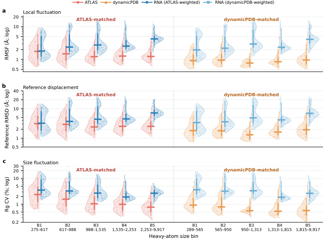
Figure 5: Size-stratified RNA-protein dynamics. Distributions of (a) mean marker-atom RMSF, (b) mean RMSD to the first sampled frame, and (c) heavy-atom R_g coefficient of variation across five size bins. RNA uses C4' markers and protein uses C \alpha ; vertical axes are logarithmic. Split violins show proteins on the left and matched RNAs on the right; bars indicate the median, interquartile range, and 5th–95th percentiles.
