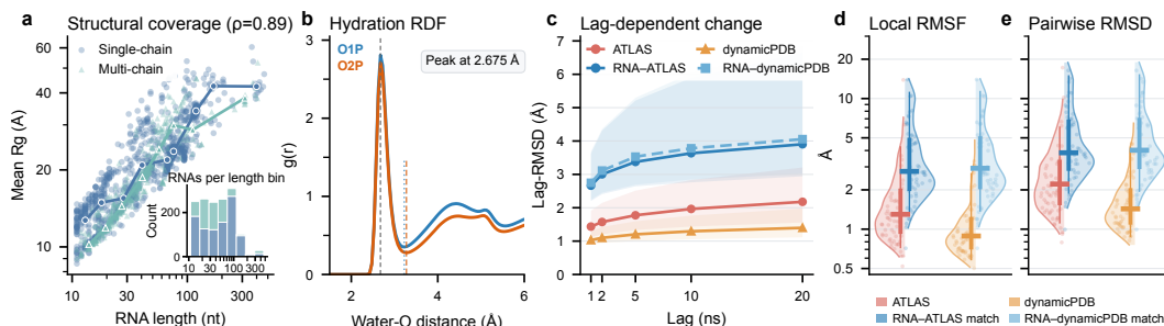
Figure 1: RNADynBench visualized. a , Mean R_g versus RNA residue count. Points show individual RNAs, lines connect length-binned medians, and the inset shows counts; \rho is Spearman correlation between RNA length and mean R_g . b , Median phosphate–water radial distribution functions (RDFs); shading shows the interquartile range, and vertical lines mark the first peak and minima. c , Weighted median lag-RMSD for size-matched RNA–protein comparisons; shading shows the weighted interquartile range (IQR). d,e , Weighted distributions of mean local RMSF ( d ) and median pairwise RMSD ( e ). Split violins show protein left and matched RNA right, with median, IQR, and 5th–95th percentiles. RNA uses C4' atoms and protein uses C \alpha atoms.
