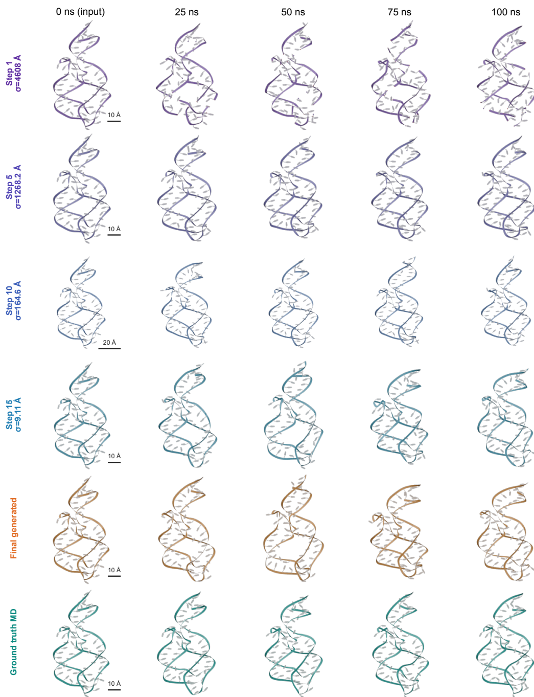
Figure 7: Stepwise denoising of the low-motion held-out RNA 3IVN.A. Columns show 0, 25, 50, 75, and 100 ns. Step rows are diagnostic \hat{\mathbf{x}}_0 estimates at the labeled noise scales; the final two rows show the generated trajectory and reference MD. Ribbon gaps mark O3'–P distances of at least 2.6 Å.
