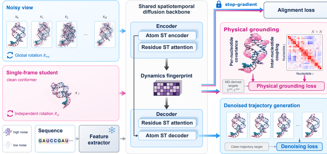
Figure 2: Overview of RNADynNet. RNADynNet jointly learns trajectory generation and single-conformer dynamics representations from MD trajectories. During training, the trajectory view (blue) provides temporal context for denoising and alignment, while the single-conformer view (pink) learns a dynamics representation from one conformer. Physical grounding supervises both views with MD-derived dynamical statistics. At inference, a single conformer supports two modes: the denoising path generates a trajectory, whereas the encoder readout directly yields a dynamics fingerprint. ST denotes spatiotemporal.
