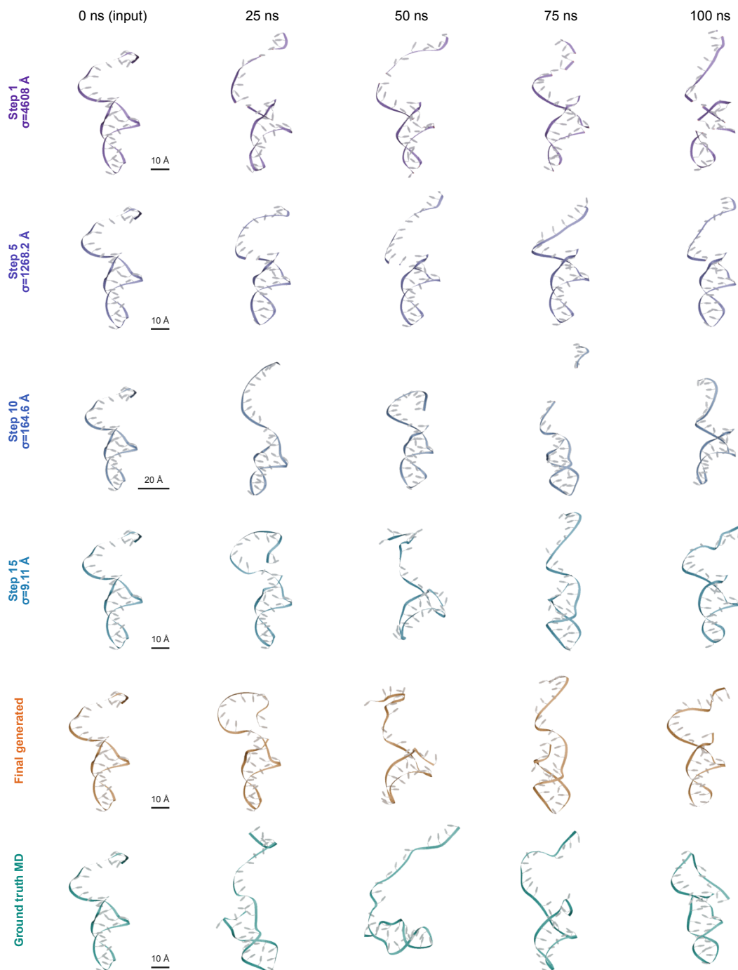
Figure 9: Stepwise denoising of the high-motion held-out RNA 6AZ4 A. Columns show 0, 25, 50, 75, and 100 ns. Step rows are diagnostic \hat{x}_0 estimates at the labeled noise scales; the final two rows show the generated trajectory and reference MD. Ribbon gaps mark O3'-P distances of at least 2.6 Å.
