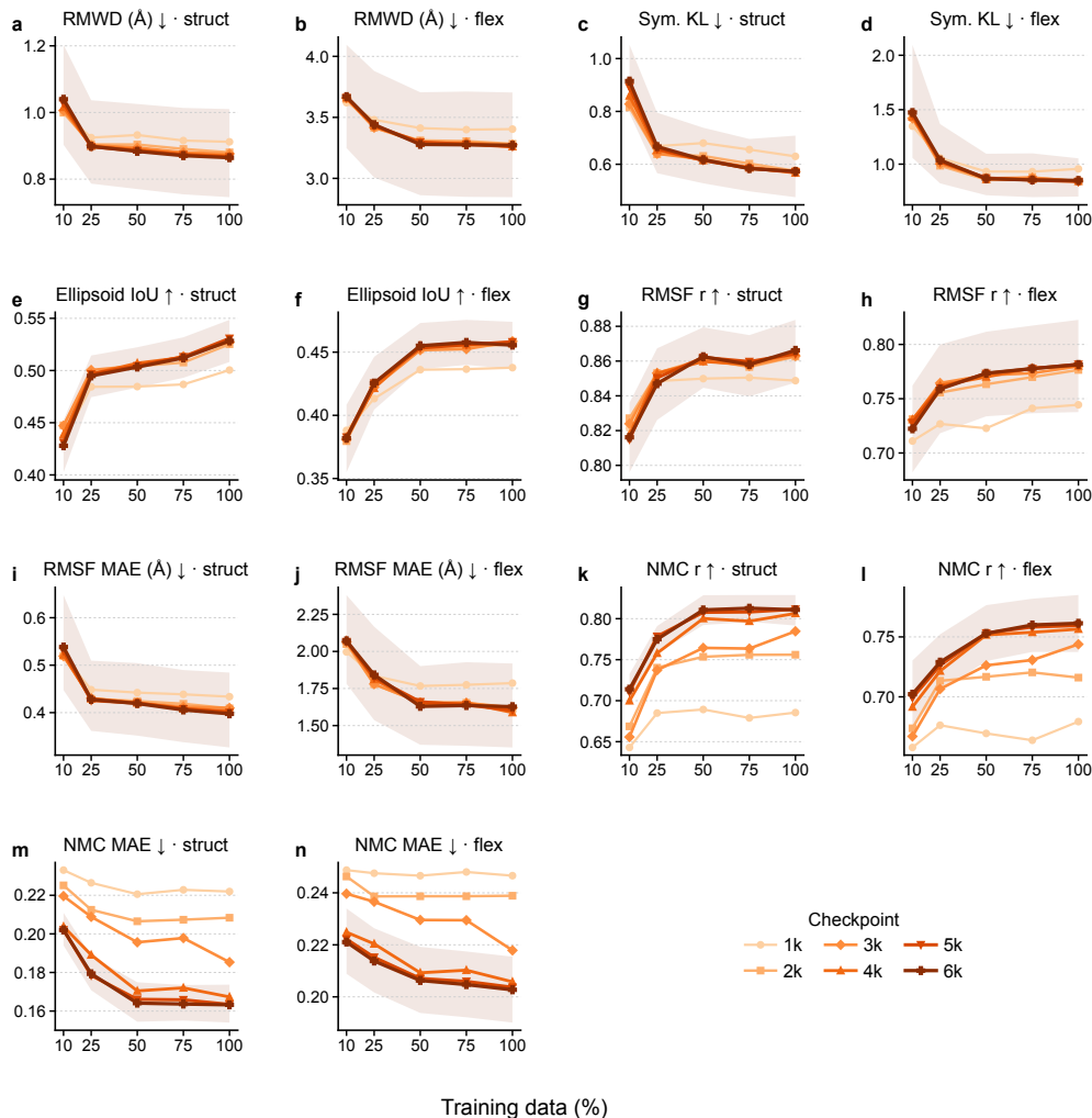
Figure 6: Predictive data scaling. Orange curves darken from 1k to 6k training updates across 10–100% of the training data. Shading shows pointwise 95% source-RNA-group bootstrap intervals for 6k only. Each checkpoint uses its EMA backbone and EMA descriptor heads.
