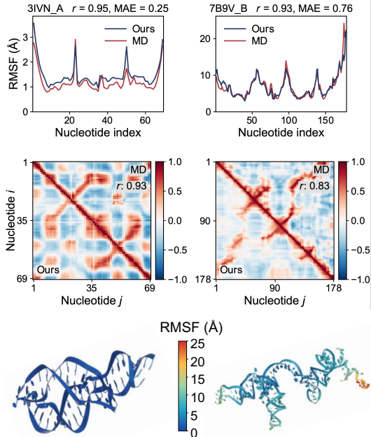
Figure 3: Dynamics inference from single conformers. Predicted per-nucleotide RMSF and pairwise nucleotide motion couplings from RNADynNet are compared with MD references for two RNAs. Motion-coupling matrices show RNADynNet below the diagonal and MD above; structures are colored by RMSF.
