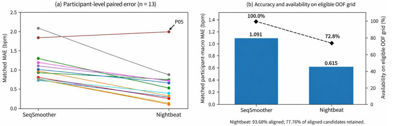
Fig. 3. Participant-level matched error and prediction availability. (a) Paired matched MAE for the 13 independent held-out participants; Nightbeat has lower matched MAE in 12 of 13 participants. (b) Matched participant-macro MAE is shown together with final prediction availability on the 20,792-endpoint SeqSmoother-eligible out-of-fold grid: 100% for SeqSmoother and 72.85% for Nightbeat. Nightbeat aligns to 93.68% of the grid and retains 77.76% of those aligned candidates after quality gating.
