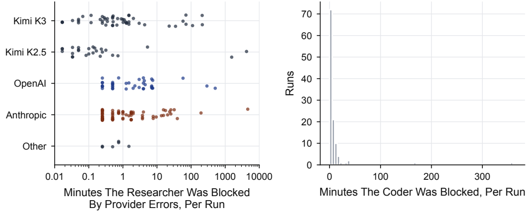
Figure 16: Time lost to model-provider errors in the main experiments. Left: minutes each Researcher was blocked by provider errors (malformed responses, rate limiting, overloads) per run, grouped by provider, on a log scale; one point per run. Right: histogram of minutes the Coder was blocked per run.
