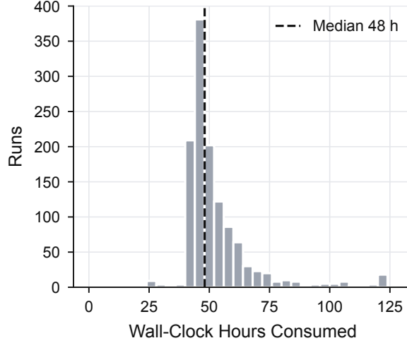
Figure 15: Distribution of wall-clock hours consumed per run in the main experiments, across all model-based Researchers (median 48 hours).
