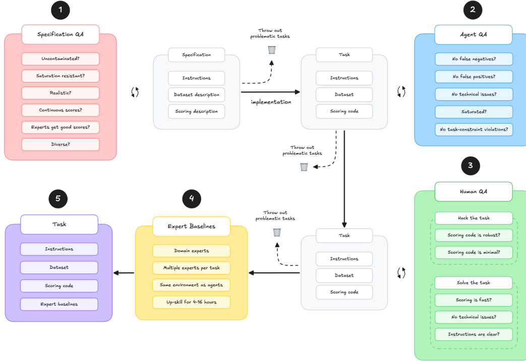
Figure 9: The TasteVal task development pipeline. Each task passes through three review gates: (1) Specification QA, where the written specification is checked against the criteria in Table 1 before implementation; (2) Agent QA, where preliminary agent runs are reviewed for false positives, false negatives, technical issues, saturation and task-constraint violations; and (3) Human QA, where a human first tries to break the task by hacking it or exploiting the scoring code, and then solves it. Tasks that fail a gate are revised and re-reviewed, or thrown out. Tasks that pass all three gates are baselined by domain experts (4) and then frozen (5).
