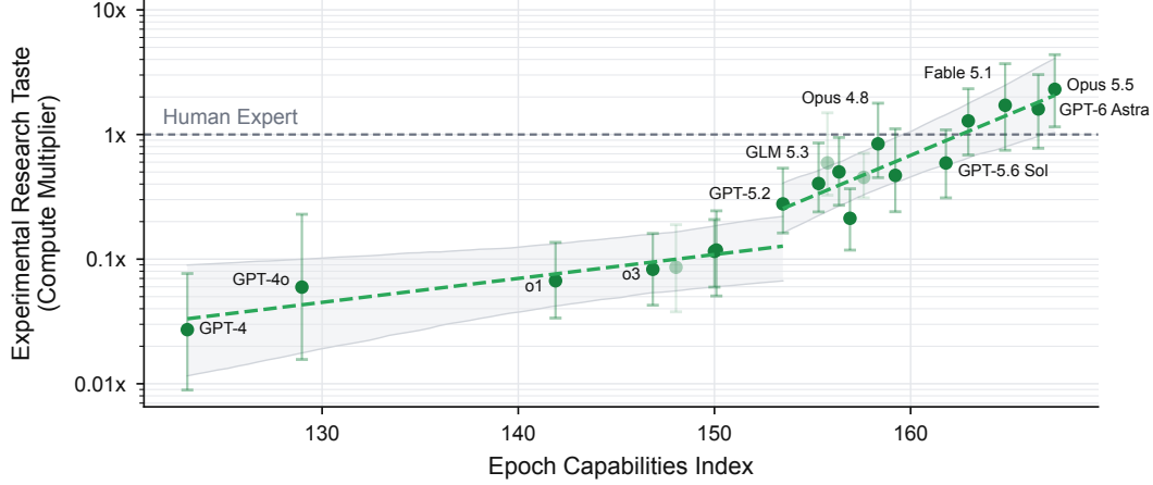
Figure 8: Since GPT-5.2, the compute multiplier doubles every 4.6 ECI units (95% CI 3.1–8.8). Each model’s compute multiplier from Figure 1 is plotted against its Epoch Capabilities Index score [Epoch AI, 2026], a measure of general capability, with separate log-linear fits before and after the break at GPT-5.2 ( R^2 = 0.95 ). Colors, error bars and shaded regions as in Figure 1.
