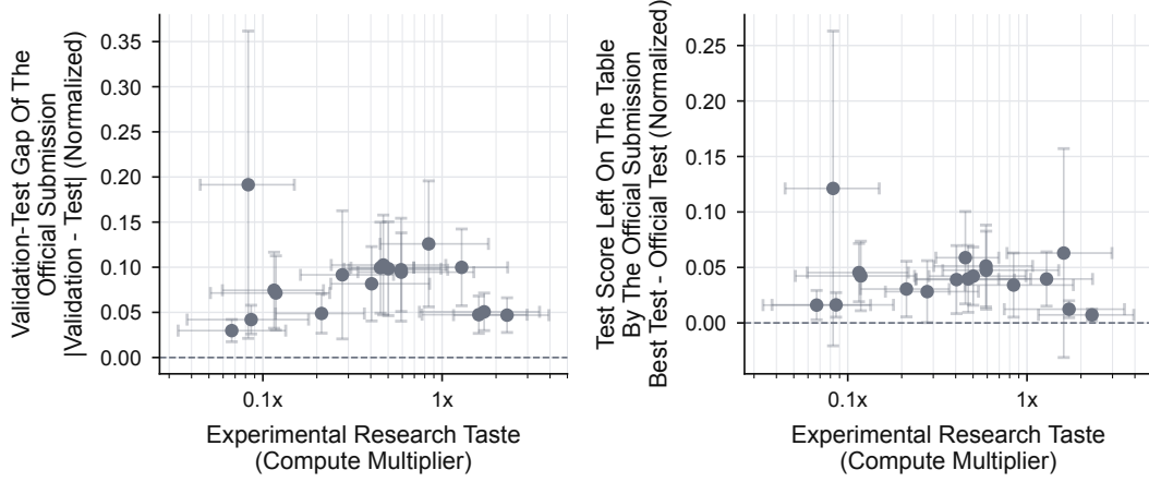
Figure 20: Two measures of official-submission quality against the compute multiplier; one point per model, means with 95% CIs. Left: absolute generalization gap of the official submission, |\text{validation score} - \text{test score}| . Right: regret of the official submission (the best test score among the run’s submissions minus the official submission’s test score; zero when the Researcher chose its best submission). Both are in normalized units (naive baseline 0, expert baseline 1). Only runs in which the Researcher marked an official submission are included; models with fewer than 30 such runs are omitted.
