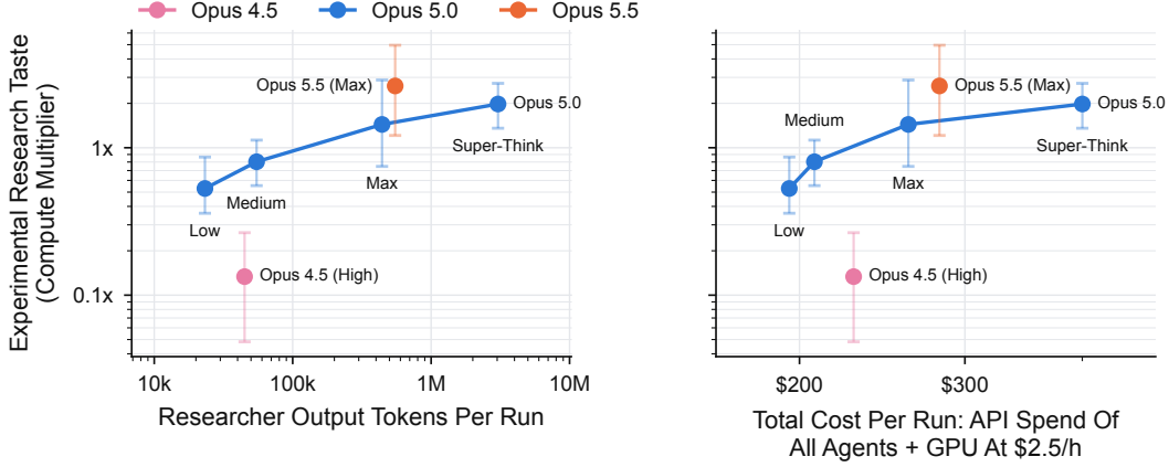
Figure 6: Opus 5.0’s compute multiplier rises with Researcher inference compute. We evaluate Opus 5.0 at low, medium and max reasoning effort, and at max reasoning in our ReAct-Super-Think scaffold. We only use 6 tasks across all models for this analysis. Error bars are 95% intervals from a two-level hierarchical bootstrap with 1,000 resamples, drawing first over tasks and then over runs within each task. Left: compute multiplier against Researcher output tokens per run (arithmetic mean over runs). Right: the same against total API and compute spend per run, including the spend across Researcher, Coder, Liaison and monitors. Opus 5.5 (max) and Opus 4.5 (high) in the standard scaffold are shown for reference.
