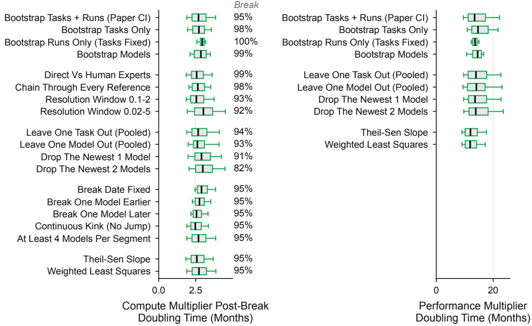
Figure 12: Post-break doubling time of the compute multiplier (left) and doubling time of the performance multiplier’s single trend (right), over 1,000 draws per perturbation. For the compute multiplier the break date is re-chosen in each draw unless the row fixes it, and the column beside the left panel is the share of draws whose peak Chow F exceeds the 5% critical value. Boxes span the 25th–75th percentiles, whiskers the 10th–90th. Reference rows read every model directly against the expert baseline, chain through every model, or change the window (0.1–2x, 0.02–5x) in which a reference is trusted; the continuous-kink row fits one line whose slope changes at the break.
