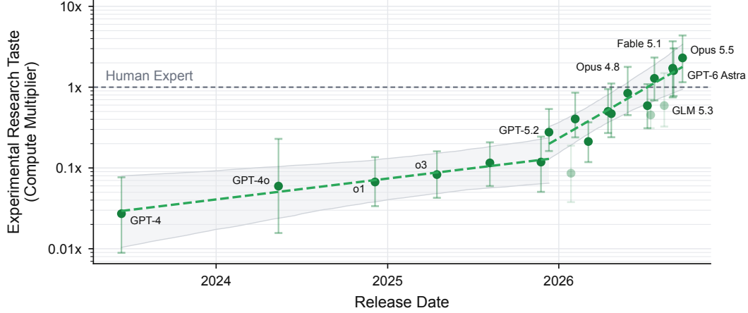
Figure 1: The compute multiplier of models has doubled every 3.0 months (95% CI 1.7–5.0 months) since December 2025, up from every 14.0 months before. Each point is one model’s compute multiplier relative to our expert baseline (1x), plotted against its release date. At-the-time frontier models are shown in dark green and used for the fits; non-frontier models are shown in light green. The dashed lines are separate log-linear fits before and after the break at the release of GPT-5.2 ( R^2 = 0.96 ), and the shaded regions their 95% bands. Error bars are 95% intervals from a two-level hierarchical bootstrap with 1,000 resamples, drawing first over tasks and then over runs within each task.
