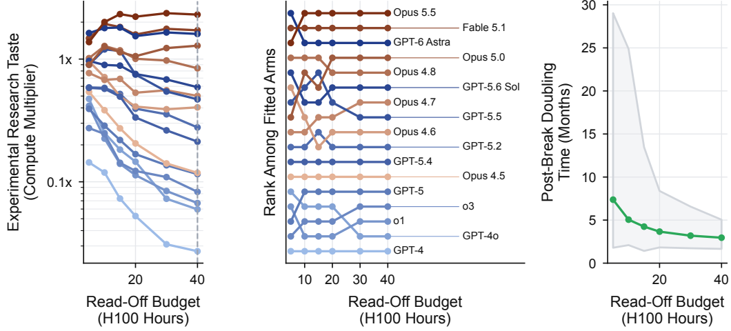
Figure 13: Truncating runs before the full 40-hour budget leaves the model ranking and frontier models’ multipliers nearly unchanged, but lengthens the post-break doubling time as the budget shrinks. We truncate every run and every reference at B GPU hours, for B from 5 to 40, keep only submissions scored by then, rebuild the reference envelopes and recompute the chain exactly as in the main text. Left: each model’s compute multiplier as a function of the read-off budget. Middle: each model’s rank among the fitted models. Right: the post-break doubling time with its 95% CI, the break date re-chosen at every budget and in every bootstrap draw.
