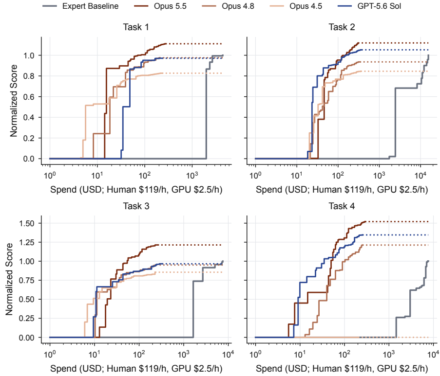
Figure 18: As Figure 17, but against total Researcher expenditure in USD on a log scale: API spend for models, salary for humans at $119/h, plus GPU time at $2.5/h for both.
