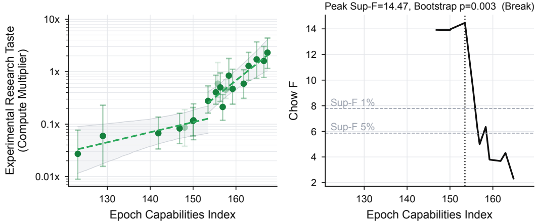
Figure 11: Against general capability, the compute multiplier’s trend also changed at GPT-5.2. Left: each frontier model’s compute multiplier against its Epoch Capabilities Index score, with separate log-linear fits before and after the break (non-frontier models faded and not fitted). The multiplier doubled every 15.7 ECI units before the break and every 4.6 ECI units (95% CI 3.1–8.8 units) after it. Right: the Chow F-statistic for a break at each model’s ECI score. Error bars and shaded regions as in Figure 10.
