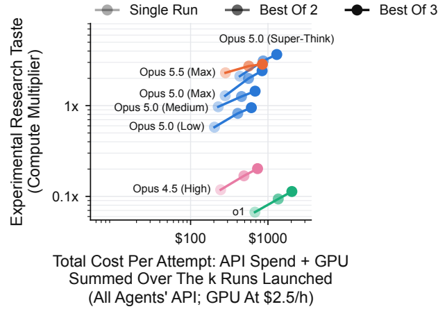
Figure 21: Best-of- k scaling of the compute multiplier against total cost. We compare models across 6 tasks. For each arm, k runs are launched and the one with the best validation score is kept; points show the expected test multiplier for k = 1, 2 and 3. Cost is summed over all k runs: API spend for all agents plus GPU time.
