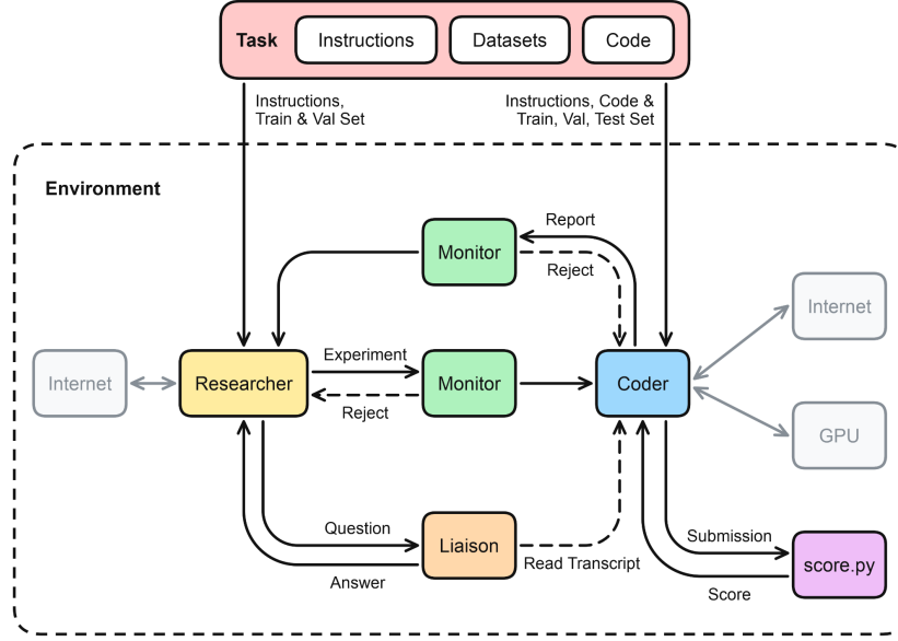
Figure 2: An overview of TasteVal. Each task consists of instructions, datasets, and scoring code. The Researcher, the model under evaluation, sees the instructions and the train and validation sets, and decides which experiments to run; the Coder, fixed across all runs, additionally sees the test set and scoring code, implements each experiment on a single H100, and reports back the results. Two Monitors enforce the Coder-Researcher contract, one in each direction, and the Liaison answers the Researcher’s questions about the Coder’s progress by reading its transcript.
