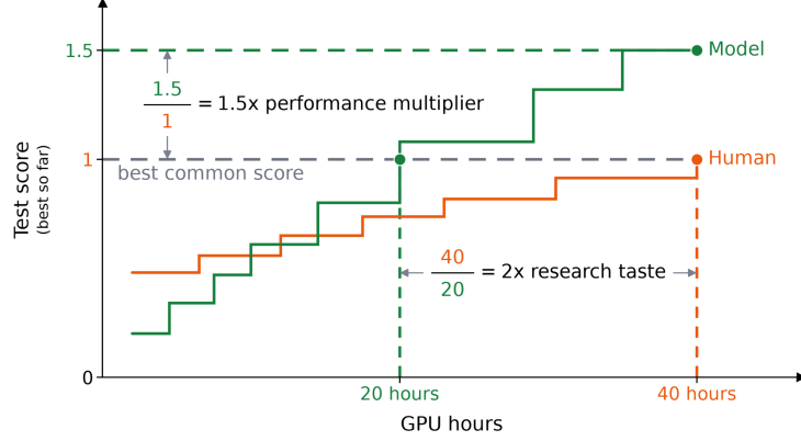
Figure 3: Computing the compute multiplier and the performance multiplier for a single run. Each curve shows the normalized score (naive baseline 0, expert baseline 1) of the run’s selected submission as a function of GPU hours spent: its best on validation so far, until it produces the submission it will mark official. Because two runs rarely end at the same score, we compare them at the weaker run’s endpoint score (here the human’s). The stronger run’s compute is the GPU hours at which it first reached that score (20 hours for the model), and the weaker run’s compute is its whole budget (40 hours). This gives a compute multiplier of 40/20 = 2x : the model reached the expert’s final score with half the compute. The performance multiplier is the ratio of the runs’ final normalized scores, regardless of compute: the model ends at 1.5 and the expert at 1, so the model’s performance multiplier is 1.5x .
