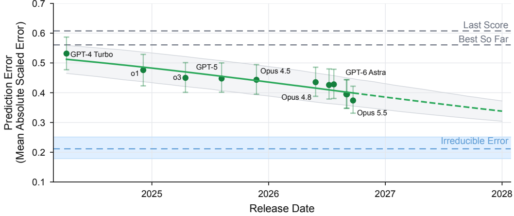
Figure 7: Mean absolute scaled error of each model’s predictions of the validation score of 1,173 experiments drawn from 120 main-experiment runs, given the task, the experiment description, and the run’s earlier experiments and their scores. Dashed and dotted gray lines show two naive baselines, predicting the run’s last score (0.608) or its best score so far (0.561). The blue dotted line is a lower bound on the irreducible error (0.211), estimated by re-executing 24 experiments 9 times each with fresh training seeds and re-scoring the results. The blue band is its 95% CI. We fit a sigmoid that falls from the last-score baseline to the irreducible error ( R^2 = 0.85 ), and the dashed green line extrapolates the trend. Error bars and the shaded band are 95% intervals from a bootstrap over runs within each task, with the four tasks held fixed.
