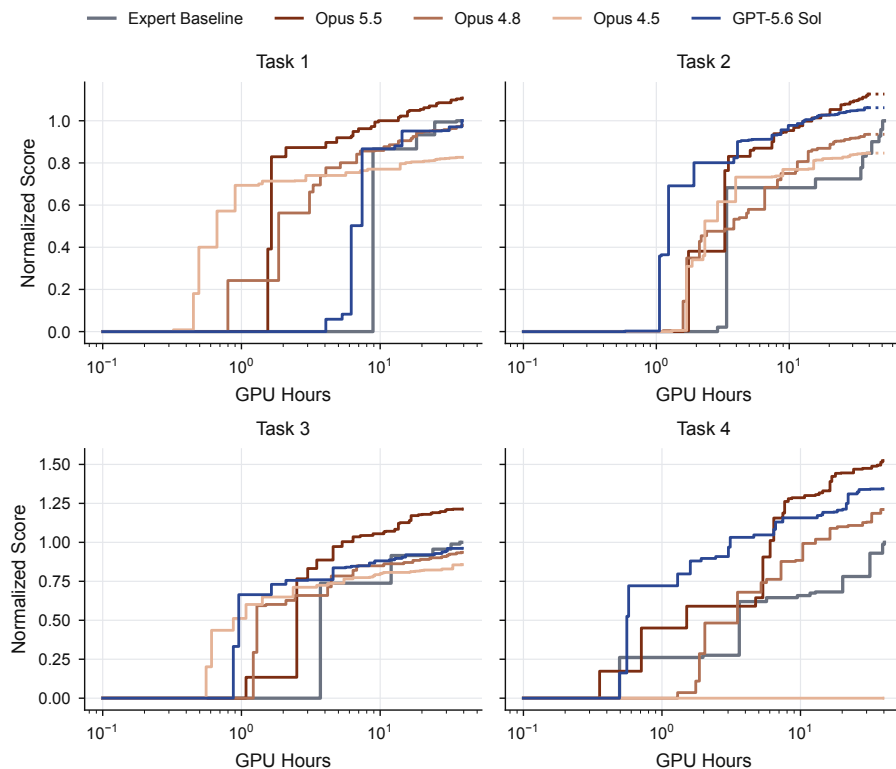
Figure 17: Score trajectories on four tasks against GPU hours. Each panel shows the best normalized test score so far (naive baseline 0, expert baseline 1) as a function of GPU hours spent, for Opus 5.5, Opus 4.8, Opus 4.5 and GPT-5.6 Sol, alongside the best human. Model curves are the median across all 6 seeds; the human curve is the best per task attempt.
