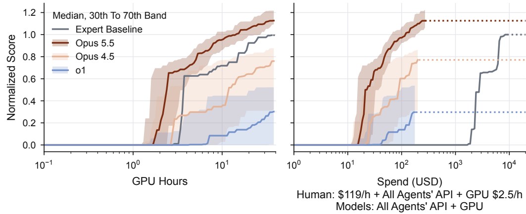
Figure 19: Normalized score against GPU hours (left) and total expenditure (right), pooled across all tasks. Lines are medians and bands span the 30th to 70th percentiles across runs, for Opus 5.5, Opus 4.5, o1 and the human baseliners; the black line is the expert baseline, the best human attempt per task.
