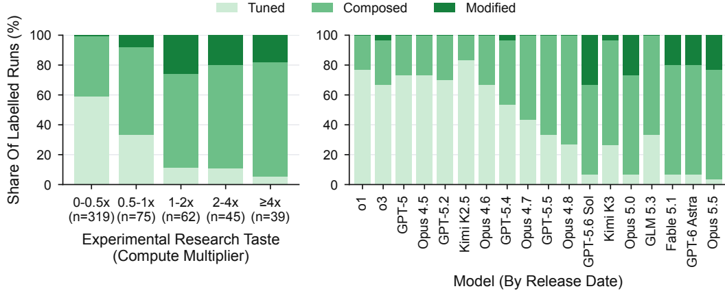
Figure 5: We label 540 official submissions from our main experiments as Tuned, Composed, Modified, or Invented; none met the bar for Invented. Left: share of each class, bucketed by the run’s compute multiplier ( n is the number of labeled runs per bucket). Right: share of each class for each of the 18 models, ordered by release date (30 labeled runs per model).
