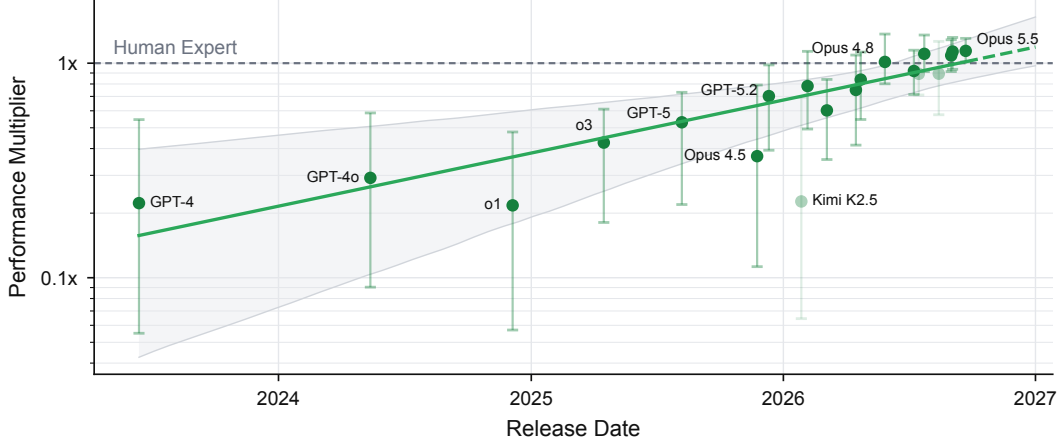
Figure 4: The performance multiplier has been doubling every 14.6 months (95% CI 8.4–29.8 months). Each point is one model’s performance multiplier, the official submission’s test score reached within the full 40 GPU-hour budget rescaled so that the naive baseline is 0 and the expert baseline is 1, plotted against release date ( R^2 = 0.83 on the log-linear fit). Colors and error bars as in Figure 1; the shaded region is the 95% band of the fit.
