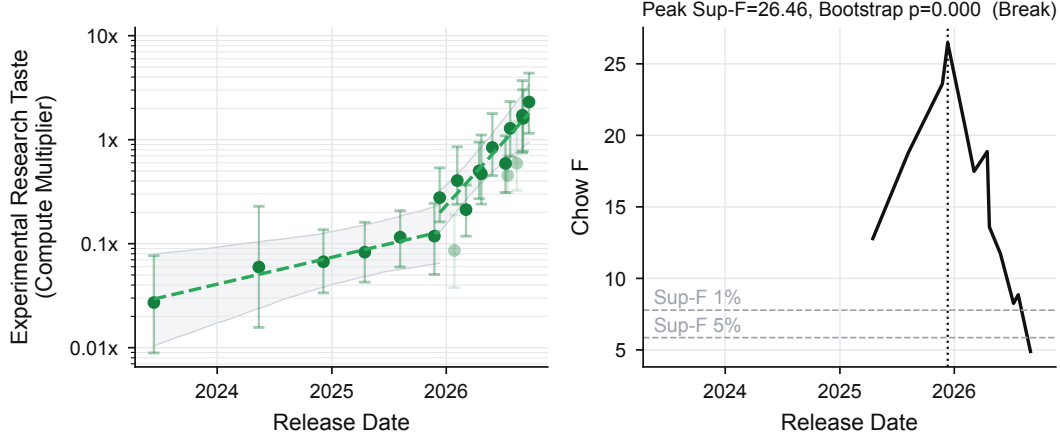
Figure 10: The compute multiplier’s trend changed in December 2025. Left: each frontier model’s compute multiplier against its release date, with separate log-linear fits before and after the break (non-frontier models faded and not fitted). The multiplier doubled every 14.0 months before the break and every 3.0 months (95% CI 1.7–5.0 months) after it. Right: the Chow F-statistic for a break at each model’s release date. Error bars are 95% intervals from the two-level hierarchical bootstrap of Figure 1. Shaded regions are the 95% band of each segment’s fit across bootstrap draws with the break date held at its point estimate; the interval on the post-break doubling time re-chooses the break date in each draw.
