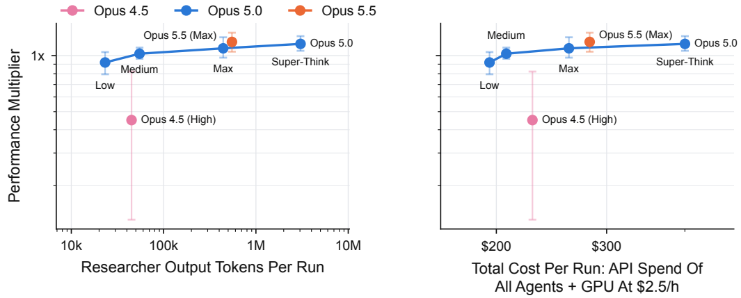
Figure 22: As Figure 6, for the performance multiplier. Error bars are 95% intervals from a two-level hierarchical bootstrap with 1,000 resamples, drawing first over tasks and then over runs within each task. Left: performance multiplier against Researcher output tokens per run (arithmetic mean). Right: the same against total API and compute spend per run, including the spend across Researcher, Coder, Liaison and monitors.
