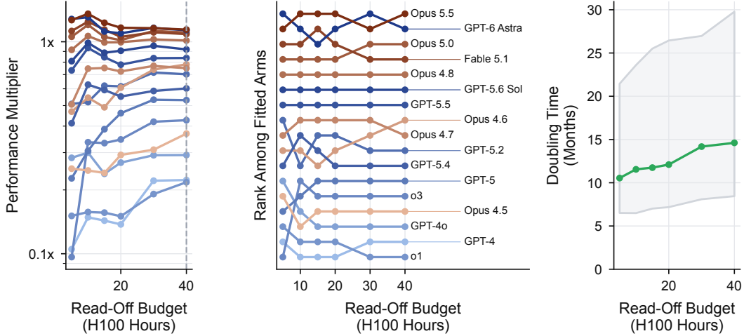
Figure 14: As Figure 13, for the performance multiplier; the right panel shows the doubling time of its single log-linear trend, which has no significant break.
