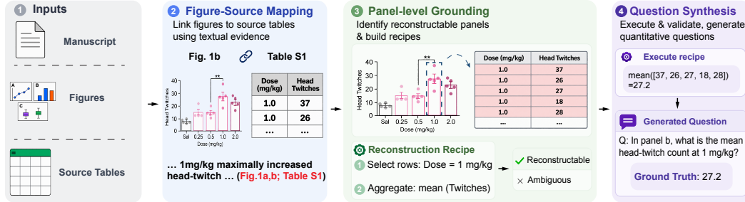
Figure 1: Overview of the PlotGround pipeline. Given a bioRxiv paper organized as a filesystem (manuscript, figures, and supplementary source tables), Mapping proposes candidate figure–table bindings from textual evidence such as captions and in-text references; Grounding retains only panels whose values can be reliably reconstructed and records a reconstruction recipe, rejecting ambiguous ones; Synthesis follows the recipe, validates the recomputed values, and writes questions using only figure-visible labels. For clarity, the example shows a single panel with question text abbreviated. Real figures are typically multi-panel and are given to models in full (Appendix A.2).
