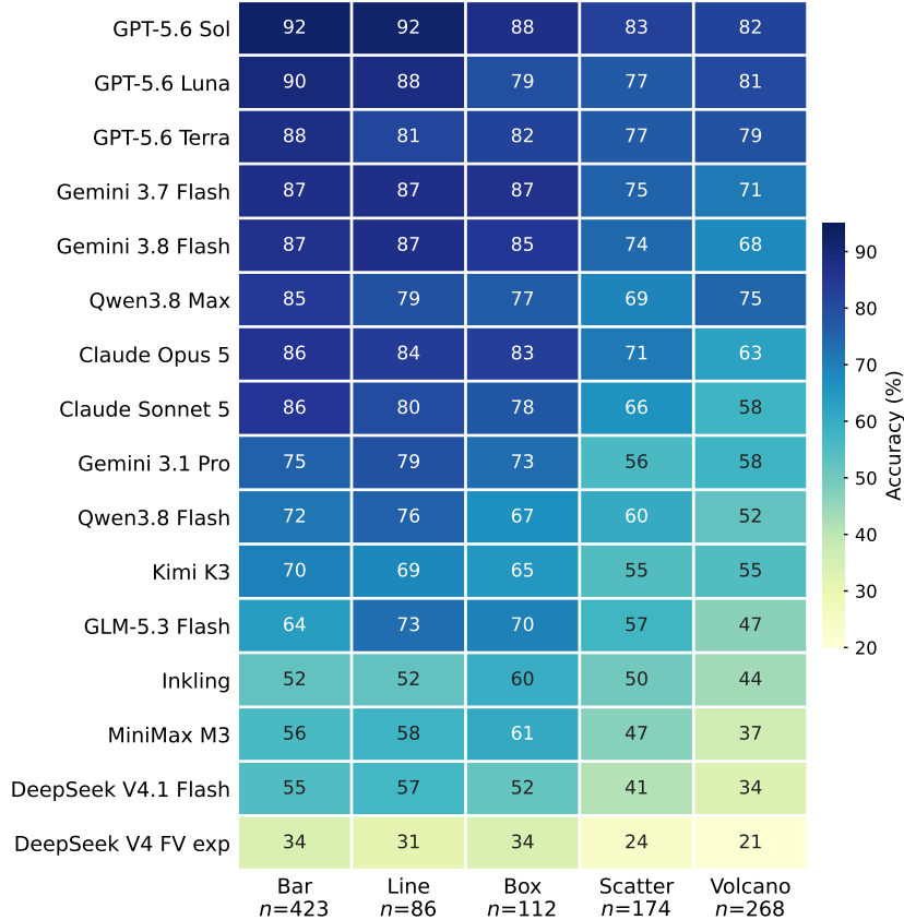
Figure 5: Accuracy by chart type. Per-model accuracy at a \pm 5\% relative tolerance for the models in Table 2. Columns show the five most common chart types, ordered by mean accuracy across models. Among these five types, either scatter or volcano plots yield the lowest accuracy for each of the 16 models. This may reflect the difficulty of locating a labelled target point among many others.
