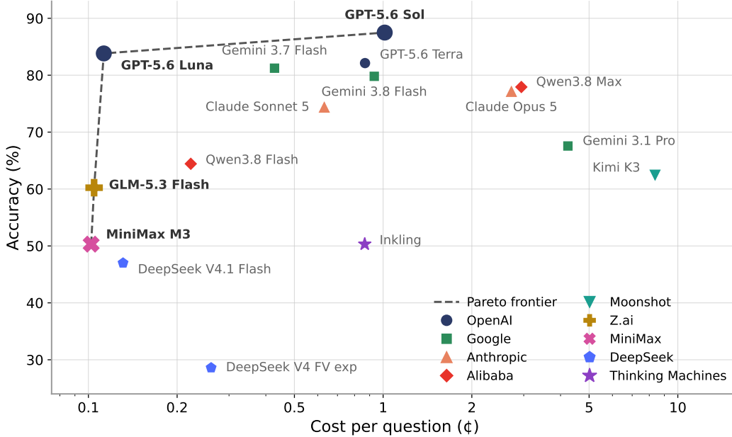
Figure 2: Accuracy versus inference cost on PlotGround-1k. Each point represents a model, with colors and marker shapes indicating developers. Accuracy is measured at a \pm 5\% tolerance, and mean inference cost per question is shown in cents on a logarithmic scale. The dashed line connects Pareto-optimal models, whose labels are shown in bold. Higher cost does not necessarily yield higher accuracy: GPT-5.6 Luna achieves 83.8% accuracy at 0.11 cents per question, compared with 62.5% at 8.37 cents for Kimi K3.
