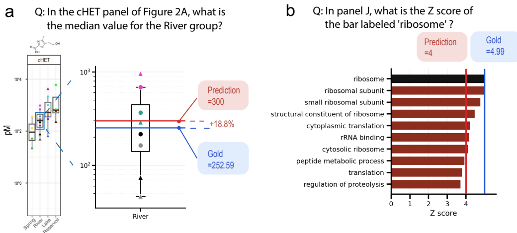
Figure 3: Representative qualitative failure cases. (a) On a log axis, a visually small discrepancy in position can correspond to a substantial numerical error; the model predicts 300 for a gold value of 252.59. (b) Models often snap predictions to labeled tick marks, failing to account for the target’s position between or beyond ticks. For a bar with gold value 4.99, eight of sixteen models predict the final labeled tick at 4.
