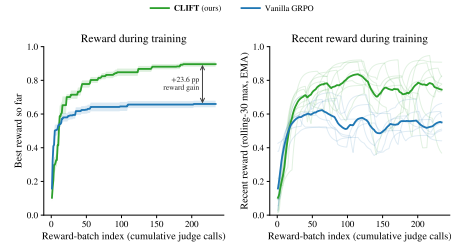
Figure 3: WAI training reward. CLIFT separates from vanilla GRPO under the same judge and browser-use stack.
