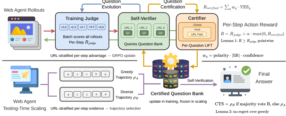
Figure 2: CLIFT overview. Training: rollouts are scored by a comparative judge and by a self-verifier that queries a polarity-tagged question bank. The CCC certifies question weights by URL tier, yielding a signed verifier score that is asymmetrically added to the judge reward and then converted into URL-stratified token advantages. Test-time scaling: the trained agent emits a greedy rollout and diverse retries; the frozen certified bank produces per-URL evidence for each pairwise comparison, and a conservative repeated-vote rule decides whether to keep the incumbent or swap.
