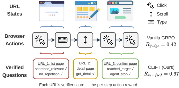
Figure 1: CLIFT concept. Vanilla GRPO broadcasts one trajectory-scalar reward; CLIFT scores each visited URL with verification questions and inherits the URL score to actions taken there. Full pipeline: Figure 2.
