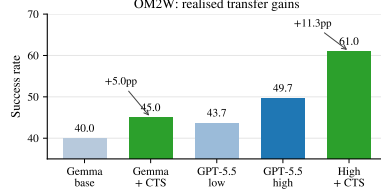
Figure 5: OM2W transfer gains. Realised SR; K is rollout budget.
