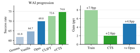
Figure 4: WAI progression and gains. Operating points and deltas.
