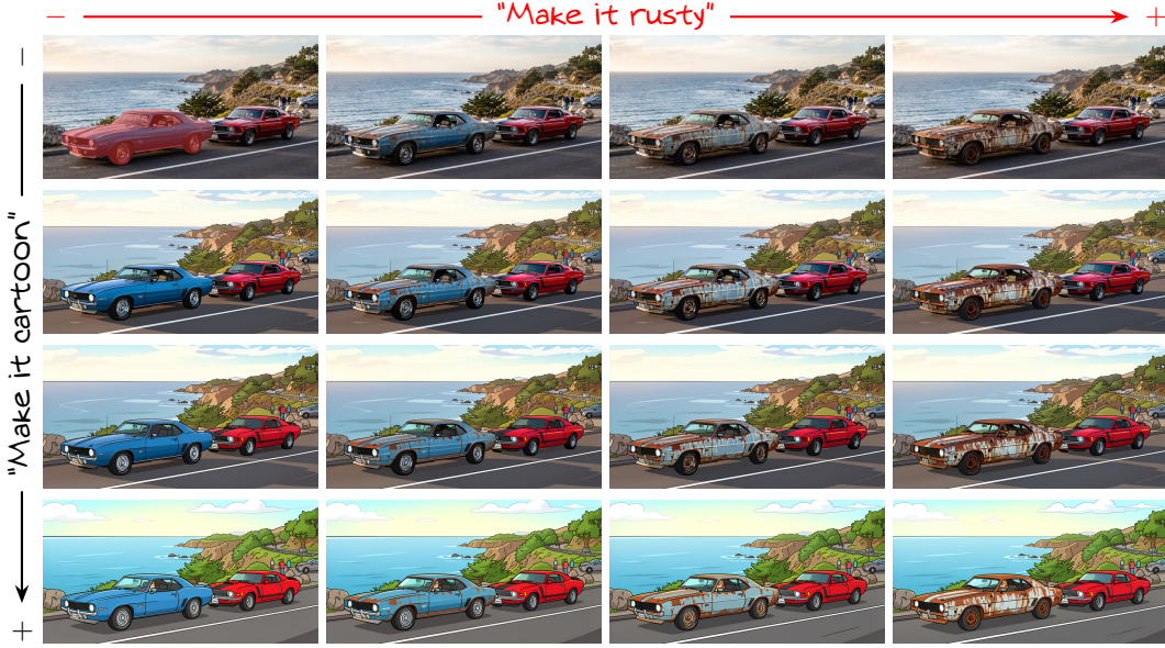
Figure 6: Composing a masked edit with a global one. A 4 \times 4 grid over two instructions applied to the same input. Strength increases left to right and top to bottom. The second axis is obtained by re-running UniSlider on the output of the first, no composed or masked examples appear in training.
