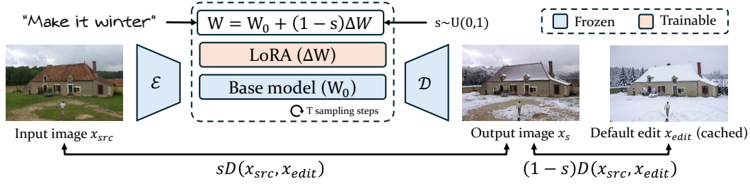
Figure 3: UniSlider training scheme. We sample s , scale the trainable LoRA against the frozen backbone (Eq. (3)), and run the full T -step inference process to get x_s ; x_{\text{edit}} is cached once at s=1 . The loss (Eq. (4)) pushes x_s to the s -implied perceptual position along the path from x_{\text{src}} to x_{\text{edit}} .
