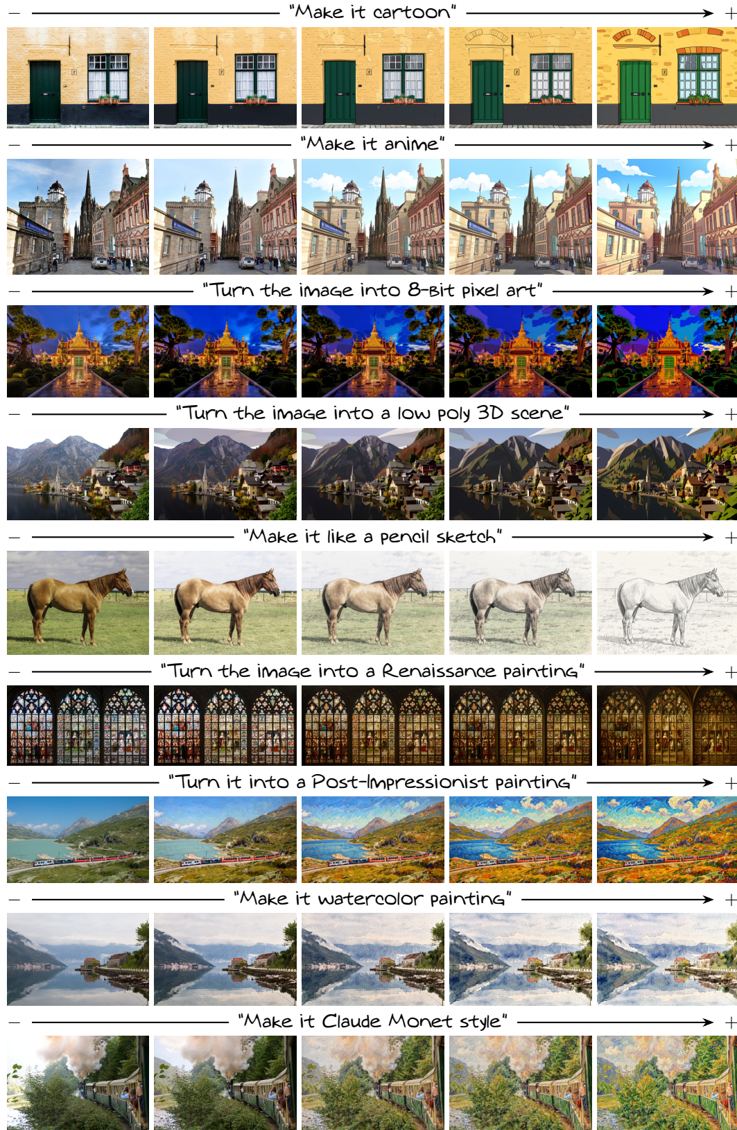
Figure 13: Additional UniSlider results with changes in visual style. From left to right input image, all the intermediate strength levels and the default output of Flux-Klein-4B. All the input images are from the DIV2K (Agustsson & Timofte, 2017) dataset.
