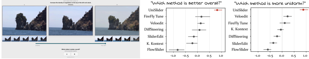
Figure 10: Benchmark 2AFC user study. Left: a screenshot of the study interface, in which annotators drag a slider back and forth to compare methods A and B at matching strengths. Right: Thurstone Case V values with confidence intervals from the pairwise judgments, for the two questions asked: which method is better overall, and which is more uniform. A total of 25 observers participated in the study making a total of 881 examples.
