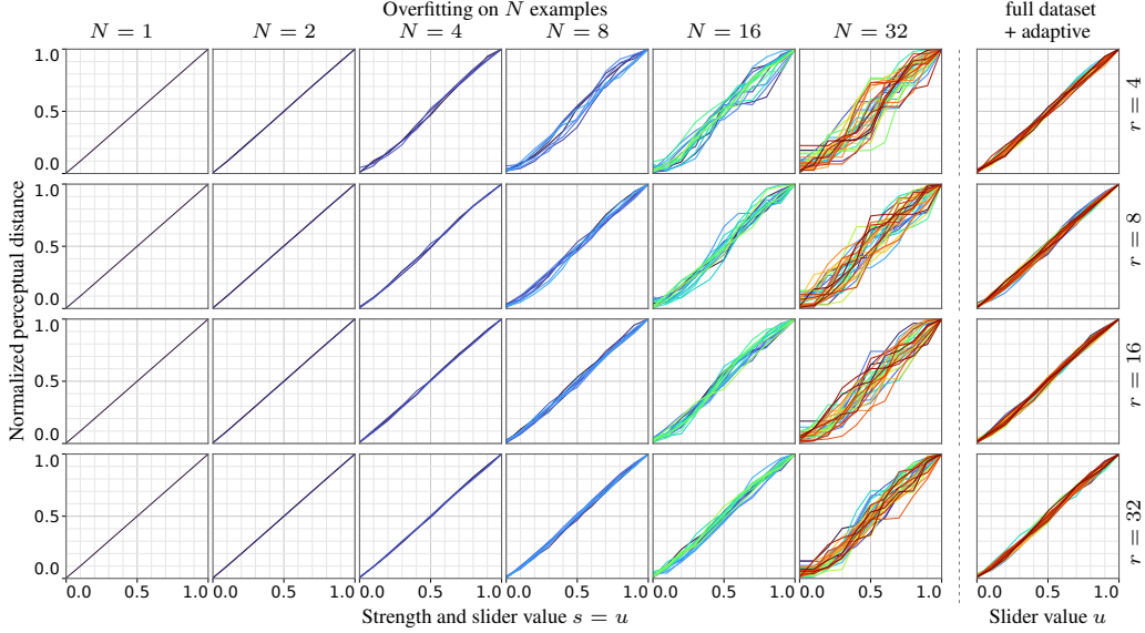
Figure 4: Uniformity degrades with the number of training examples, and is recovered by adaptive sampling. Normalized DreamSim distance from the input to the output, for adapter rank r and N overfitting examples. The diagonal is the ideal uniform slider. First six columns: the strength is the slider ( s = u ). Rightmost column (full method): one adapter trained on the full dataset, evaluated on N = 32 unseen examples, with adaptive sampling mapping u to u = g(s) .
