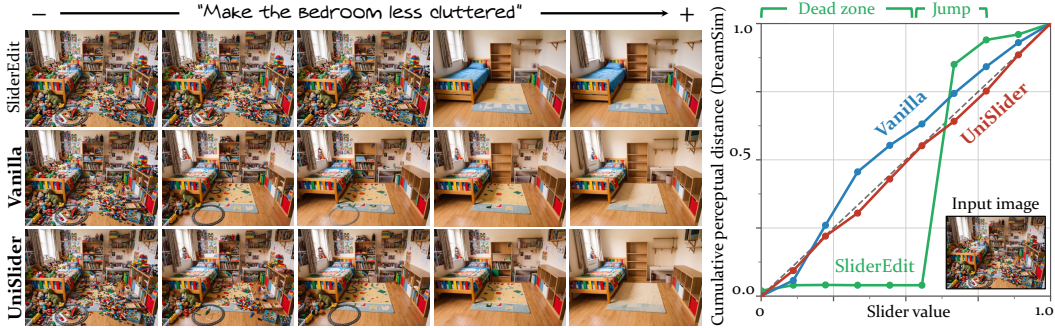
Figure 2: Training closes most of the gap to a uniform slider; adaptive sampling closes the rest. All three rows edit the same image with the same instruction. Left: frames at equal slider values for SliderEdit, our loss alone ( Vanilla ), and our full UniSlider method with strength reparametrization. Right: perceptual distance from the input to every slider frame, normalized by the total input–edit distance. The diagonal marks a perfectly uniform slider. We use DreamSim (Fu et al., 2023) as a perceptual metric.
