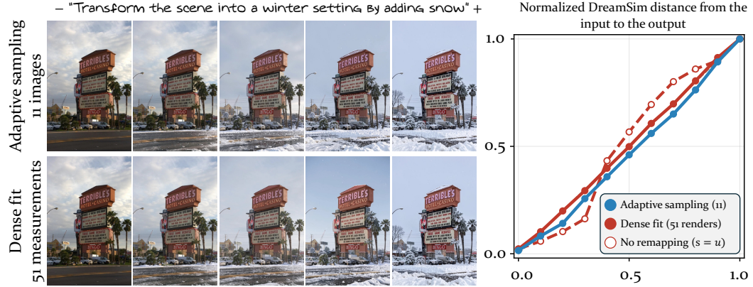
Figure 8: Adaptive sampling vs. dense reference. Left: five of the eleven frames obtained with adaptive sampling (top) and with the dense reference, which inverts a PCHIP spline fitted to 51 measurements (bottom). Right: normalized DreamSim distance from the input to each frame against the slider value u . Without remapping (dashed), adaptive sampling (blue) and dense fit (red).
