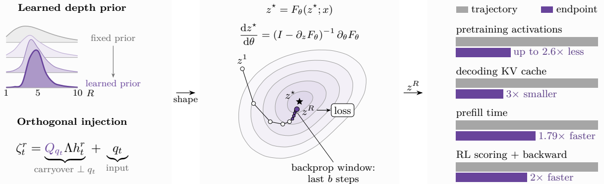
Figure 1: What shapes fixed points, and what fixed points enable. Near a fixed point, the recurrence trajectory can be skipped: training backpropagates through only the last b steps, decoding keeps terminal KV banks, a student distills prefill, and RL reuses saved states to score and update (Section 3). The depth prior and input injection shape the fixed points; we learn the prior from prediction feedback and project the carryover off the input (Section 4).
