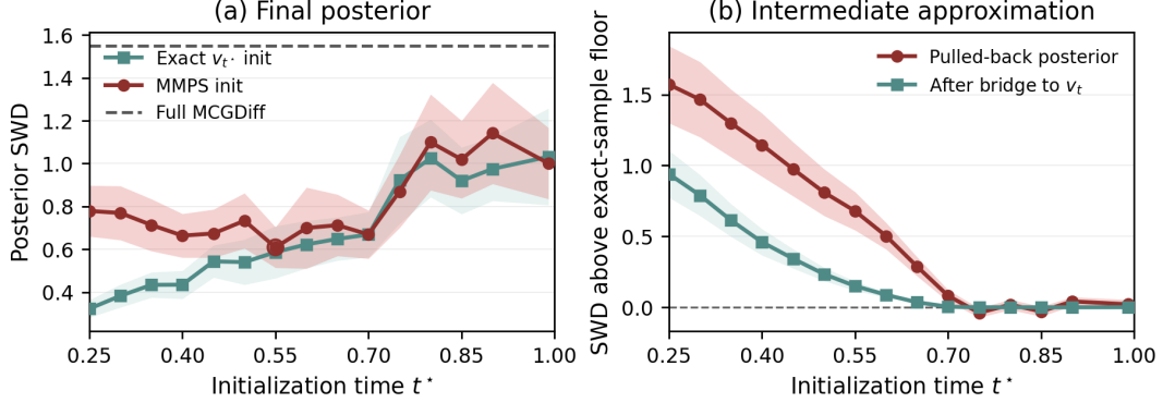
Figure 1: Effect of initialization time t^* on the standard GMM benchmark. (a) Final posterior SWD for oracle and MMPS initialization. (b) MMPS approximation error before and after the exact bridge to v_{t^*} . Generated with 1000 MMPS denoising steps and averaged over 80 seeds.
