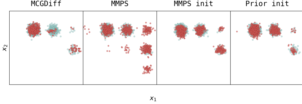
Figure 2: Posterior samples on the standard GMM benchmark for MCGDiff, direct MMPS, MMPS initialization, and prior initialization. MMPS and Prior initialization give qualitatively comparable samples on this relatively simple benchmark. Teal: exact posterior samples; Red: approximate method samples.
