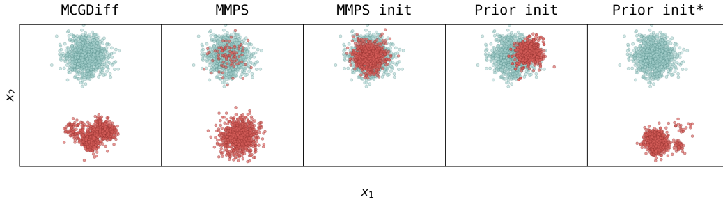
Figure 3: Posterior samples on the rare-mode GMM benchmark for MCGDiff, direct MMPS, MMPS initialization, and two separate prior initialization examples. Unless marked otherwise, initialized methods use t^* = 0.3 and ESS-thresholded resampling at 0.7N . Prior initialization* instead uses t^* = 0.4 with resampling at every step. This variant illustrates a failure mode of prior-based initialization: it collapses to the wrong posterior mode, whereas the ESS-thresholded prior initialization recovers the correct mode but remains less accurate than MMPS initialization. Teal: exact posterior samples; Red: approximate method samples.
