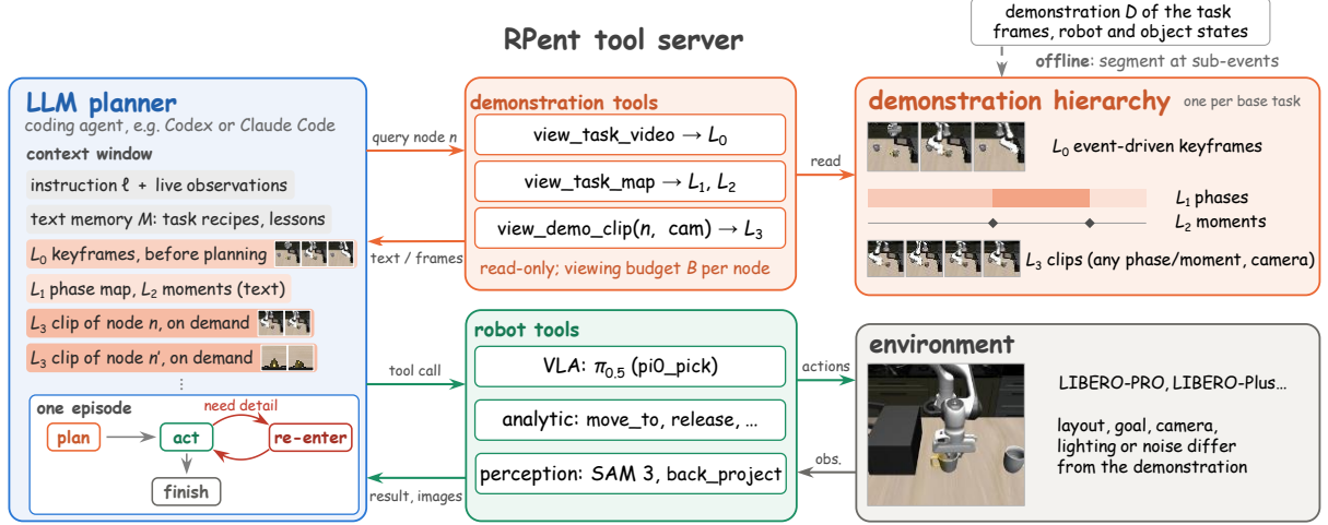
Figure 2: Architecture of RV-ICL on RPent . Each demonstration is segmented offline at its sub-events into a four-level hierarchy. During an episode the LLM agent acts through the harness. Robot tools execute on the environment, and read-only demonstration tools load a level of the hierarchy into the agent’s context. The agent reads the coarse levels ( L_0 – L_2 ) before planning and loads a clip whenever its current sub-goal needs more detail.
