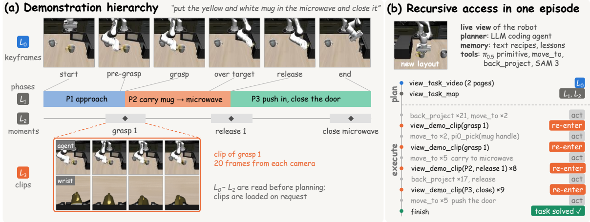
Figure 1: Overview of RV-ICL on a task from the LIBERO-10 suite of LIBERO-PRO. The agent receives one demonstration of the task as a hierarchy (a) and consults it while solving the same task in a new layout (b). (a) The hierarchy has four levels: L_0 event-driven keyframes (thin lines mark their time), L_1 phases between grasps and releases, L_2 moments around each sub-event, and L_3 20-frame clips, here of the first grasp. (b) The tool calls of one solved evaluation episode (consecutive calls grouped, robot actions in grey, re-entries in orange). The agent reads L_0 – L_2 while planning and loads clips only during execution. Each re-entry loads the clip of the current sub-goal: the grasp, the release or the closing of the door.
