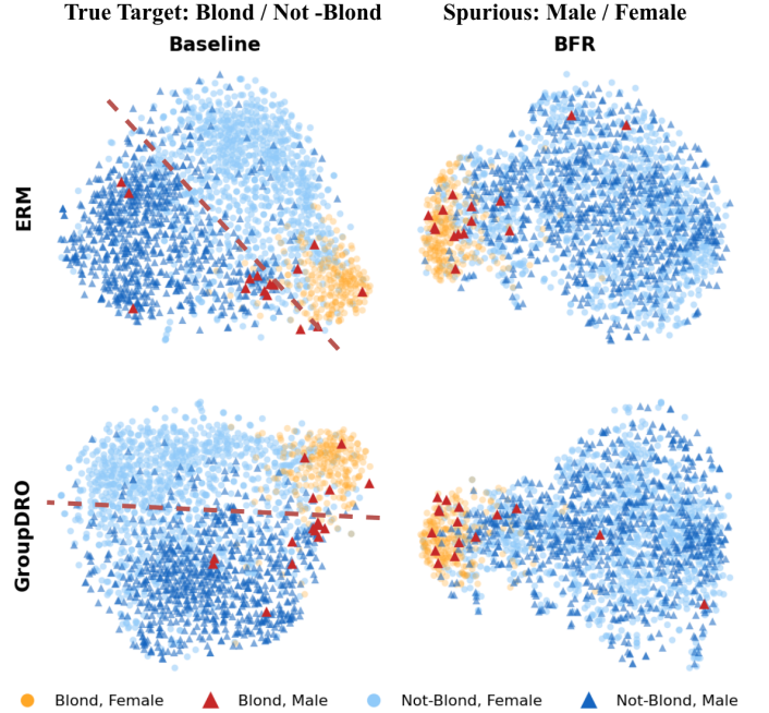
Fig. 1. t-SNE of CelebA-Std ResNet-18 features, seed 1 (Blond Hair target, Male attribute). Baseline and BFR panels illustrate different within-class subgroup layouts. BFR reduces the targeted centroid discrepancy; two-dimensional mixing does not establish concept erasure or causal feature use.
