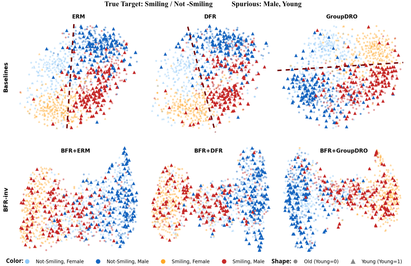
Fig. 5. t-SNE of CelebA-MB ResNet-18 features (Smiling target; Male and Young annotated attributes). Color encodes target and Male; shape encodes Young. Baseline panels show subgroup separation; BFR panels illustrate more within-class mixing. BFR averages separate class-conditional penalties for the two supplied attributes. The visualization does not establish joint distribution alignment or lack of attribute recoverability.
