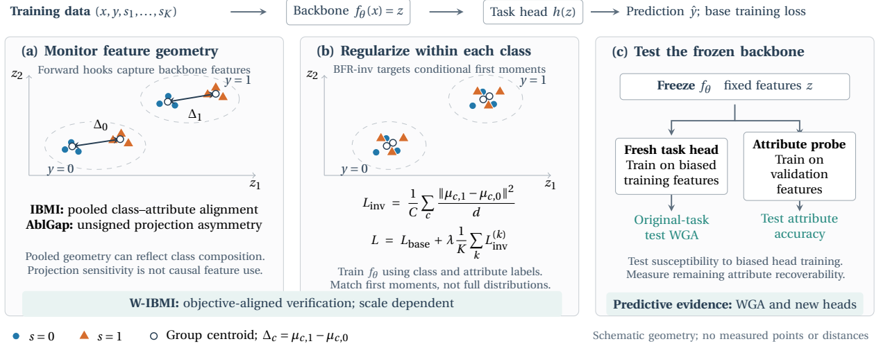
Fig. 2. BiasFlow workflow and evidence roles. (a) Forward hooks expose centroid geometry and unsigned projection sensitivity. Blue circles and orange triangles denote attribute values, dashed ellipses denote target classes, and open markers denote group centroids. (b) BFR-inv penalizes within-class centroid differences, averaged over annotated attributes during backbone training; W-IBMI is scale-dependent, objective-aligned verification. (c) Frozen-backbone tests fit a fresh task head on biased training features and a separate attribute probe on validation features, then evaluate on test features. Geometry is schematic, not measured data. Centroid alignment and projection sensitivity do not establish concept erasure or a causal intervention-selection rule; predictive evidence is limited to the tested protocols.
