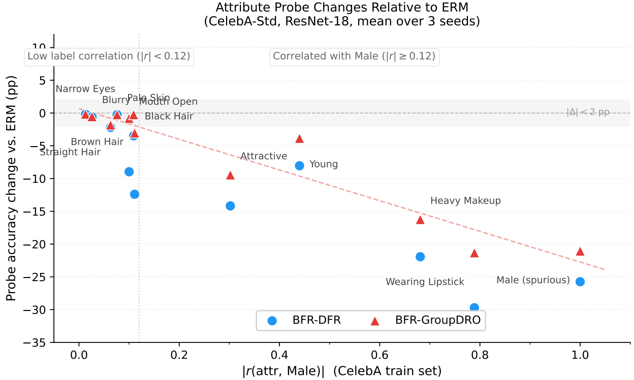
Fig. S2. Attribute-probe accuracy differences relative to ERM vs. absolute label correlation with Male, for BFR-DFR and BFR-GroupDRO. The saved plotting source uses ERM as the reference for both curves; this is not the paired BFR-minus-corresponding-base comparison in Table S5. Larger losses occur for several Male-correlated attributes, with exceptions and collateral losses at low correlation. The plot does not isolate the within-method effect of BFR or establish a distinct erased subspace.
