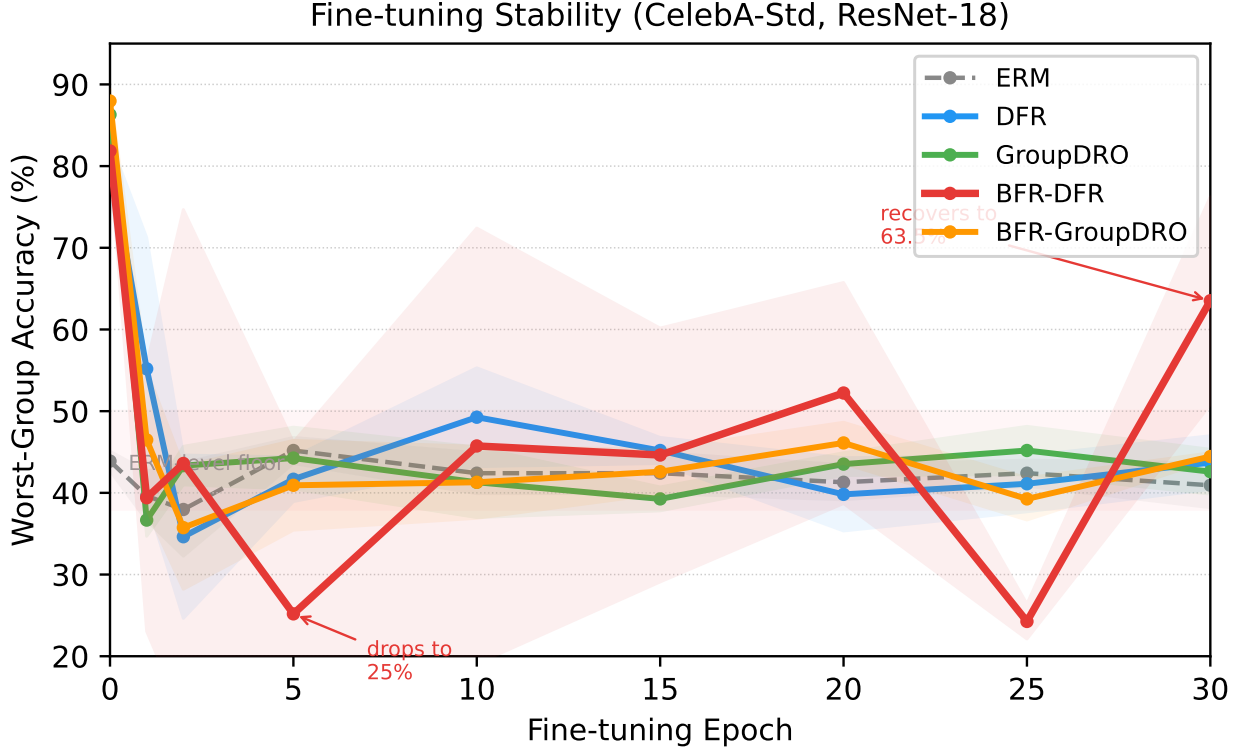
Fig. S1. WGA over 30 epochs of ERM continuation from each method’s converged checkpoint on the original CelebA-Std Blond classification task. BFR-DFR reaches 63.5% final WGA, substantially above DFR without BFR, indicating stronger retained WGA after continued training.
