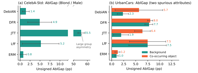
Fig. 3. Unsigned AblGap on CelebA-Std and UrbanCars, using the original plotted seed values. AblGap is |\Delta\text{Acc}_R - \Delta\text{Acc}_U| , reported in pp. Larger values indicate more asymmetric projection sensitivity across groups. The bars do not show the sign of either accuracy change, and cannot distinguish exploitation from interference.
