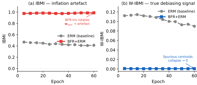
Fig. 4. Recorded IBMI and W-IBMI trajectories for ERM and BFR+ERM on CelebA-Std. Pooled centroid alignment can increase as the attribute axis becomes dominated by class composition. W-IBMI tracks the centroid penalty being optimized, rather than independent concept erasure.
