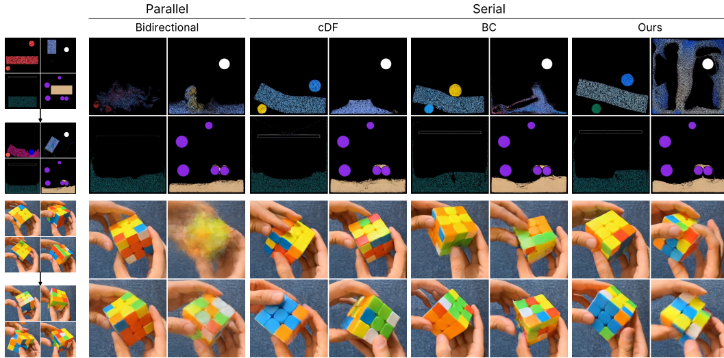
Figure 6: Qualitative comparisons with the Wan-5B-LoRA architecture. Serial methods perform similarly and produce more coherent video than the bidirectional baseline on MPMWorlds and Rubik's Cube Real datasets.
