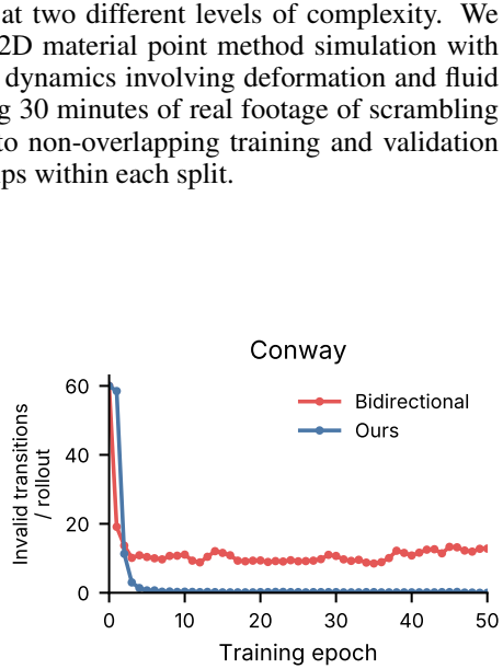
Figure 4: Learning Conway rules. Ours rapidly learns valid transitions, while the baseline continues to make errors.
