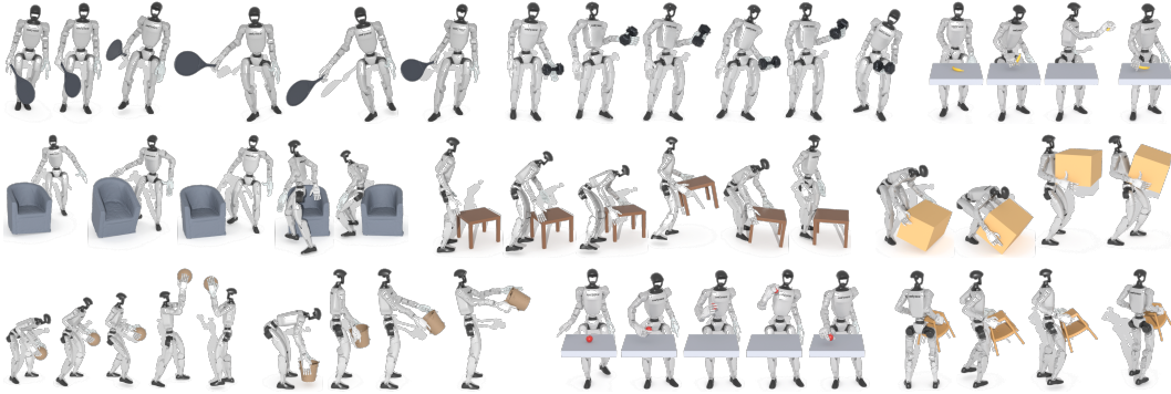
Figure 5: Physics-based tracking across objects. Executed rollouts on G1 with Inspire hands for a diverse set of objects.
