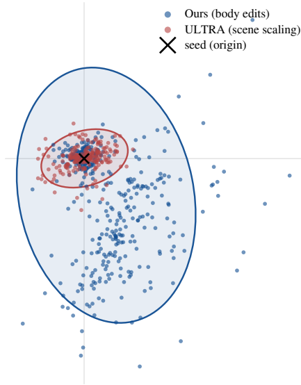
Figure 16: Body-motion variation around shared seeds. Each reference is embedded by the DCT coefficients of its body joint angles, taken relative to its seed and projected with PCA, so all seeds sit at the origin. Ellipses enclose 95% of a Gaussian fit.
