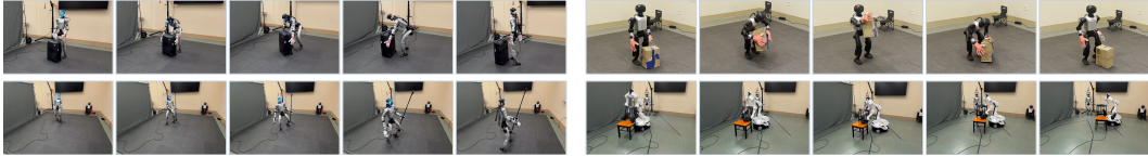
Figure 7: Real-world execution. We show the motion from our paradigm transfer to different embodiments, from Unitree G1 pulling a suitcase and G1 with Inspire hands carrying a tripod; Booster K1 lifting and placing a box and Dexmate Vega relocating a chair.
