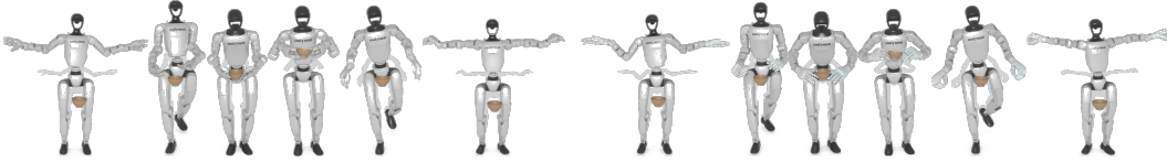
Figure 10: Retargeting with dexterous hands. A bowl-holding interaction retargeted to G1 with Dex3 (left) and Inspire (right) hands.
