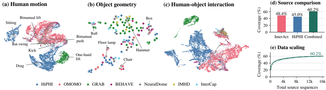
Figure 3: Our data has broad coverage. (a-c) UMAP embeddings of human motion, object geometry, and human-object interaction of our collection, colored by source dataset. (d) How well our collection covers external motions from GRAIL (Xie et al., 2026), MOVIN (Jang et al., 2023), and ELMO (Jang et al., 2024); a motion is covered when one of our sequences is close to it (Sec. E.1). (e) The same coverage as the number of our source sequences grows.
