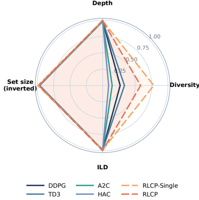
Figure 1: Performance across the 19 experimental configurations. The axes are normalized, and set size is inverted so that larger values are preferable on every axis. RLCP improves catalog diversity while maintaining competitive session depth under the same set size cap as the baselines. The full detailed results and configurations are in Appendix F.
