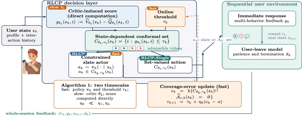
Figure 2: RLCP framework. At state s_k , critic scores g_{\theta_k}(s_k, a) and threshold \tau_k define the raw set C_{\theta_k, \tau_k}(s_k) . A minimum score fallback ensures nonempty execution. The resulting set constrains the downstream actor in RLCP or supplies the simulator in RLCP Single. Proxy miss feedback updates the threshold more frequently than the critic is updated; this schedule is an implementation choice.
