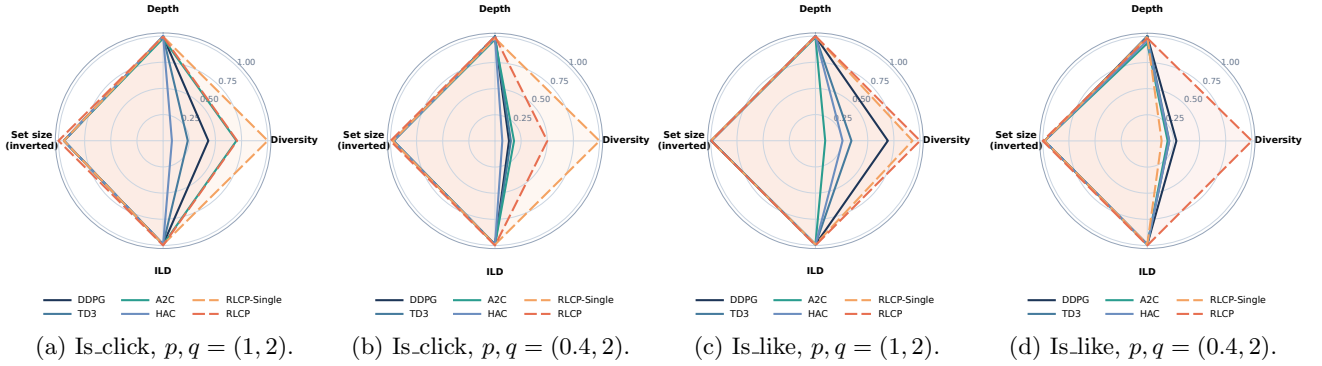
Figure 4: ML-1M radar summaries for the four reward and patience configurations reported in Tables 6–9. Each panel averages over the baseline slate sizes in the corresponding table and uses the same normalized axes as Figure 3. On the denser ML-1M data, the full RLCP is more competitive in terms of depth and catalog diversity while maintaining maximal intra-list diversity, and the RLCP variants retain their overall diversity advantage over the fixed-slate baselines.
