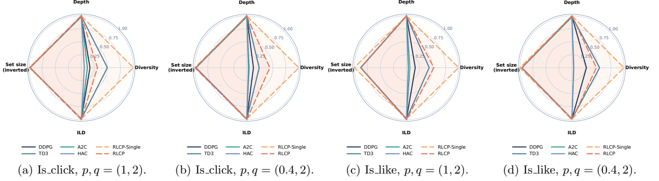
Figure 3: KuaiRand-Pure radar summaries for the four reward and patience configurations reported in Tables 2–5. Each panel averages over the baseline slate sizes in the corresponding table and shows depth, catalog diversity, intra-list diversity, and inverted set size, with larger radius indicating better performance. RLCP-Single gives the strongest catalog-diversity gains on KuaiRand-Pure while using equal or smaller admissible sets, whereas the full RLCP consistently attains the highest intra-list diversity.
