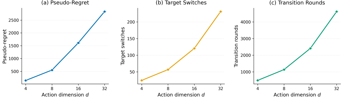
Figure 6: Scaling with the action dimension for d \in \{4, 8, 16, 32\} with a fixed reward gap of 0.2. (a) Realized pseudo-regret, (b) number of stationary-target switches, and (c) total number of transition rounds. Curves show means over 30 runs with 95% confidence intervals.
