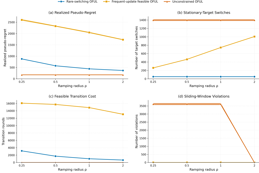
Figure 2: Rare switching under cyclic ramping constraints. (a) Pseudo-regret, (b) stationary-target switches, (c) transition rounds, and (d) constraint violations for Rare-switching OFUL, Frequent-update feasible OFUL, and Unconstrained OFUL across \rho . Curves show means over 30 runs with 95% confidence intervals.
