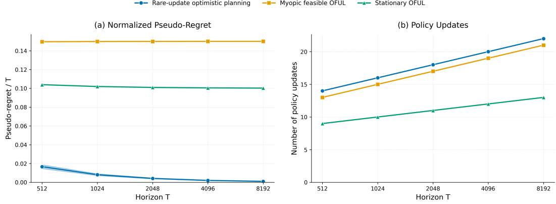
Figure 3: Planning beyond cyclic symmetry. Left: normalized pseudo-regret relative to the exact offline optimum. Right: number of policy updates. Curves show means over 30 runs with 95% confidence intervals.
