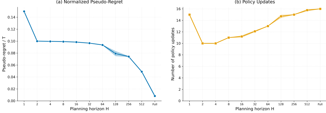
Figure 8: Sensitivity to the planning horizon H for T = 1024 . Left: normalized pseudo-regret against the offline-optimal feasible trajectory. Right: number of policy updates. The case H = 1 is myopic and “Full” denotes exact remaining-horizon planning. Curves show means over 30 runs with 95% confidence intervals.
