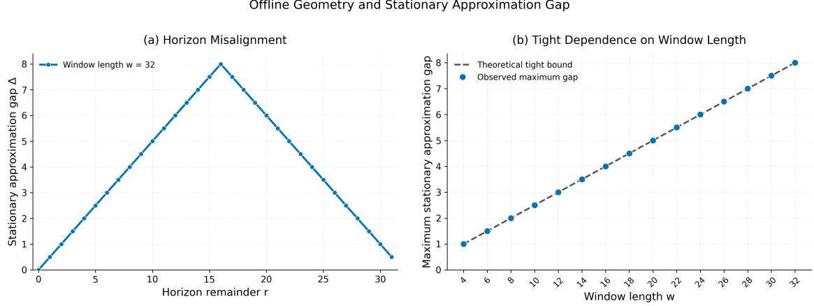
Figure 1: Offline geometry and horizon misalignment. Left: stationary approximation gap versus horizon remainder for w = 32 . Right: maximum gap versus window length; markers show the LP solutions and the dashed line shows the tight value w/4 .
