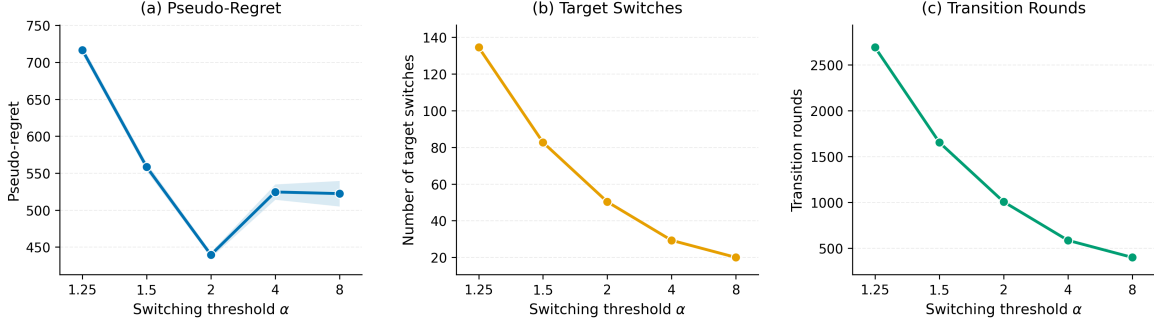
Figure 5: Sensitivity to the determinant switching threshold \alpha . (a) Realized pseudo-regret, (b) number of stationary-target switches, and (c) total number of transition rounds. The default choice \alpha = 2 achieves the lowest pseudo-regret in this experiment. Curves show means over 30 runs with 95% confidence intervals.
