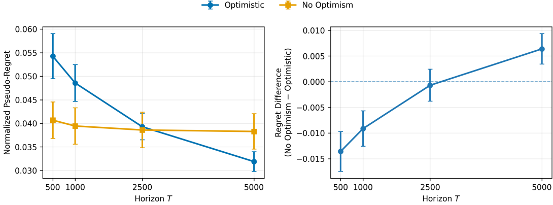
Figure 4: Ablation on optimistic exploration. Left: normalized pseudo-regret for Rare-Update Optimistic Planning and its non-optimistic variant. Right: paired regret difference, defined as \text{Regret}_{\text{NoOpt}} - \text{Regret}_{\text{Opt}} , so positive values favor optimism. Error bars denote 95% confidence intervals.
