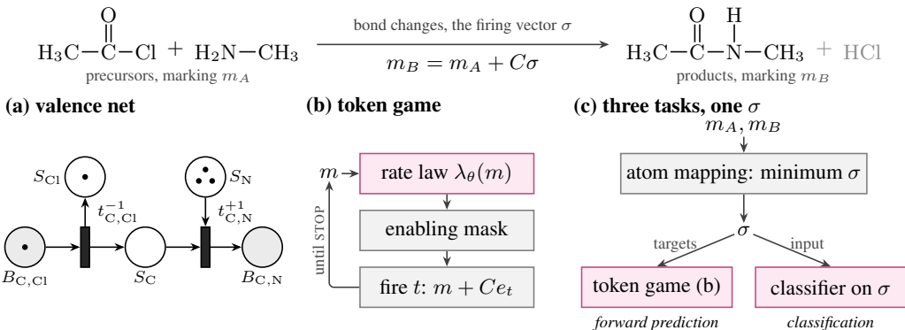
Figure 1: (a) A reaction as two markings of its valence net. (b) Only the rate law (magenta) is learned. (c) The minimum firing vector \sigma maps atoms, trains the token game and feeds the classifier.
