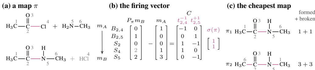
Figure 3: The firing vector. (a) A map \pi seats each product atom on the precursor atom with its number, and grey atoms leave unrecorded. (b) The state equation gives \sigma(\pi) , one firing per changed bond place, and the grey entry follows as m_A + C\sigma . The H that moves from N to Cl passes from S_5 to S_4 , while cycles in \ker C , such as the C=O of the tetrahedral intermediate, and the order of the firings stay unseen. (c) The mapper ranks maps by the bonds formed and broken, then by bond orders and charges, and returns \hat{\sigma} = \sigma(\pi_1) .
