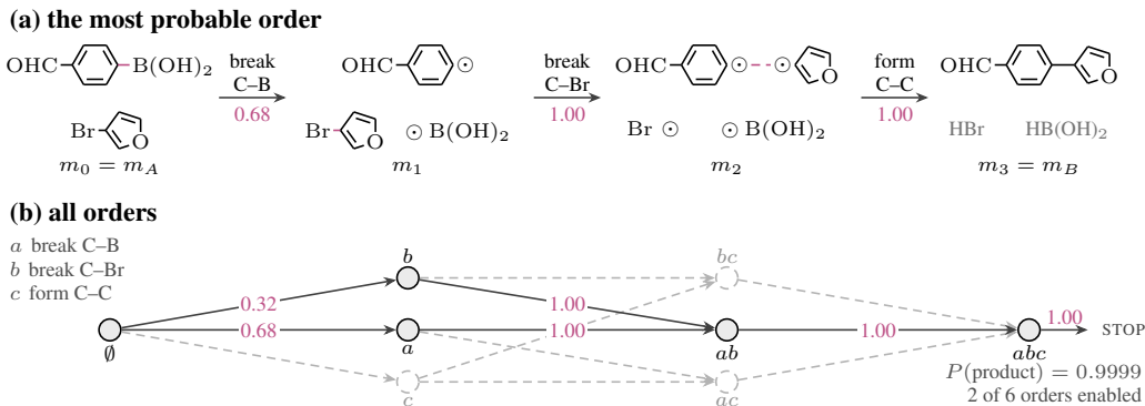
Figure 2: A bromo Suzuki-type coupling as a token game of the model trained without precomputed mappings. (a) Showing the most probable order, each bond that changes in magenta, dashed if formed. \odot is a token that a broken bond returns to the slack place of its atom. The order is valence bookkeeping, not the Pd mechanism, which would break C-Br first. (b) Forming C-C requires a token of free valence on both aryl carbons that can only be supplied by the two breaks, meaning enabling excludes the four orders that form C-C before the two bond breaks. The two remaining orders fire the same transitions and reach the same product.
