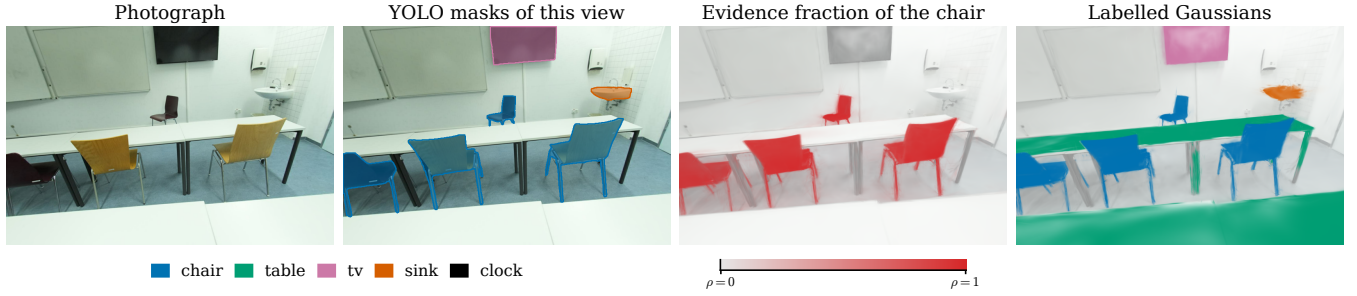
Figure 1: One view of the ScanNet++ test scene 21d970d8de. Even though YOLO does not detect the tables in this view, they are still labelled, since it detects them in other views.
