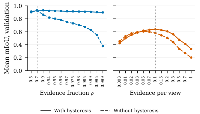
Figure 6: Mean validation mIoU along the threshold grid of each score, with the annotation masks. The dotted line is the selected threshold.
