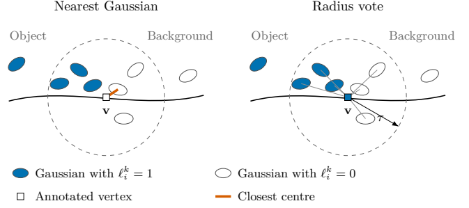
Figure 4: The two transfer operators at a vertex next to the border of an object. With \theta below 0.5, the radius vote gives the class to vertices where the nearest Gaussian does not, so the labelled region grows.
