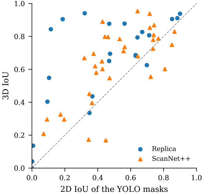
Figure 8: Pixel IoU of the YOLO masks against the 3D IoU that the method reaches from them, one marker per class and scene. Above the diagonal, the 3D result is better than the masks.
