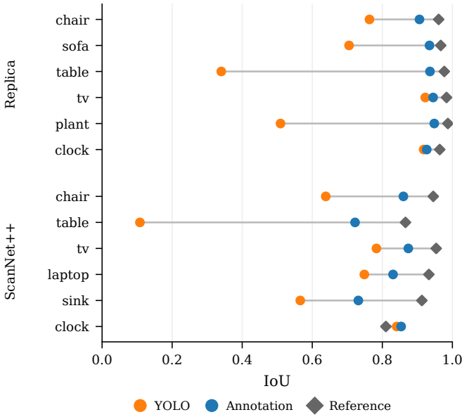
Figure 7: IoU of each class with each mask source and for the reference, averaged over the scenes that contain the class.
