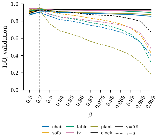
Figure 10: IoU of each class on the validation scenes along \beta , with the annotation masks, with and without hysteresis. The dotted line is \beta = 0.7 .
