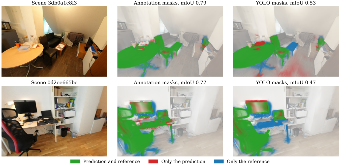
Figure 5: Prediction against reference in two ScanNet++ test scenes close to the median, over all their evaluated classes. The mIoU is the one of the whole scene, measured on the mesh.
