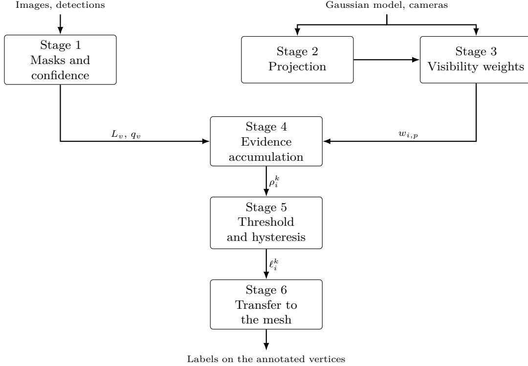
Figure 2: The six stages of the method. Stages 2 and 3 do not depend on the class, and a change of \beta or \gamma only runs the pipeline again from stage 5.
