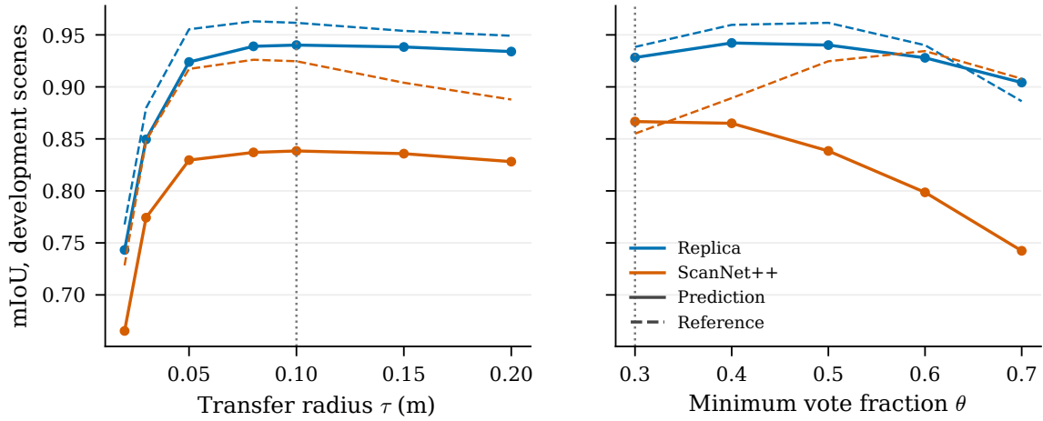
Figure 11: Development sweep of the radius vote with the annotation masks. Solid lines are the prediction and dashed lines the reference.
