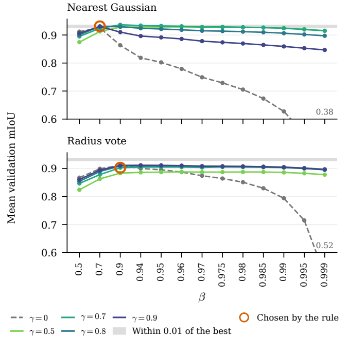
Figure 9: Mean validation mIoU along \beta for every \gamma , with the annotation masks. The grey band holds the candidates within 0.01 of the best mean.
