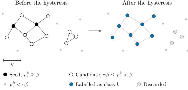
Figure 3: Hysteresis on the graph of Gaussian centres. A component takes the class only when it contains a seed.
