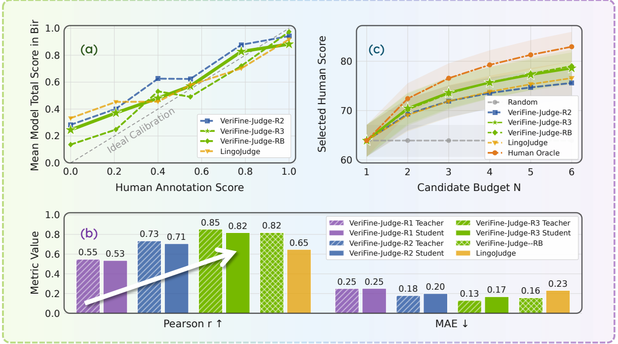
Figure 3: Judge Performance Comparison. (a) Calibration curves showing the mean judge score within each human-score bin; the gray diagonal denotes ideal calibration. (b) Judge-human alignment measured by Pearson correlation and MAE for teacher and student judges across improvement rounds and reference-based baselines. (c) Test-time scaling is evaluated by the human score of the selected candidate as the candidate budget increases. Shaded regions denote 95% bootstrap CI.
