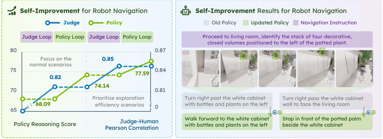
Figure 4: Self-improvement on Robot Navigation Task. The left part shows the quantitative results in the robot navigation task with significant improvement in final policy performance, and the right part shows the qualitative results with a sequential reasoning example: the updated policy with VERIFINE corrects the action failures of the old policy.
