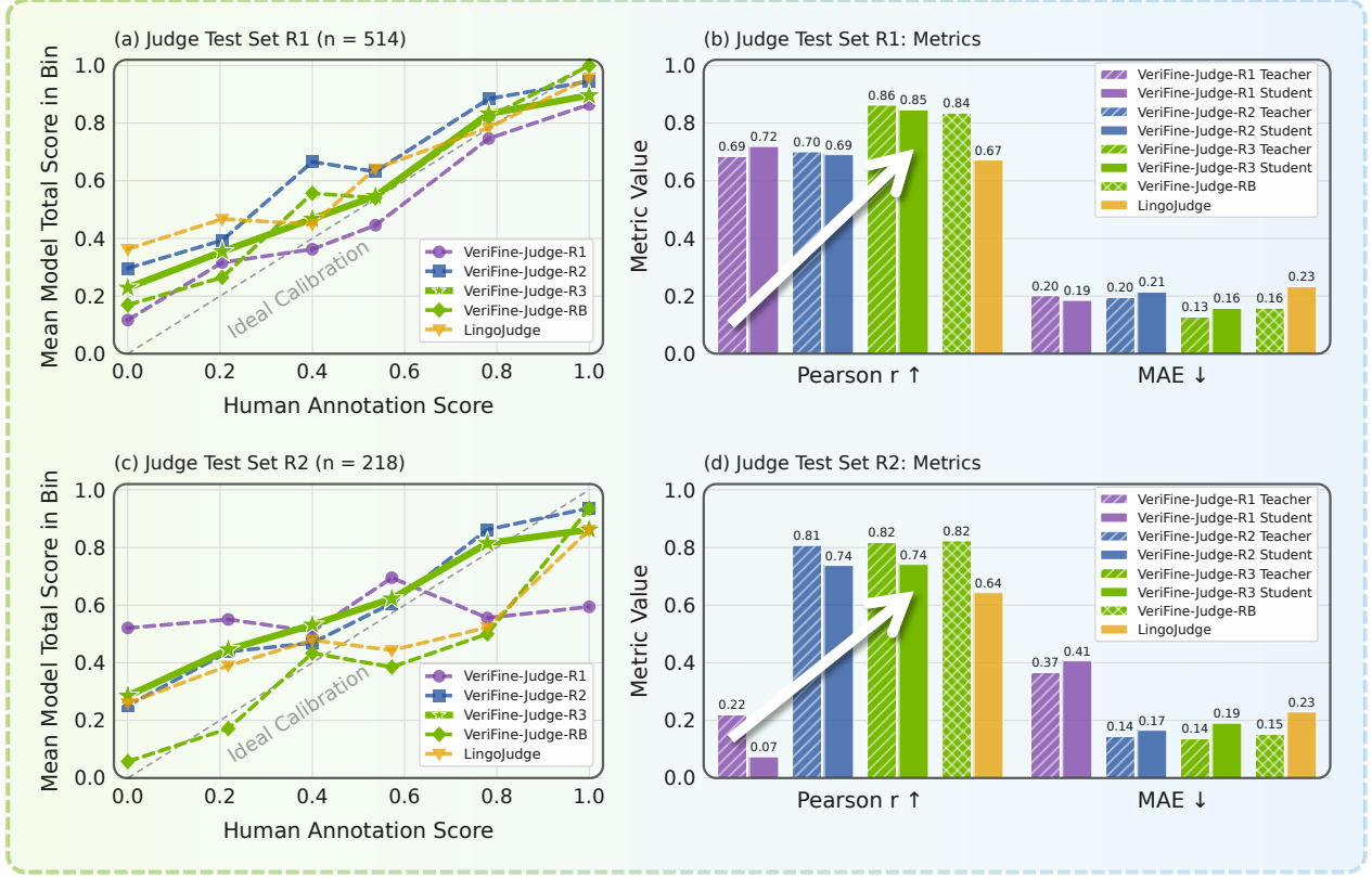
Figure 6: Evolved Judge Performance and Evolved Test Sets (R1 and R2). (a) (c) Calibration curves showing the mean judge score within each human-score bin for two evolved test subsets for the judge test set; the gray diagonal denotes ideal calibration. (b) (d) Judge-human alignment measured by Pearson correlation and MAE for teacher and student judges across improvement rounds and reference-based baselines.
