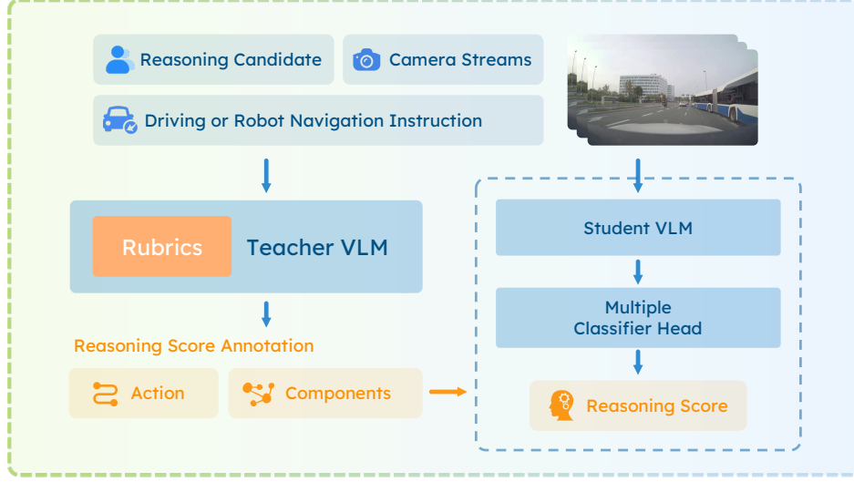
Figure 7: Teacher-Student Architecture of the Reference-free Rubric Judge. The teacher evaluates policy outputs using visual context, ego state, a driving or robot navigation instruction, and a structured rubric. Its evaluations are distilled into a compact student judge for scalable verification.
