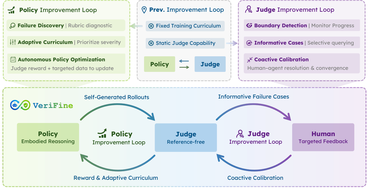
Figure 2: VERIFINE is an agent harness framework for scaling verification. The Policy Improvement Loop uses a reference-free judge to diagnose recurring failures, adapt the training curriculum, and optimize the policy. When verification limits further progress, the Judge Improvement Loop selectively acquires human guidance and refines the judge through coactive calibration, resolving disagreements in rubric-based judgments. The updated judge guides subsequent data selection and policy optimization, allowing verification capability to evolve with the policy’s failure patterns.
