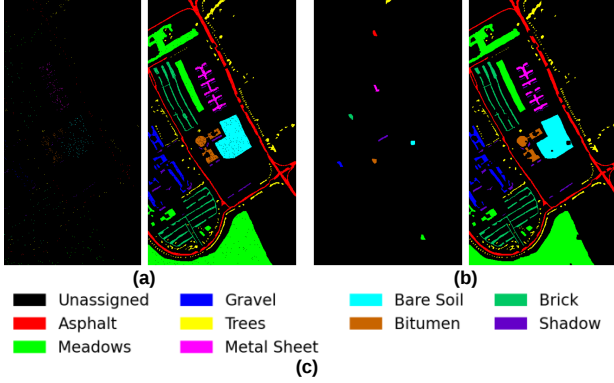
Fig. 2: Examples of the sampling settings used in this study: (a) random sampling, where training and testing patches may overlap; (b) non-random spatial sampling, where training and testing regions are selected with greater spatial separation; (c) Class Labels.
