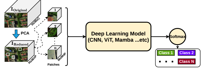
Fig. 1: General Patch-based hyperspectral image classification framework using PCA and deep learning models.
