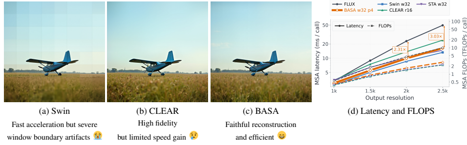
Figure 2: Motivation for BASA. Swin-style window attention (Liu et al., 2021) provides fast inference but introduces severe window boundary artifacts. CLEAR (Liu et al., 2025) preserves high visual fidelity, while its practical speed gain is relatively limited. BASA preserves faithful reconstruction while achieving efficient inference, providing a favorable quality–efficiency trade-off.
