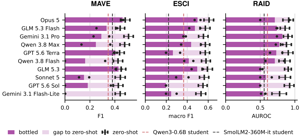
Figure 2: Good zero-shot performance does not reliably guarantee good bottling capability. We report mean bottled score against zero-shot score on each task: bottling performance usually falls well short of the zero-shot mode’s 95% CI.
