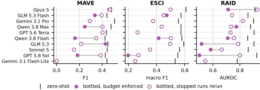
Figure 4: Letting agents exceed the budget limit does not uniformly close the zero-shot-bottling gap. We report shifts in per-task performance after re-running budget-terminated bottling runs.
