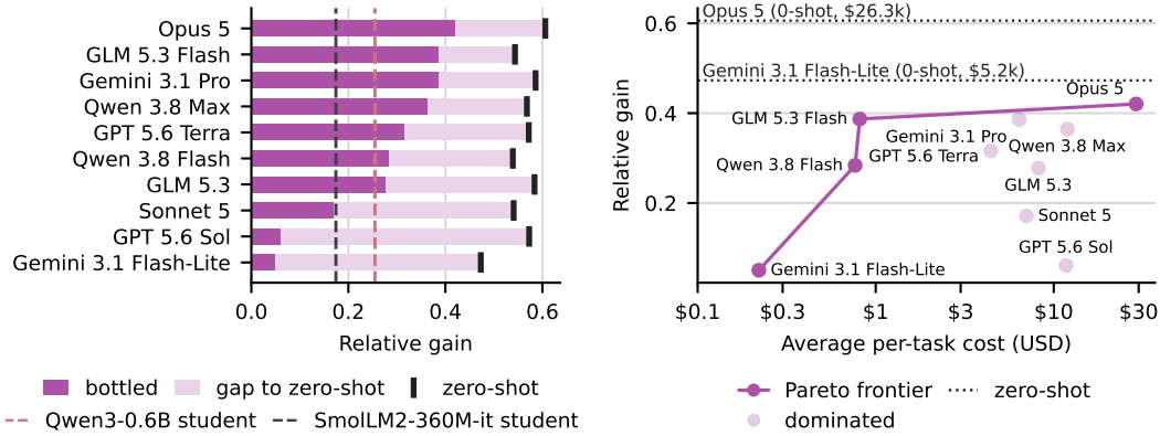
Figure 1: Bottling performance separates models with similar zero-shot capabilities; more expensive models do not necessarily bottle better. We show aggregated relative gains for each model, averaged over the three tasks and two runs. Left: each model’s bottled score against its zero-shot score. Right: Pareto frontier.
