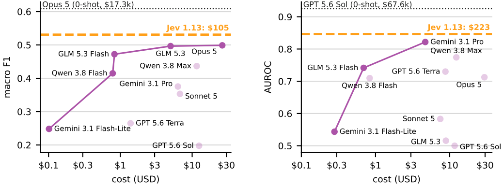
Figure 3: Bottling competes with Jev on ESCI and RAID. We plot each model’s mean bottling performance vs cost on the full workload, alongside Jev’s 1000-sample performance estimates and projected full-workload costs.
