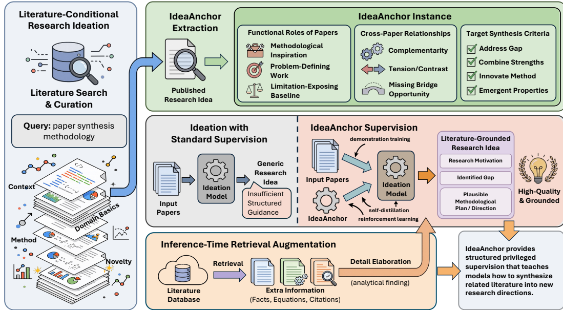
Figure 1: Overview of IdeaAnchor. Starting from a set of papers, we extract IdeaAnchor instances from published papers by identifying the functional roles of prior work, their cross-paper relationships, and the target synthesis criteria. These structured anchors make otherwise implicit synthesis logic explicit, providing privileged supervision for demonstration learning, self-distillation, and reinforcement learning. At inference time, the framework uses either related papers or a topic query as input. It can also incorporate retrieval augmentation, which complements the learned synthesis capability by supplying factual and methodological details for elaborating generated research ideas.
