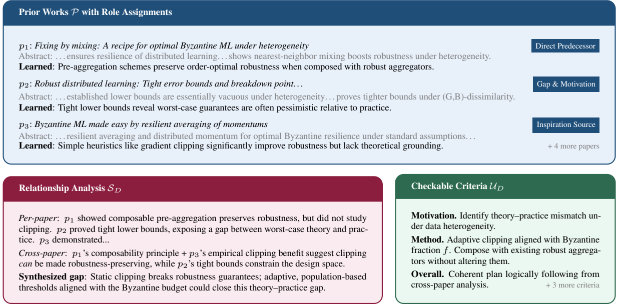
Figure 2: A sample IdeaAnchor instance derived from a paper on Byzantine-resilient distributed learning. The anchor encodes per-paper role assignments with learned insights ( top ), a cross-paper relationship analysis identifying the synthesized gap ( bottom-left ), and literature-grounded checkable criteria ( bottom-right ).
