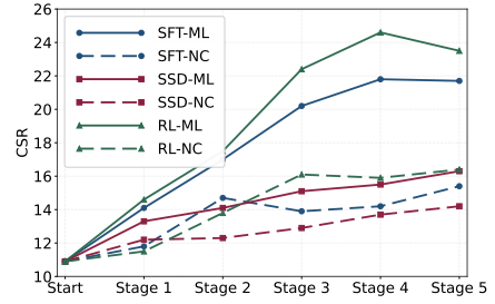
Figure 5: Training dynamics of anchor-driven ideation. CSR is measured on the ICLR benchmark across training stages for SFT, Self-Distillation, and RL over Qwen3-8B. Solid curves use machine-learning anchors, while dashed curves use only natural-science anchors and are evaluated on the same benchmark.
