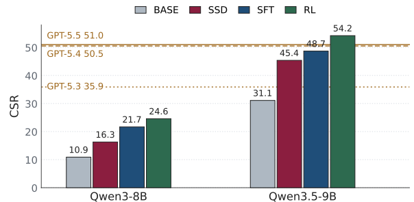
Figure 3: Main automated evaluation on the ICLR 2026 benchmark with 924 instances. Bars report CSR (%) for the base, self-distillation (SSD), SFT, and RL variants of Qwen3-8B and Qwen3.5-9B. Horizontal lines show proprietary model references.
