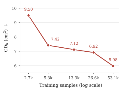
Figure S4: Dataset scaling analysis for bridge matching model training.
