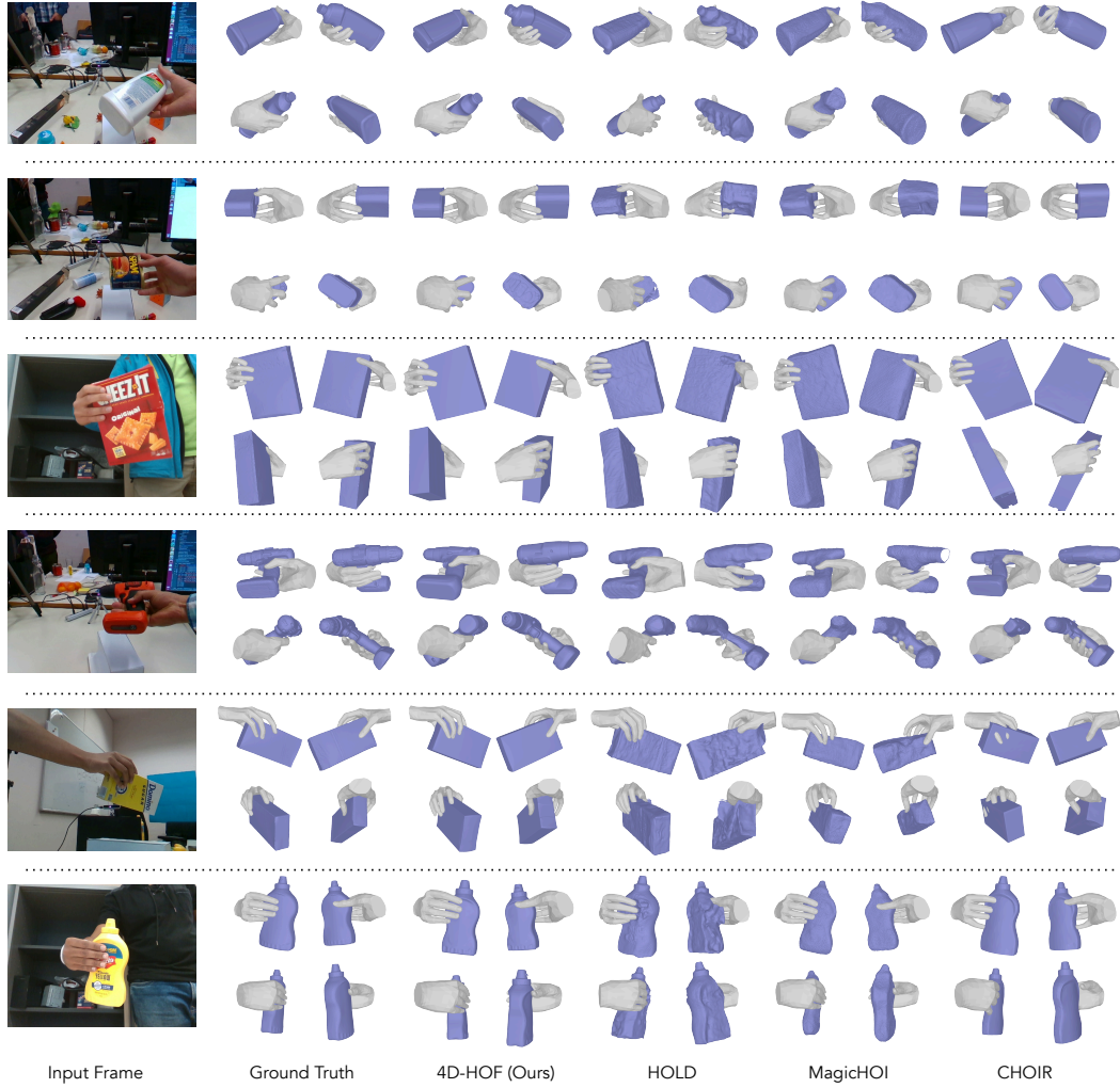
Figure S2: Qualitative results on HO3D-v3 (Hampali et al., 2020) following MagicHOI’s setting.
