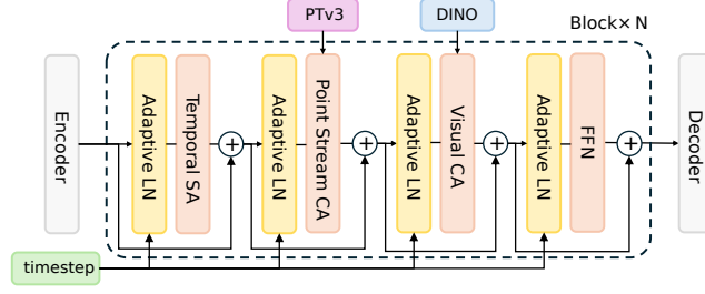
Figure S1: Model architecture. Our model adopts a DiT-style architecture for conditional flow matching. The latent hand-object state is processed through temporal self-attention, point-stream cross-attention using Point Transformer V3 features, and visual cross-attention using DINO features. Adaptive layer normalization conditioned on the timestep is applied throughout the network to modulate the generative transport process.
