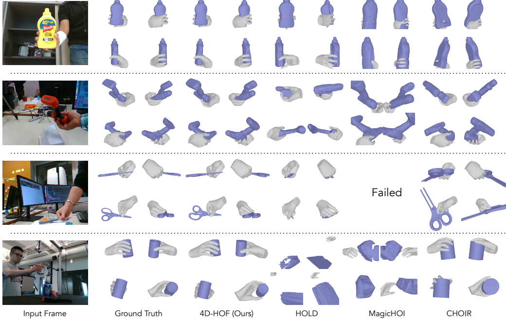
Figure 3: Qualitative results on HO3D-v3 (Hampali et al., 2020) and DexYCB (Chao et al., 2021). 4D-HOF consistently outperforms HOLD (Fan et al., 2024) and MagicHOI (Wang et al., 2025b) in preserving accurate geometry and hand-object interactions. Please see our supplementary video for detailed comparisons.
