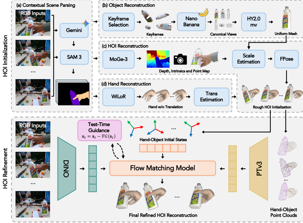
Figure 2: 4D-HOF overview. Given a monocular video, we construct initial hand-object states by leveraging foundation models, including (a) contextual scene parsing, (b) object reconstruction, (d) hand reconstruction, and (c) depth alignment for recovering metric geometry, producing coarse HOI initialization. We then formulate HOI refinement as a conditional generative bridge matching problem that takes the HOI initialization together with RGB and 3D cues as input and outputs the refined HOI reconstruction. At inference time, test-time guidance adjusts the evolving states to better satisfy physical and image-space constraints.
