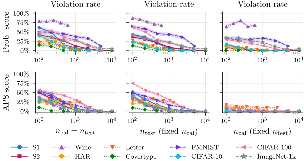
Figure 8: We show the violation rate as we vary n_{\text{cal}} and n_{\text{test}} jointly (left) or independently (middle and right). All panels report the mean \pm standard error based on 100 random draws of the calibration and test sets from the fixed evaluation pool.
