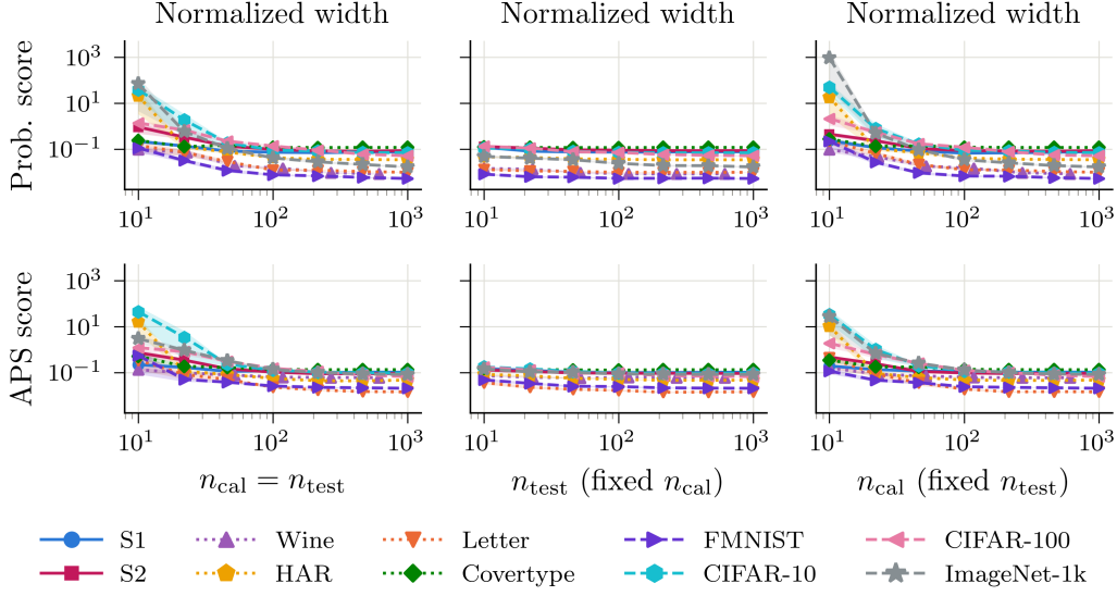
Figure 9: We show the normalized width as we vary n_{\text{cal}} and n_{\text{test}} jointly (left) or independently (middle and right). All panels report the mean \pm standard error based on 100 random draws of the calibration and test sets from the fixed evaluation pool.
