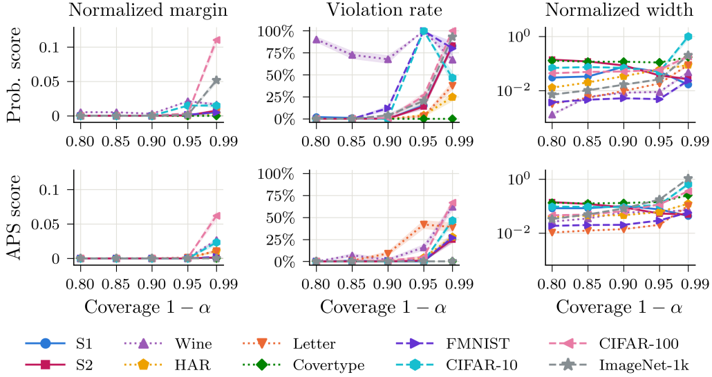
Figure 10: We show the normalized margin, violation rate, and normalized width as we vary the nominal coverage level 1 - \alpha \in \{0.8, 0.85, 0.9, 0.95, 0.99\} , with n_{\text{cal}} and n_{\text{test}} fixed at their largest values for each dataset. All panels report the mean \pm standard error based on 100 random draws of the calibration and test sets from the fixed evaluation pool.
