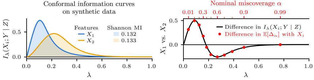
Figure 2: Conformal mutual information accurately reflects feature utility for reducing set size, whereas Shannon mutual information may not. We show information profiles \lambda \mapsto I_\lambda(X_i; Y | Z) for two candidate features X_1 and X_2 with similar Shannon mutual information (left), along with their differences in I_\lambda and \mathbb{E}[\Delta_\alpha] using the probability score (right). Nominal miscoverage levels \alpha \in \{0.01, 0.1, \dots, 0.9, 0.99\} are indicated along the top axis. Despite having nearly identical Shannon mutual information, X_1 yields a larger conformal set-size reduction at high coverage ( 1 - \alpha > 0.6 ), whereas X_2 reduces set size more at low coverage levels. Each difference in \mathbb{E}[\Delta_\alpha] is positioned at the geometric mean of the two calibrated thresholds.
