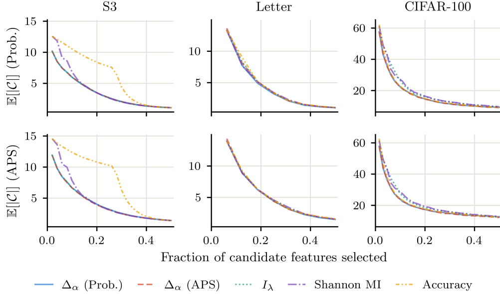
Figure 12: We show the expected set size using the probability score and APS score against the fraction of candidate features selected. Each curve is the mean over 10 random splits of the evaluation pool. We show only the first half of the selection trajectory, after which the curves largely coincide. On S3 and CIFAR-100, the gap between \Delta_\alpha and Shannon MI is concentrated in the early steps, which becomes diluted when averaging over the full trajectory.
