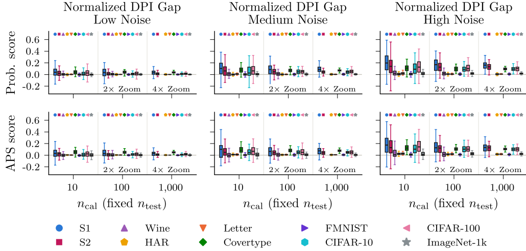
Figure 11: We show the normalized DPI gap across calibration sample sizes and degradation levels, using boxplots to summarize 100 random draws of the calibration and test sets. Each column corresponds to a degradation level, and the marker for each dataset is indicated above the corresponding boxplots. For visual clarity, we magnify the y -axis by 2\times and 4\times for n_{\text{cal}} = 100 and n_{\text{cal}} = 1,000 , respectively. Datasets whose evaluation pool is too small for a given calibration size are omitted.
