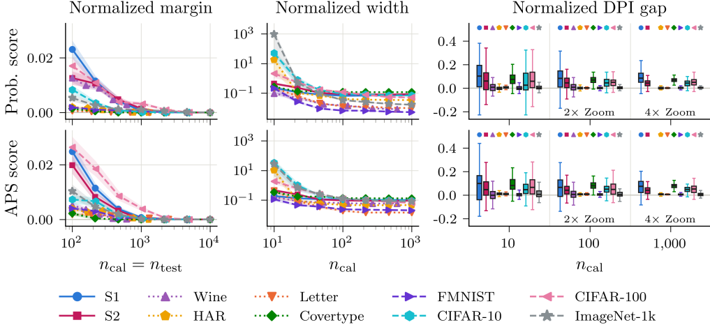
Figure 3: We show the normalized margin, width, and DPI gap based on 100 random draws of the calibration and test sets from the fixed evaluation pool. The margin and width panels report the mean \pm standard error, while the DPI gap panel summarizes the distribution using boxplots. Datasets whose evaluation pool is too small for a given calibration size are omitted.
