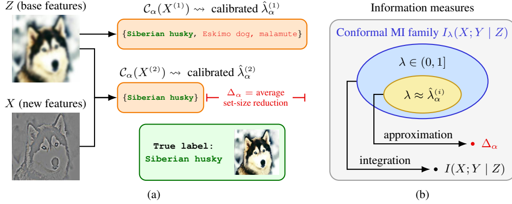
Figure 1: We illustrate an example of our setting in (1a), where Z is a low-resolution image and X is its residual. The information gain of X beyond Z can be quantified by \Delta_\alpha . We develop the information hierarchy in (1b), showing that conformal mutual information near the calibrated \lambda approximates \Delta_\alpha , while Shannon mutual information aggregates the entire family (Theorem 1).
