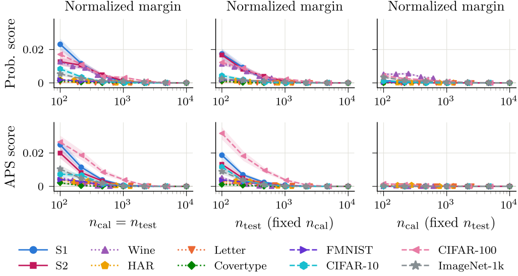
Figure 7: We show the normalized margin as we vary n_{\text{cal}} and n_{\text{test}} jointly (left) or independently (middle and right). All panels report the mean \pm standard error based on 100 random draws of the calibration and test sets from the fixed evaluation pool.
