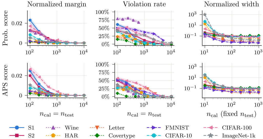
Figure 6: We show the normalized margin and violation rate as we jointly vary n_{\text{cal}} and n_{\text{test}} (left and middle) and the normalized width as we vary n_{\text{cal}} while keeping n_{\text{test}} fixed (right). All panels report the mean \pm standard error based on 100 random draws of the calibration and test sets from the fixed evaluation pool.
