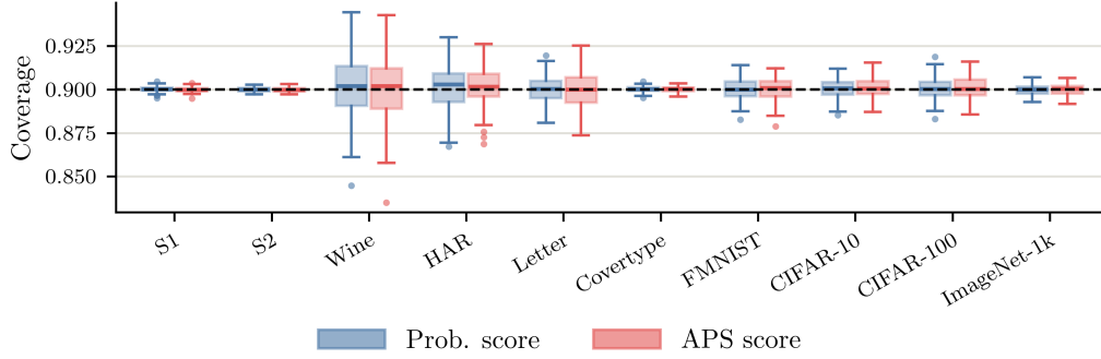
Figure 5: Empirical marginal coverage of the conformal predictors using (X, Z) over 100 random equal calibration and test splits of the evaluation pool. The dashed line indicates the nominal coverage level 1 - \alpha = 0.9 .
