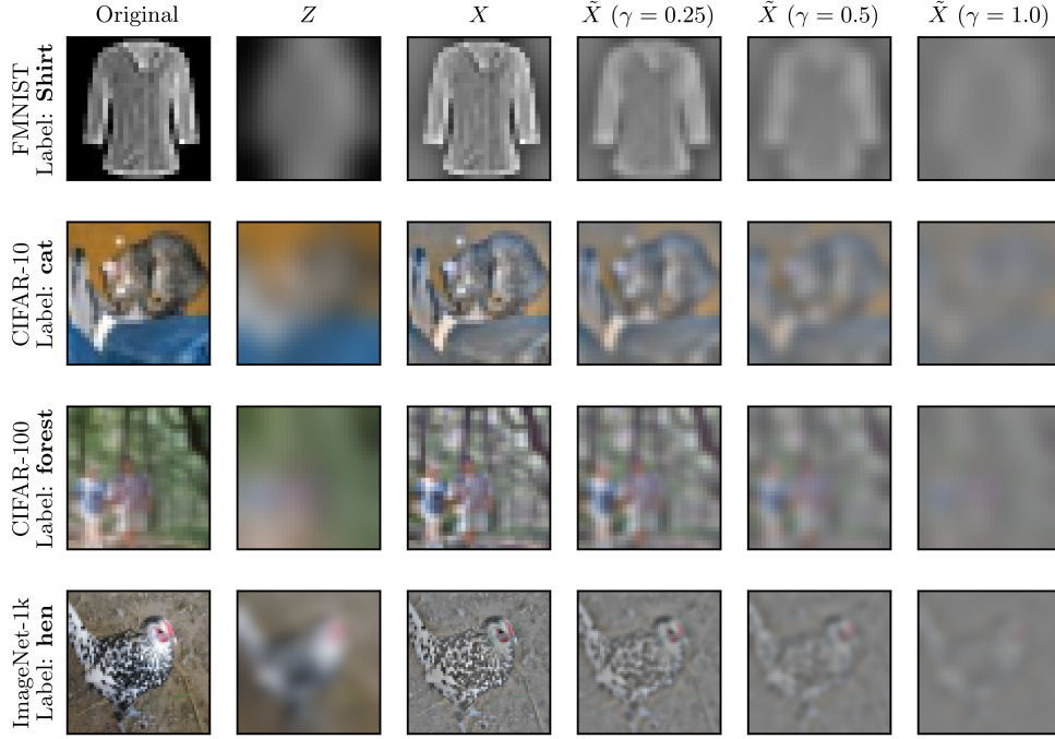
Figure 4: Examples of the original image, base, new, and degraded features for each image dataset. The degraded features apply an additional Gaussian blur with standard deviation \gamma\sigma to X .
