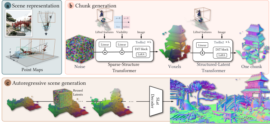
Fig. 2. Overview of our method. (a) Scene representation. We lift the input image using an estimated point map and partition the scene into adaptive 3D chunks. (b) Chunk generation. For each chunk, the generator first predicts the sparse structure and then its structured geometry latents. Both stages are conditioned on surface-aligned lifted image features, while the first stage further receives a depth-based visibility indicator to distinguish free space vs. occluded regions. (c) Autoregressive scene generation. We generate neighboring chunks sequentially while reusing latents in overlapping regions, allowing each new chunk to complete unseen geometry conditioned on the previously generated scene chunk. The assembled latents are finally decoded into the full scene mesh.
