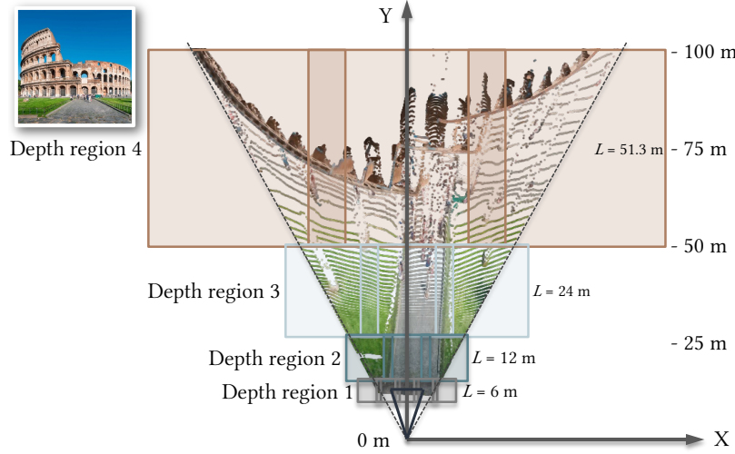
Fig. A1. Chunk allocation. We partition this Colosseum into overlapping depth regions and allocate chunks to cover the estimated point cloud within the camera frustum.
