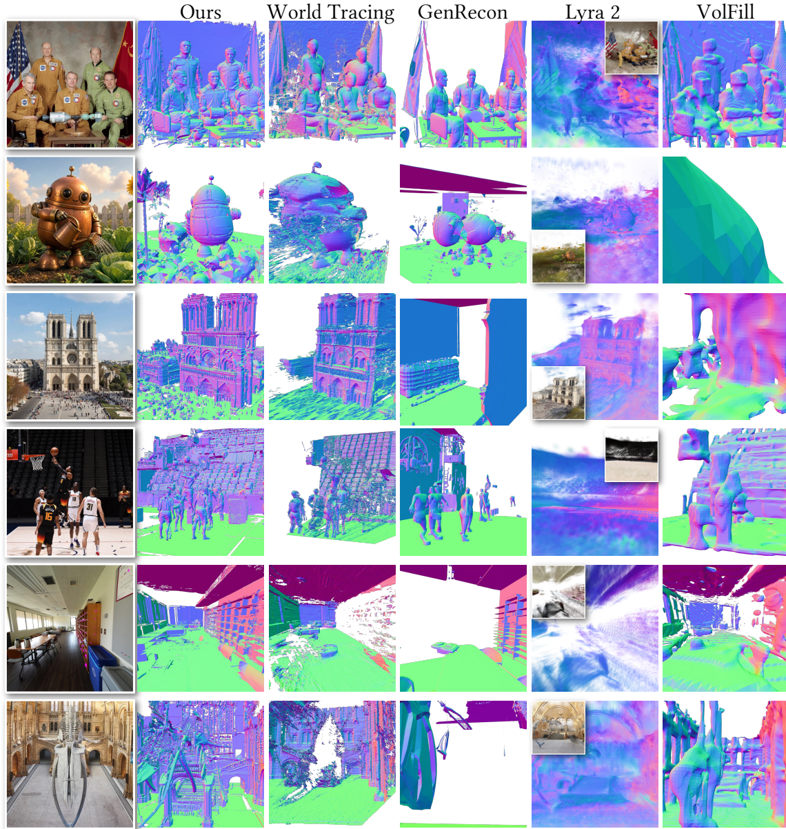
Fig. A4. Additional qualitative comparisons on diverse scenes. We evaluate scenes containing people, animals, large architectural structures, and unusual object configurations. Our method more consistently recovers coherent geometry and scene structure, while the baselines often exhibit incomplete geometry, simplified layouts, or coarse surfaces.
