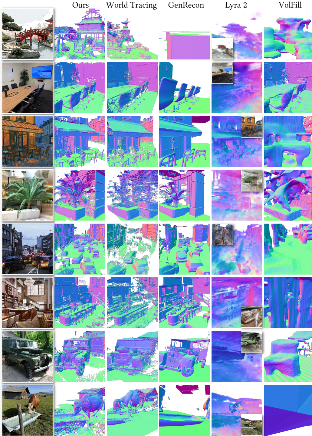
Fig. A3. Additional qualitative comparisons on diverse scenes. We compare surface-normal renderings across indoor and outdoor environments. Our method better preserves scene layout and local geometry, and occluded regions. For Lyra 2, we overlay its RGB rendering on the normal map.
