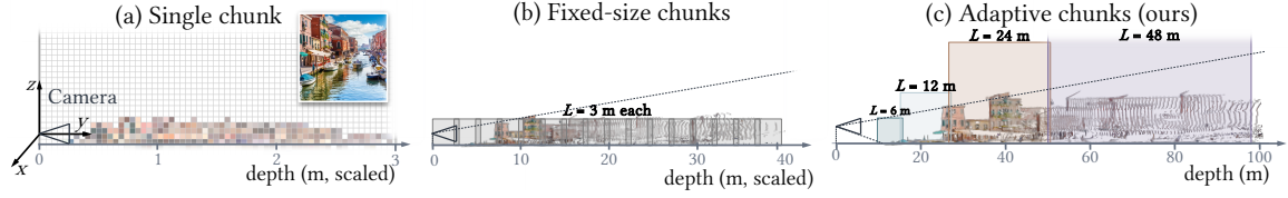
Fig. 3. Scene chunking strategies. A single chunk (a) compresses the entire scene into one fixed volume, sacrificing geometric detail, while fixed-size chunks (b) require many chunks to cover large scenes. Our adaptive strategy (c) increases the physical chunk size with depth, preserving finer resolution nearby while efficiently covering distant regions. Best viewed zoomed in.
