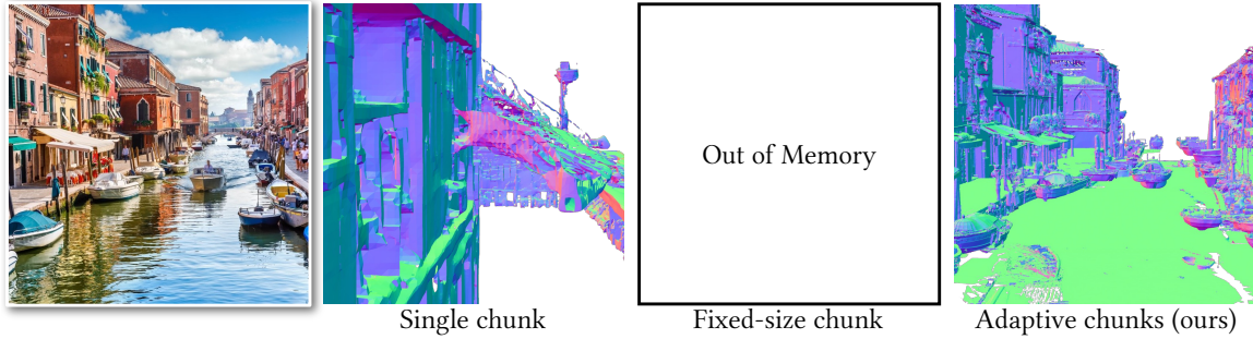
Fig. A2. Comparison of chunking strategies. A single chunk compresses the entire scene into a fixed canonical volume, distorting depth and producing wall-like geometry. Fixed-size chunks require too many chunks for large scenes, and it ran out of memory on an 80G GPU. Our adaptive strategy efficiently covers the scene while preserving geometric detail.
