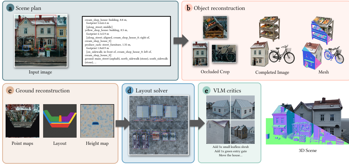
Fig. A5. Agentic framework for outdoor scene construction. Given an input image, (a) a VLM first produces a scene plan describing objects, their dimensions and spatial relations, and ground regions. (b) Each visible object is cropped from the image, completed to recover occluded geometry, and reconstructed into a 3D mesh. (c) Ground geometry is recovered from the estimated point map, semantic layout, and height map. (d) A layout solver places the reconstructed assets while satisfying spatial constraints and avoiding collisions. (e) A VLM critic iteratively inspects the assembled scene and proposes corrections to object placement and missing content, producing the final 3D scene.
