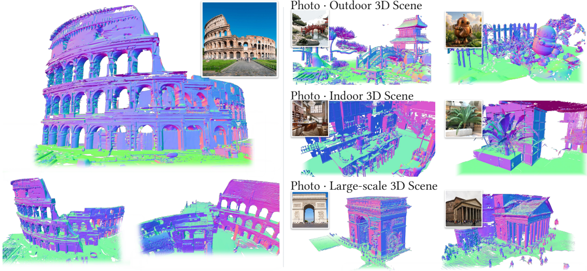
Fig. 1. Generating a complete 3D mesh from a single image. Our method reconstructs detailed scene meshes from one photograph. The method completes geometry beyond the observed view and supports indoor, outdoor, and large-scale scenes. We show the Colosseum reconstruction from multiple viewpoints (left) and diverse reconstruction results (right).
