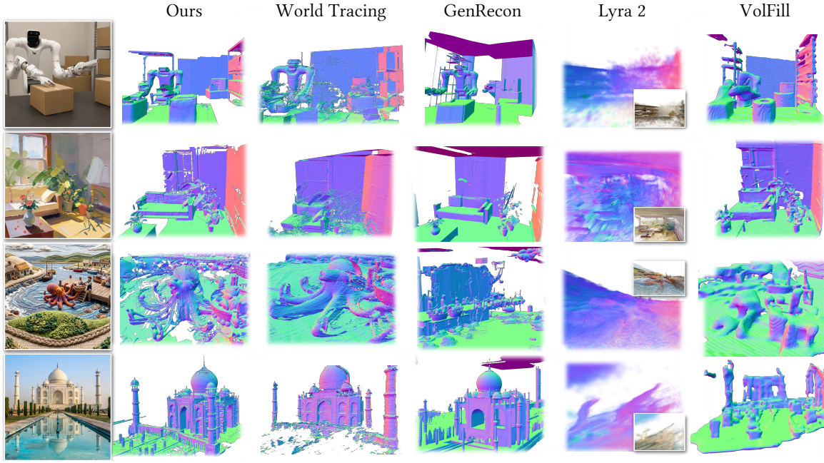
Fig. 5. Visual comparisons. Our method preserves global scene layout while recovering finer details across diverse inputs. World Tracing [48] produces noisy occluded regions and lacks detail. GenRecon [36] often imposes a room-like prior for outdoor scenes. For Lyra 2 [37], we overlay RGB on the normal map. Although the rendering appears plausible, the underlying geometry is inaccurate. VolFill [27] has line-like surface artifacts and fails on outdoor scenes.
