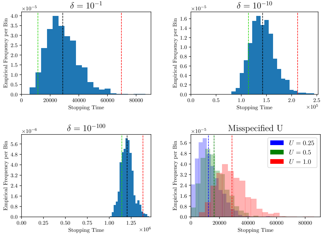
Figure 1: Histograms of stopping times in 1000 runs. The first three figures use U = 1 and vary \delta , the dashed lines are (green) the expected stopping time as predicted by Theorem 4, (black) the empirical average stopping time, and (red) the stopping time as predicted by Lemma 3 (as also spelled out in Table 1). The last figure fixes \delta = 1/10 and mis-specifies U = 1, \frac{1}{2}, \frac{1}{4} . Here the dashes show the average stopping times. U = \frac{1}{4} admits 4 mistakes, all other runs were perfect.
