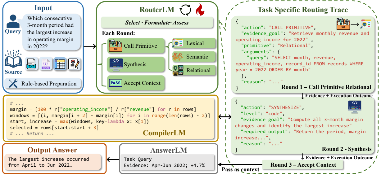
Figure 1 | Overview of RECAST. At each round, RouterLM uses the task, compact source profile, and evidence and feedback from earlier rounds to either select and formulate a primitive or synthesized operation or pass the evidence to AnswerLM when it considers the evidence sufficient.
