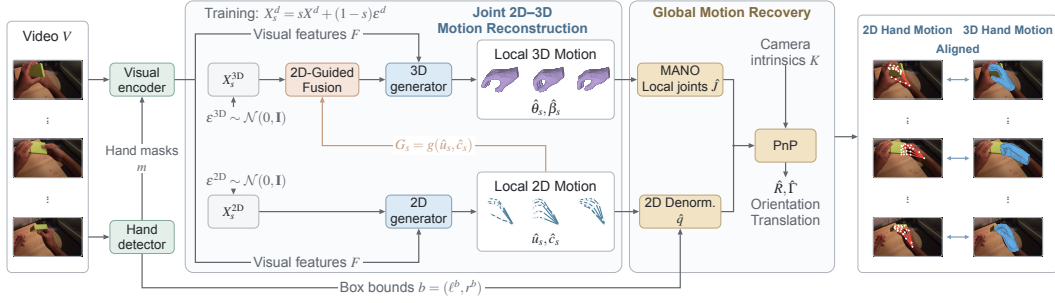
Figure 2: Overview of JoHan. We first combine full-frame video features with encoded detector-derived hand masks m to form visual conditions F . Within the Joint 2D–3D Motion Reconstruction module, the 2D generator predicts clean local motion \hat{X}_s^{2D} from the noisy state X_s^{2D} at each flow step. This prediction is then encoded as guidance G_s for the 3D generator, allowing the predicted 2D geometry to inform 3D motion generation. After that, detector-derived bounds restore the image-plane location and scale of the generated 2D local poses. A PnP solver then uses these restored poses, the corresponding local MANO joints, and camera intrinsics K to recover global orientation \hat{R} and translation \hat{\Gamma} , which are used to place the reconstructed hands in the camera coordinate system.
