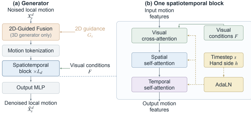
Figure 6: Conditioned generator architecture. (a) Each generator maps noised local motion X_s^d to a clean-motion prediction \hat{X}_s^d . Only the 3D generator uses 2D-Guided Fusion, which incorporates the guidance G_s from the current 2D prediction before motion tokenization. (b) Each spatiotemporal block applies visual cross-attention conditioned on F , followed by spatial and temporal self-attention. Gold dashed arrows indicate AdaLN-Zero conditioning from timestep s and hand side h in both generators.
