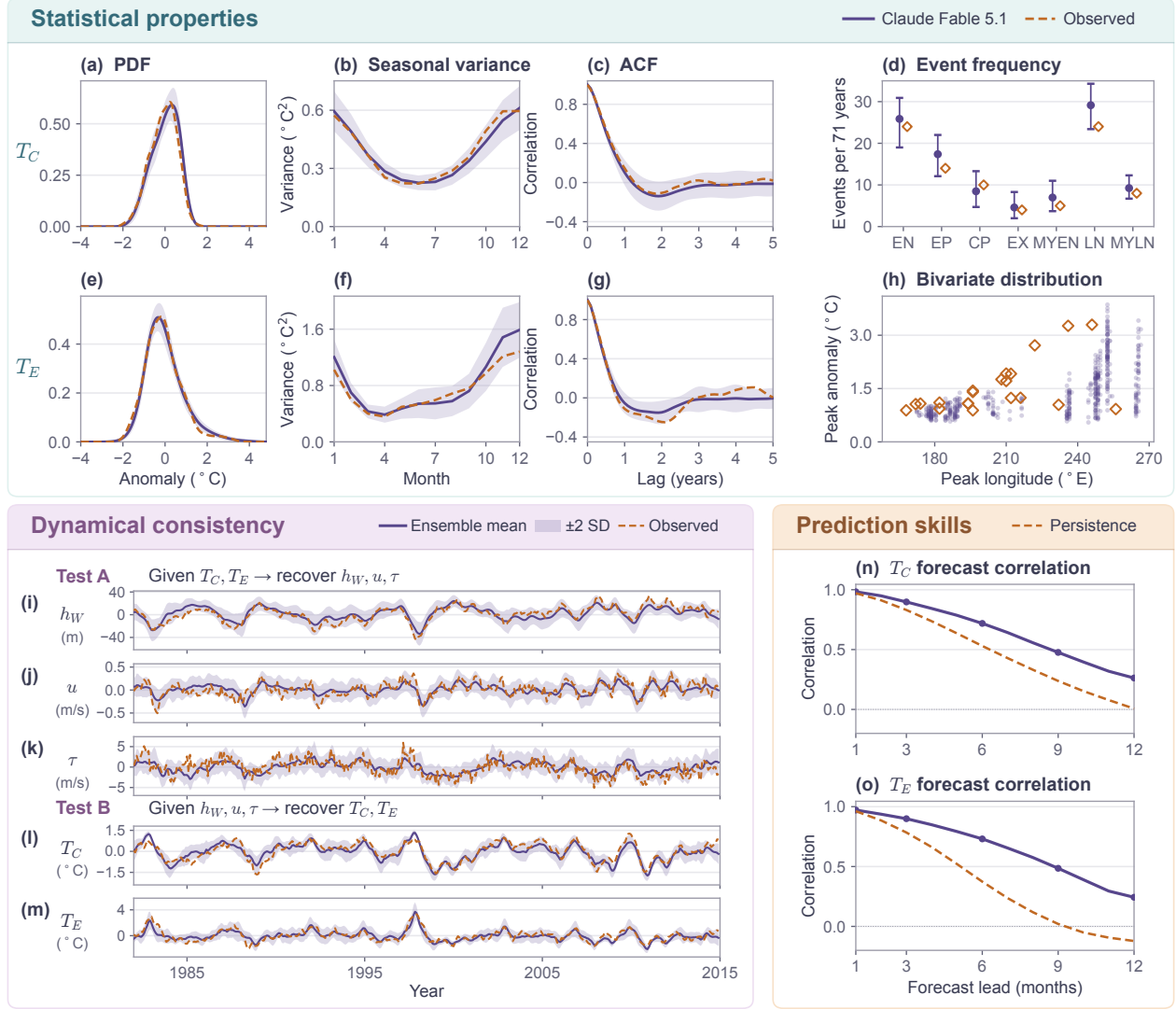
Figure 4: Scientific diagnostics of the final ENSO model produced by Claude Fable 5.1. Panels (a–c, e–g): Simulated and observed probability density functions (PDFs), seasonal variance, and autocorrelation functions (ACFs) for T_C and T_E . Panel (d): Event counts per seventy-one years, with model means and 2.5th–97.5th percentile ranges compared against observed counts. EN and LN denote El Niño and La Niña. EP and CP denote eastern- and central-Pacific El Niño, and EX denotes extreme El Niño. MYEN and MYLN denote multi-year events. Panel (h): Peak temperature anomalies versus peak longitudes for simulated and observed events. Panels (i–m): State reconstruction from partial measurements. Test A uses T_C and T_E to reconstruct h_W , u , and \tau . Test B swaps the observed and reconstructed variables. Panels (n, o): Correlations between ensemble-mean forecasts and observations at lead times of one to twelve months over the held-out 2015–2024 period, compared with persistence.
