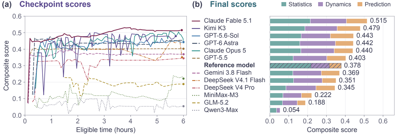
Figure 3: Model development and final scores. Panel (a): Composite scores of the checkpoints of each system against eligible time from the start of the run, including data processing and diagnostic development. Filled circles mark final checkpoints, and colors and line styles follow the system names in panel (b). Panel (b): Final scores of the twelve systems and the reference model, ranked by composite score. Stacked segments show the weighted contributions of statistical properties, dynamical consistency, and predictive skill, with weights of 0.3, 0.3, and 0.4, and numbers at the ends give the composite scores.
