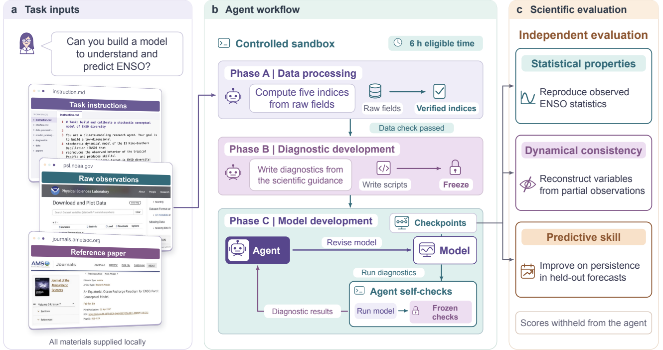
Figure 2: Overview of SciEXAM FOR ENSO. Given background material, raw observations, and a reference paper, the agent works through three phases within a six-hour budget: (A) processing the observations into indices that must pass a data check, (B) writing its own diagnostics from the task’s scientific guidance, which are then frozen, and (C) developing the model while rerunning these diagnostics. Hidden graders evaluate the final model on statistical properties, dynamical consistency, and predictive skill without returning scores to the agent. Dialogue is illustrative.
